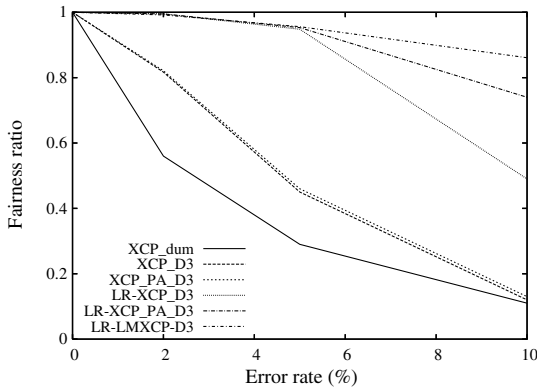
Fig. 3. Fairness ratio measured between lossy and loss-free flows as a function of the loss rate. \text{dupackthreshold} = 3 .
