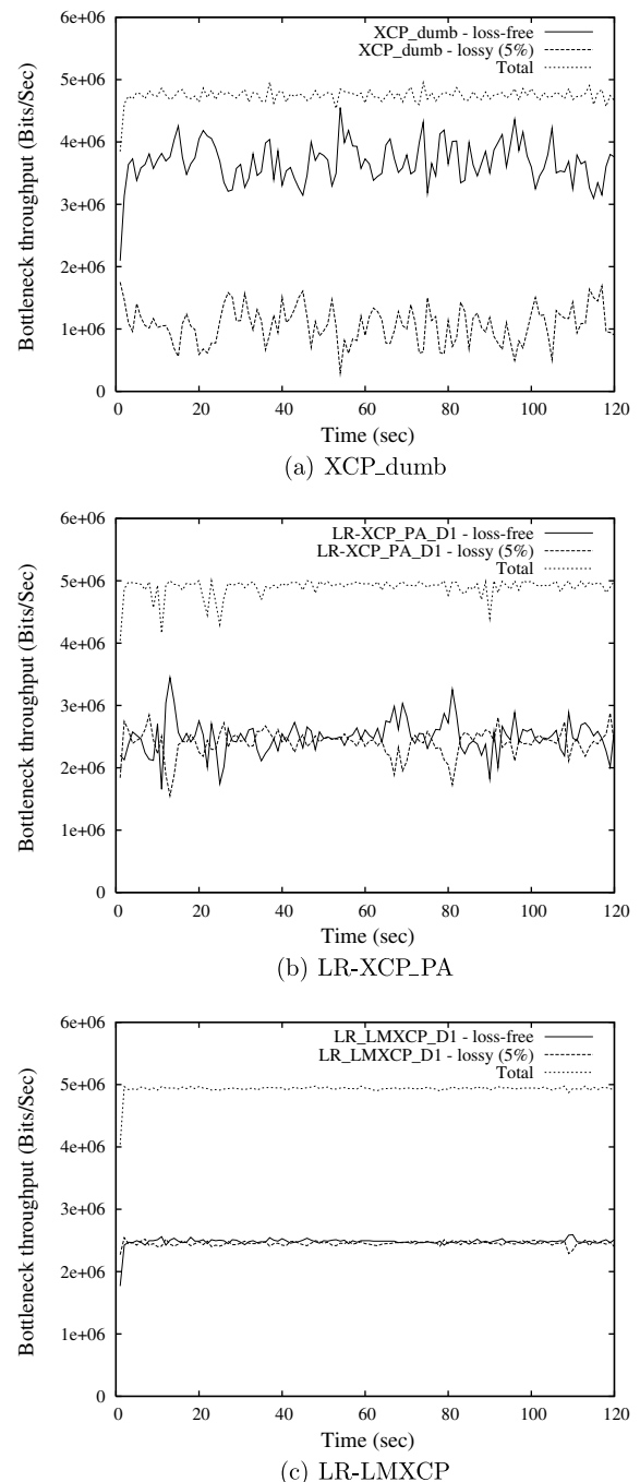
Fig. 2. Sums of throughputs measured respectively for loss-free and lossy flows. Sums of throughputs are plotted as a function of time, and loss rate is set to 5% for lossy connections. In all graphs, the dupackthreshold parameter is set to 1 (as indicated by D1).
