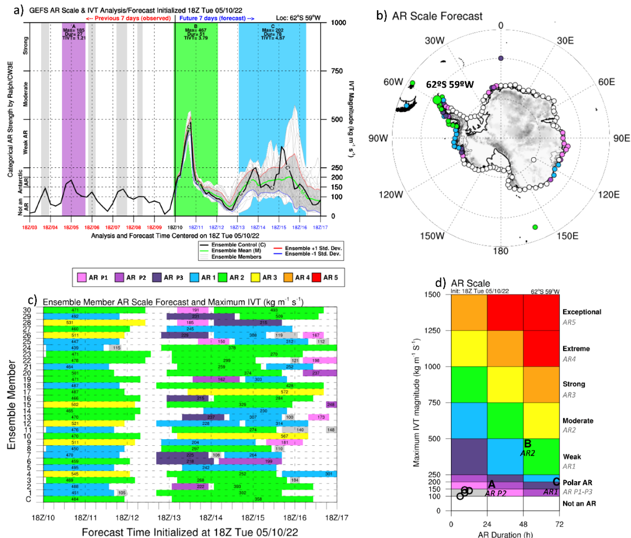
Figure 4. Example of CW3E Polar AR Toolkit on 10 May 2022 at the northern Antarctic Peninsula. (a) The plume diagram represents the integrated water vapor transport (IVT) forecast for each of the NCEP Global Ensemble Forecast System (GEFS) ensemble members (thin gray lines), the unperturbed GEFS control forecast (black line), the ensemble mean (green line), and plus or minus one standard deviation from the ensemble mean (red line (+), blue line (-), and gray shading). Colored shading represents the AR scale forecast for the given time, calculated using the model control forecast. (b) Dots on the map represent the maximum AR Scale forecast from the GEFS control member at that grid point for the next seven days. The enlarged dot indicates the location for panel (c) AR forecasts. (c): AR Scale magnitude and timing calculated for each GEFS ensemble member shaded according to scale. Values within the shading represent the magnitude and timing of maximum IVT during each forecasted AR at 62°S, 59°W. Gray shading in each panel represents IVT > 100 (kg m -1 s -1 ) for a duration less than 24 hours. (d) Letters represent where each AR identified by panel (a) (color shaded regions) fall on the Polar AR Scale matrix and how the AR scale is calculated for each. Circles correspond to vertical gray shadings in the panel (a) where IVT exceeds 100 (kg m -1 s -1 ) for less than 24 hours.
