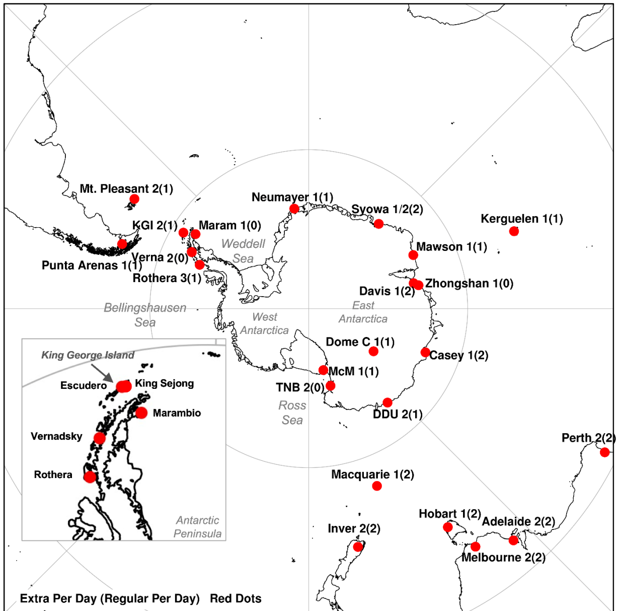
Figure 2: Stations releasing additional radiosondes during the winter TOPs. The number of additional radiosonde ascents each day are listed for each site next to the site names, and the number of regularly scheduled ascents are enclosed in parentheses. Abbreviated names have been used for Invercargill (Inver), Dumont d’Urville (DDU), Terra Nova Bay (TNB) where two sites are combined, McMurdo (McM), Vernadsky (Verna), King George Island again with two sites (KGI), and Marambio (Maram). The inset zooms up on the Antarctic Peninsula and observations from Escudero, King Sejong, and Vernadsky are employed in Figure 8.
