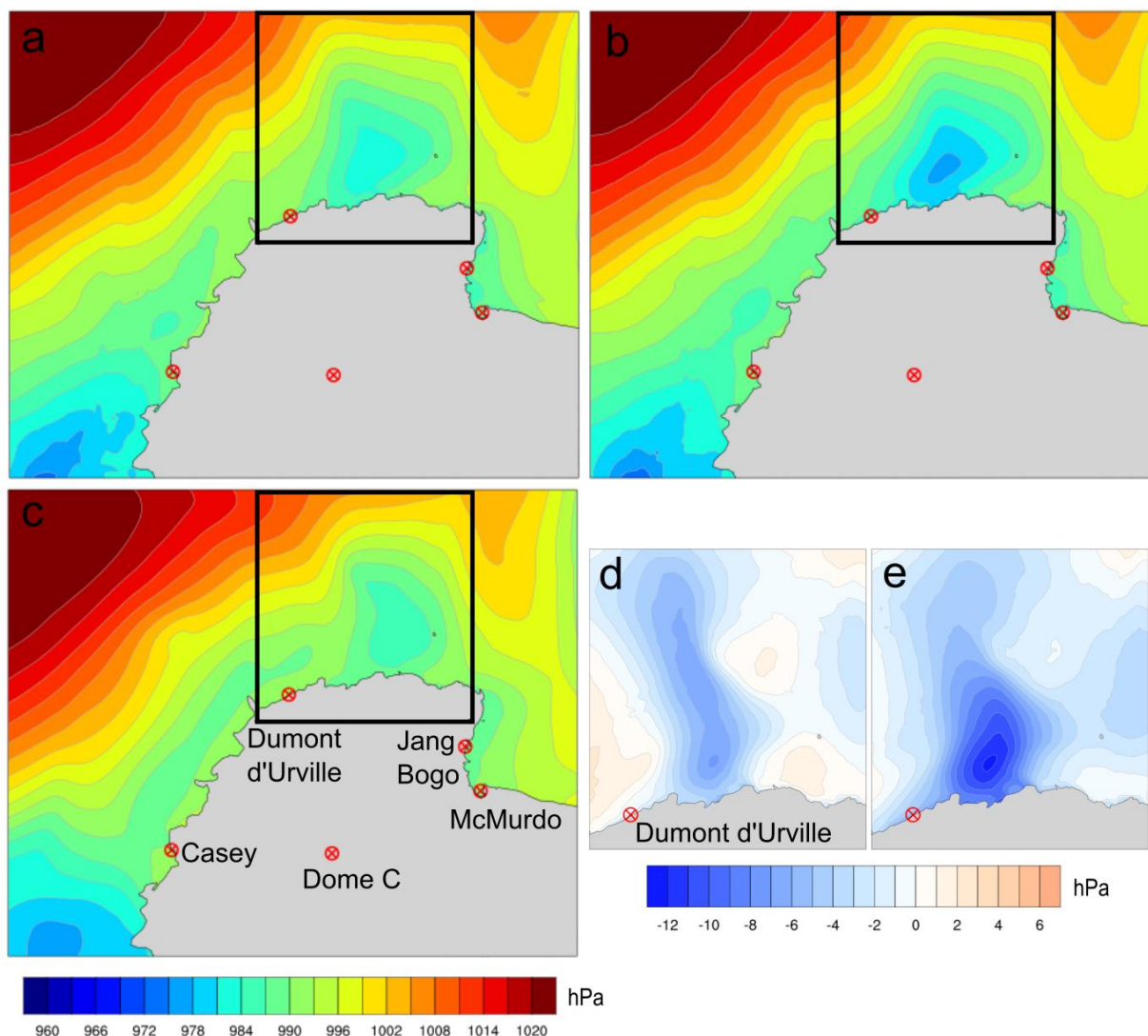
Figure 7. Mean sea level pressure at 1200 UTC 7 July 2022 during TOP3. (a) 60-hour TOP forecast assimilating extra radiosondes; (b) 60-hour TOP forecast without extra radiosondes; (c) ERA5 global reanalysis. (d) Bias of forecast (a) in relation to ERA5 adjacent to Dumont d'Urville station. (e) Bias of forecast (b) in relation to ERA5. Forecast initial time is 0000 UTC 5 July 2022. Sites releasing extra radiosondes during TOP3 are shown by red circles with a cross and are labelled in (c). Zoomed region for (d) and (e) shown in (a)-(c). Contour interval is 3 hPa in (a)-(c) and 1 hPa in (d) and (e).
