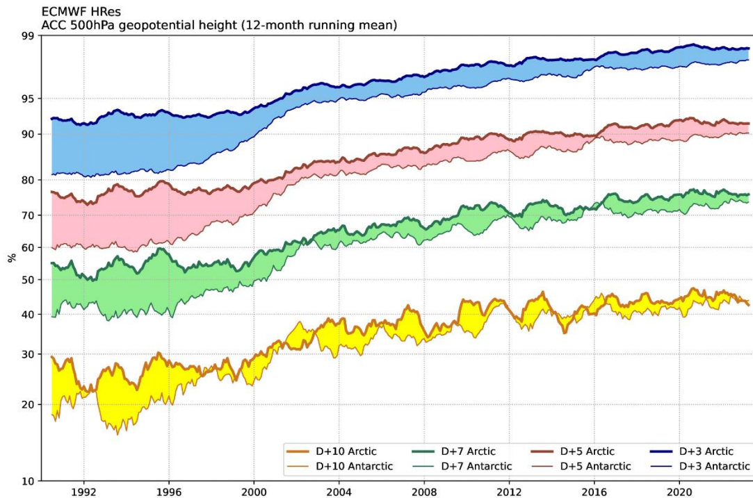
Figure 1: Evolution of forecast skill at different lead times (days 3, 5, 7, 10) in the Arctic (thick lines) and Antarctic (thin lines). Shown is the 12-month running mean of anomaly correlation coefficient (ACC in %) of 500 hPa geopotential verified against analysis for the high-resolution operational run (HRes) of ECMWF's Integrated Forecasting System (IFS). The difference in forecast skill between the two regions, indicated by the colored areas between the running-mean lines, decreased markedly in the late 1990s coinciding with the start of the satellite microwave radiance assimilation (e.g., Simmons and Hollingsworth 2002) but has remained nearly constant since then. The polar regions are defined here as north of 60°N and south of 60°S.
