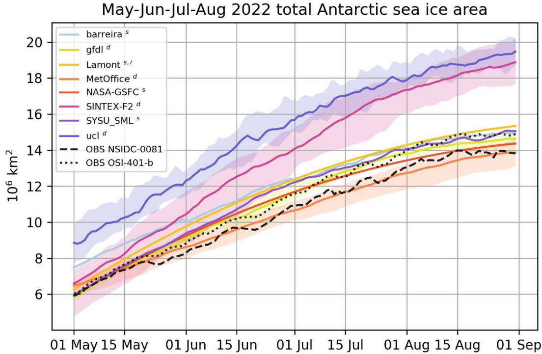
Figure 13: Temporal evolution of the total Antarctic sea ice area forecasted by eight groups and institutions participating in the Special Observing Period 2022 SIPN South experiment. The thick colored lines denote the forecast ensemble median while the shadings denote the ensemble ranges. The letters s and d in the legend refer to forecasts produced with statistical and dynamical models, respectively. The letter i expresses that the output has been interpolated (quadratically) from monthly to daily values. The two broken lines are observed sea ice areas from two satellite data sets.
