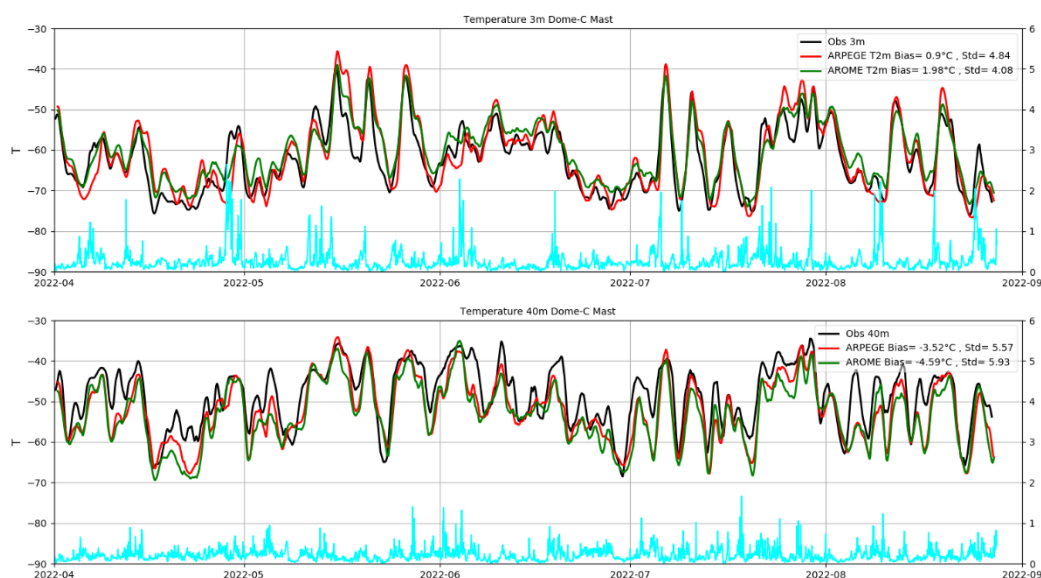
Figure 11: Time series of hourly temperature at 3 m (top panel) and 40 m (bottom panel) above ground from mast observations at Dome C (black lines, data courtesy C. Genthon), the ARPEGE output at the nearest grid point (red lines) and the mean of the 36 nearest grid points of AROME (green line). Blue lines show the AROME standard deviation based on the spatial variability among the 36 grid points. From 1 April to 31 August 2022.
