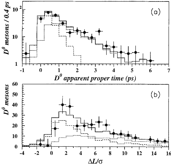
Fig. 2a, b. Apparent proper time distribution t = \Delta L \cdot M(D^0)/p(D^0) a and normalised decay length \Delta L/\sigma b for D^0 mesons from D^{*+} with X_E(D^{*+}) above 0.15, where both tracks ( K^- \pi^+ ) have hits in the vertex detector. The measured distribution after background subtraction is shown with data points. The simulated D^0 from c\bar{c} events (dashed histogram), simulated D^0 from b\bar{b} events (dotted histogram), and sum of the c\bar{c} and b\bar{b} contributions (solid histogram) assume \tau(B) = 1.3 ps and P_{b \rightarrow D^{*+}}/P_{c \rightarrow D^{*+}} = 0.87
