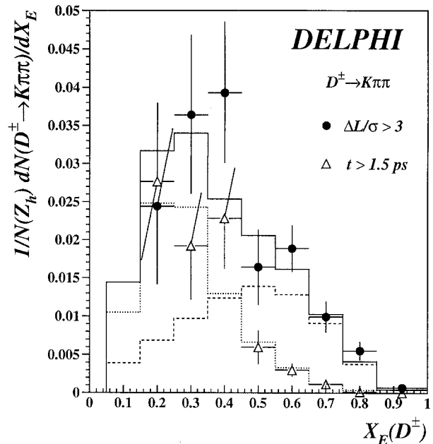
Fig. 8. X_E distributions of D^+ mesons with \Delta L/\sigma > 3 (full dots), or apparent proper time above 1.5 ps (triangles) where the 25% c\bar{c} contribution is subtracted. The histograms are as in Fig. 6
