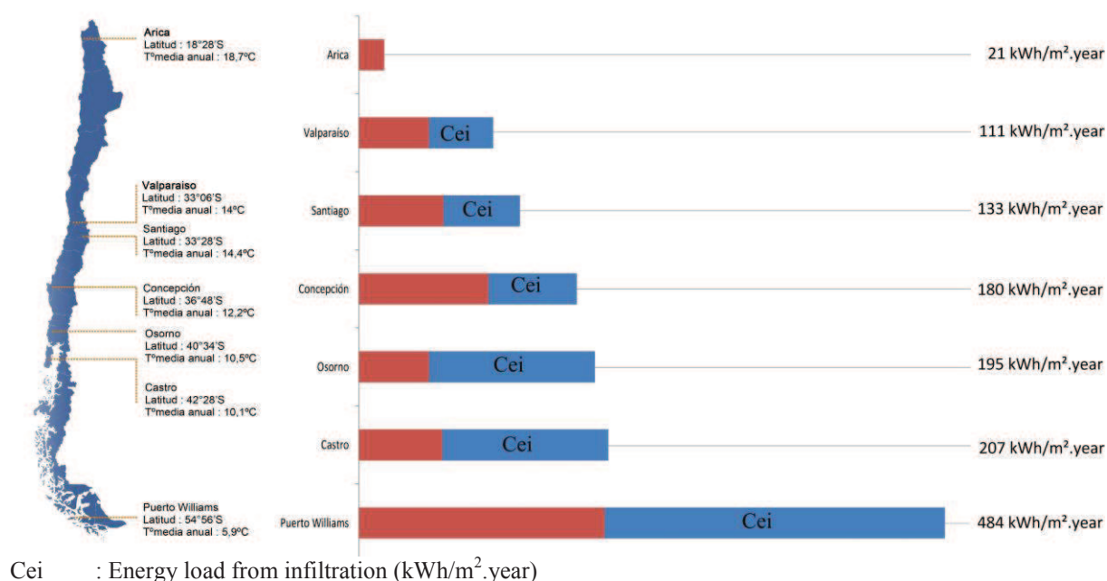
Figure: 1 Weighted energy demands by provincial capital with energy load from infiltration. Source: Bobadilla, 2014.
