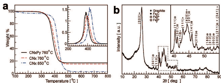
Figure 3. (a) Thermogravimetric analysis of N-CNT and PN-CNT. The latter are oxidized at lower temperature, indicating higher chemical reactivity. The larger amount of byproducts for lower temperature nanotubes is a consequence of a higher proportion of metal particles as a result of shorter nanotubes. The inset shows that the oxidation onset for PN-CNT occurs 15 °C below the onset for N-CNT grown under the same conditions. (b) X-ray diffraction pattern of PN-doped CNTs (sample B). The inset shows enlargement of the region between 40 and 55°. The metal particles in the sample are a mixture of \text{Fe}_3\text{C} , \text{Fe}_2\text{P} , and \text{Fe}_3\text{P} . The mean particle sizes are 10–12, 13, and 17 nm, respectively.
