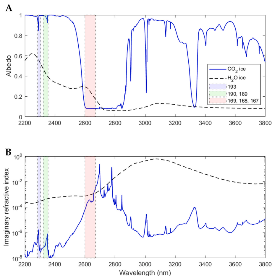
Fig. 1. (A) Simulated \text{CO}_2 ice (solid blue line; equivalent grain size of 10 mm, see Section 5.3) and \text{H}_2\text{O} ice (dashed black line, equivalent grain size of 0.3 mm) albedo spectra using the Planetary Spectrum Generator (PSG) tool (see Section 5.3, Villanueva et al., 2018) over the LNO spectral range. The different orders mentioned in the text (orders 167, 168, 169, 189, 190 and 193) are highlighted in blue, green and red (see figure legend). (B) Imaginary refractive index for \text{CO}_2 ice (Hansen, 2005) and \text{H}_2\text{O} ice (Warren and Brandt, 2008) describing the absorption coefficient over the LNO spectral range. Same legend as panel A. (For interpretation of the references to colour in this figure legend, the reader is referred to the web version of this article.)
