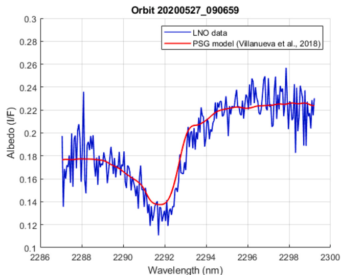
Fig. 10. PSG fit on the 2.29 \mu\text{m} CO 2 ice absorption band well present in the LNO spectrum (orbit 20200527_090659). A reduced \chi^2 of 0.15 is obtained. See line 3 in Table 1 for more details.
