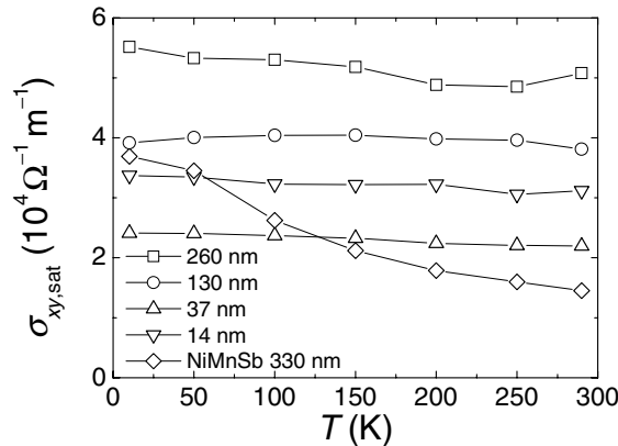
Figure 4. Saturation anomalous Hall (AH) conductivity versus temperature for Co 2 MnSi:GaAs and NiMnSb:GaAs films.
