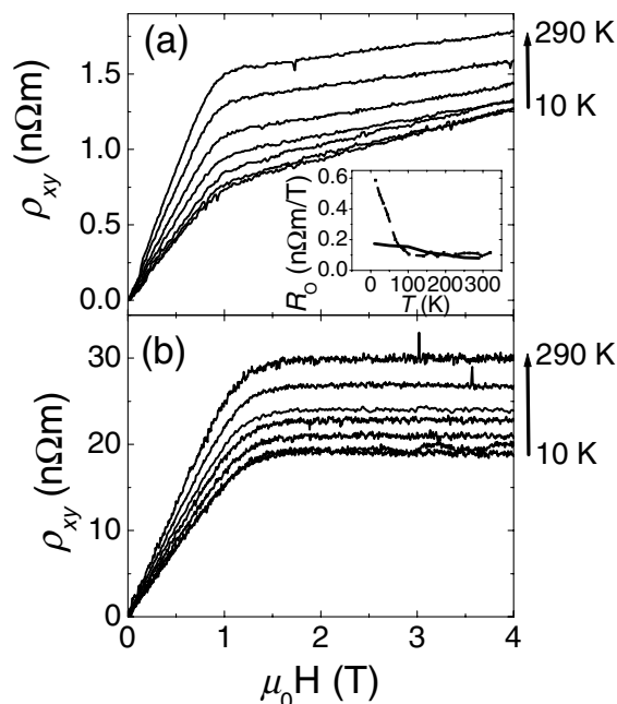
Figure 2. Hall resistivity versus field at 10, 50, 100, 150, 200, 250 and 290 K for (a) 330 nm NiMnSb film and for (b) 260 nm Co 2 MnSi film. Inset: ordinary Hall constant versus temperature for NiMnSb film (solid line) and bulk data taken from Otto et al [20].
