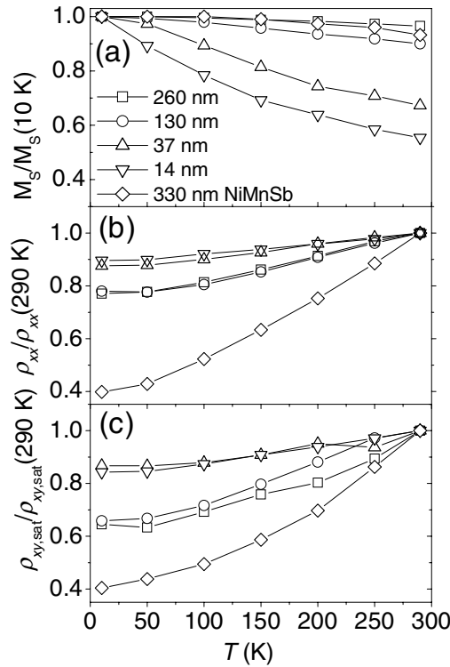
Figure 3. (a) Normalized saturation magnetization versus temperature of the \text{Co}_2\text{MnSi} and \text{NiMnSb} films; (b) normalized longitudinal resistivity versus temperature. Symbol shapes are as in figure 3(a). (c) Normalized saturation Hall resistivity. Symbol shapes are as in figure 3(a).
