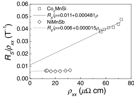
Figure 5. AH constant divided by resistivity versus resistivity, for the 260 nm \text{Co}_2\text{MnSi} :GaAs and 330 nm \text{NiMnSb} :GaAs films. Symbols represent data and dashed lines linear fit with the fit parameters shown in the figure caption.
