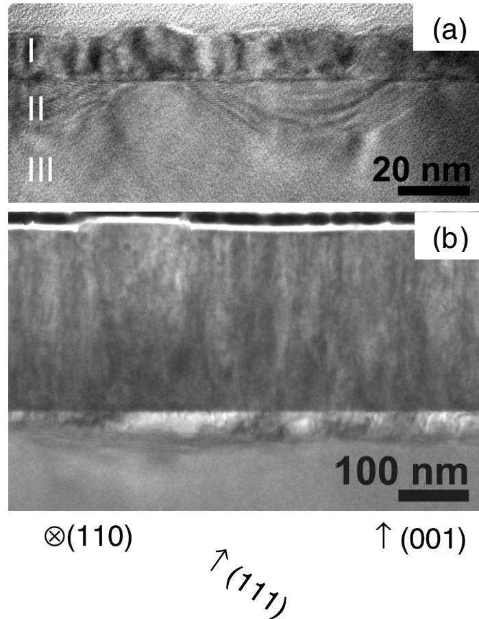
Figure 1. TEM bright field images of cross-section \text{Co}_2\text{MnSi} film deposited on GaAs (001) substrate. Zone axis is (110). Regions labelled as follows: I: \text{Co}_2\text{MnSi} film, II: reaction zone III: GaAs substrate.
