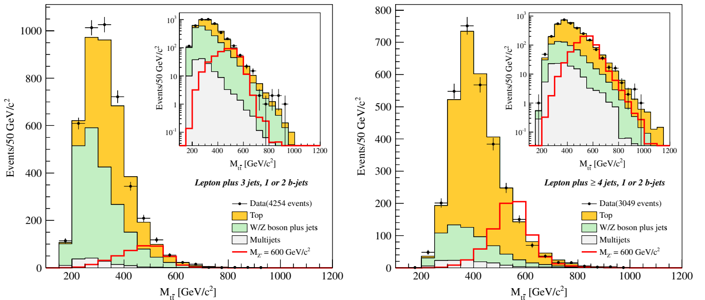
FIG. 1 (color online). Reconstructed M_{t\bar{t}} for the three-jet events (left) and four-or-more-jet events (right). The distribution of the M_{t\bar{t}} spectrum is on a linear scale, and the inset shows a logarithmic scale of the same distribution. The background expectation is normalized to the best fit to the data. The red histogram shows the expectation for a 600 \text{ GeV}/c^2 mass hypothesis for the leptophobic top-color resonance normalized to the predicted cross section.
