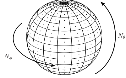
Figure 3: Discretized sphere surface \mathcal{S}_d with N_\theta = 16 latitudes and N_\phi = 16 longitudes (256 pixels)
