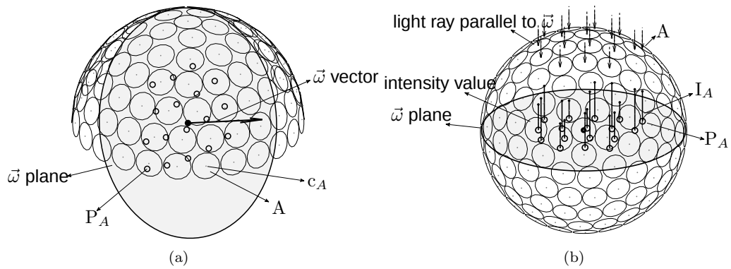
Figure 6: (a) projection of the camera centers contributing in direction \vec{\omega} onto the planar surface normal to \vec{\omega} (b) another view point of the camera centers projection onto the planar surface normal to \vec{\omega}
