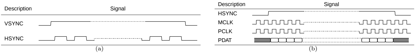
Figure 12: (a) Timing diagram for VSYNC and HSYNC, (b) timing diagram for HSYNC, MCLK, PCLK and pixel data
