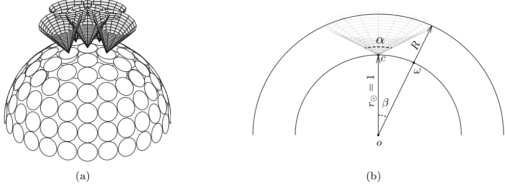
Figure 8: (a) Pinhole cameras with isotropic angle-of-view on the Panoptic device; for the sake of clarity, only five cameras are modeled in this figure, (b) intersection of the isotropic angle-of-view boundary and the spherical surface of radius R
