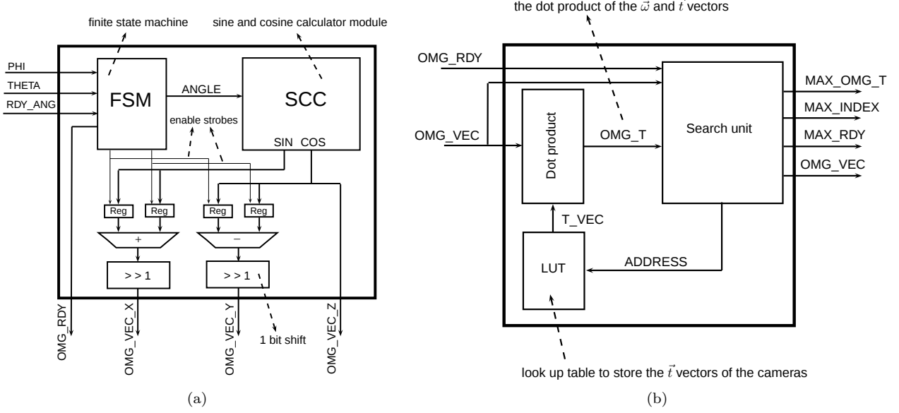
Figure 16: (a) Internal architecture of the omega vector generation module with one sine and cosine calculator module; (b) the nearest camera position finder module
