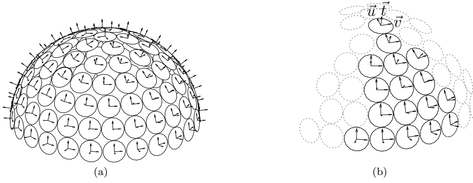
Figure 4: (a) radial and tangential vectors identifying the target direction and the coordinates of the cameras image frame plane, (b) zoomed portion of the previous picture
