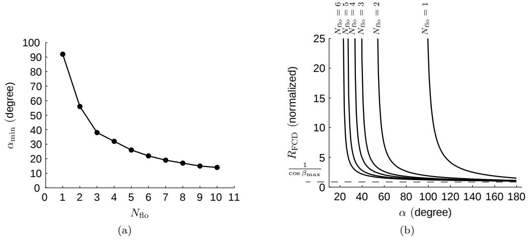
Figure 9: (a) Minimum AOV for the cameras of the Panoptic device with N_{\text{flo}} + 1 latitude floors, (b) R_{\text{FCD}} vs AOV of the Panoptic device.
