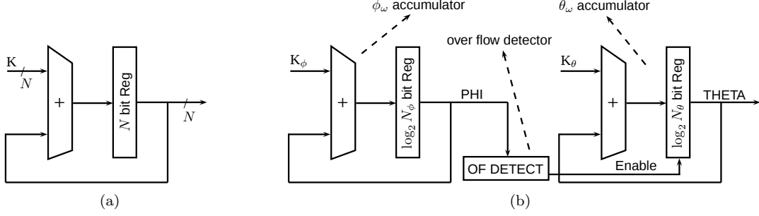
Figure 15: (a) An N bit accumulator, (b) \phi_\omega and \theta_\omega generation accumulators
