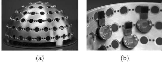
Figure 2: (a) Side view, (b) and internal view of the fabricated Panoptic camera with individual imagers
