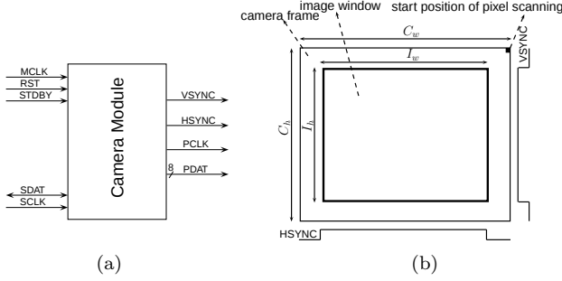
Figure 11: (a) camera module interface, (b) camera frame
