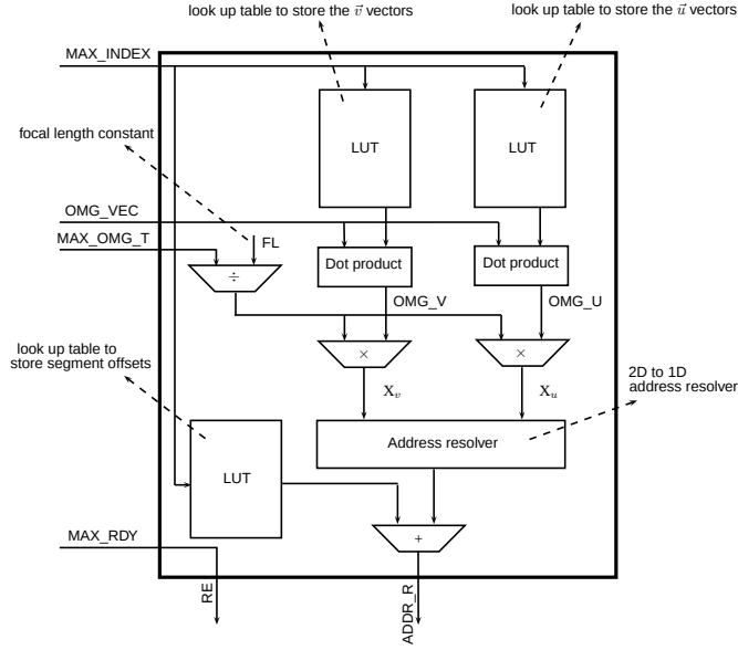
Figure 17: Internal architecture of the pixel position generation module
