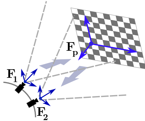
Figure 19: Extrinsic parameter calibration principles
