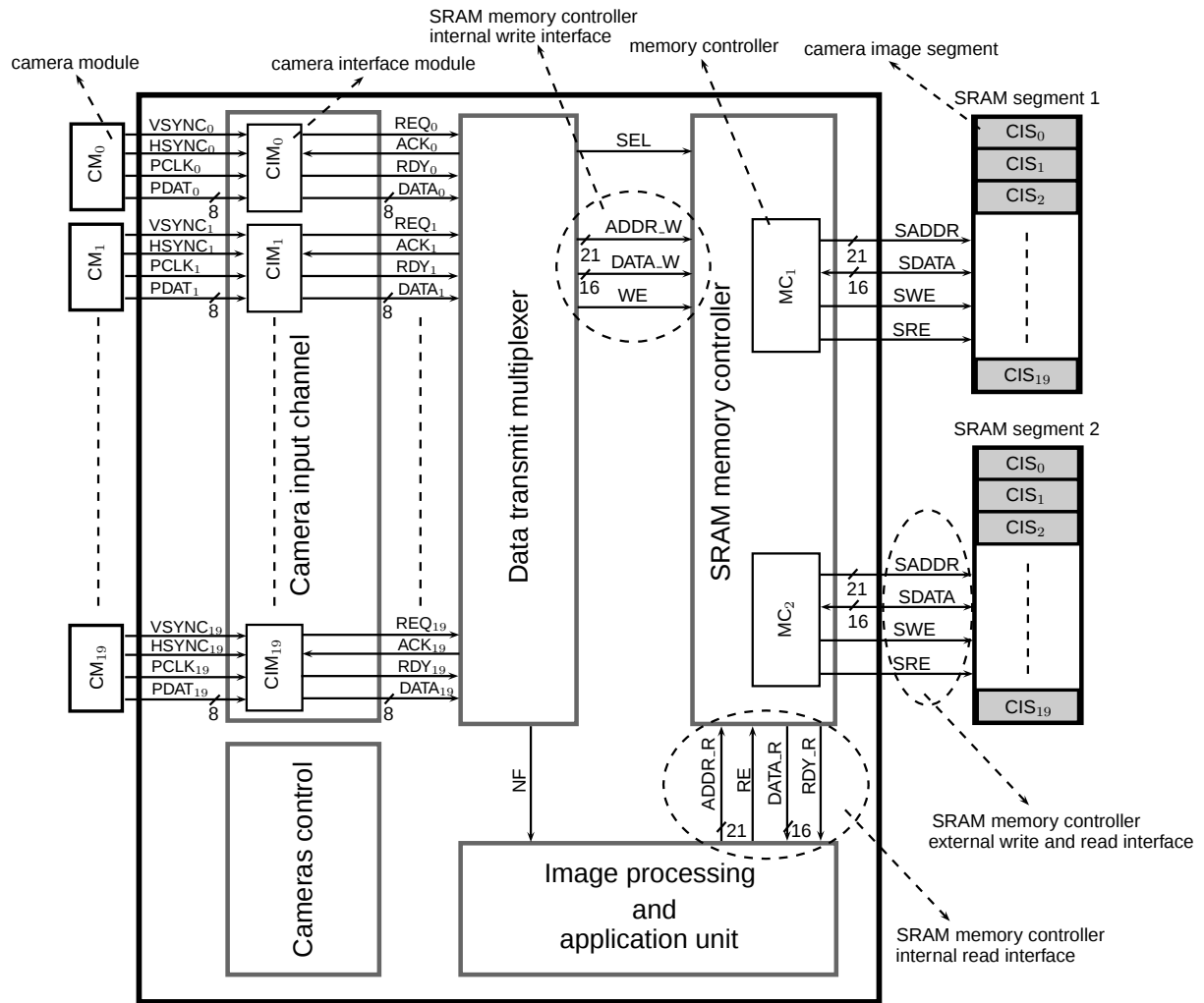
Figure 13: Architecture of the concentrator FPGA. For the sake of clarity the camera module connections to the cameras control unit and the data link and control unit are not shown in this picture.
