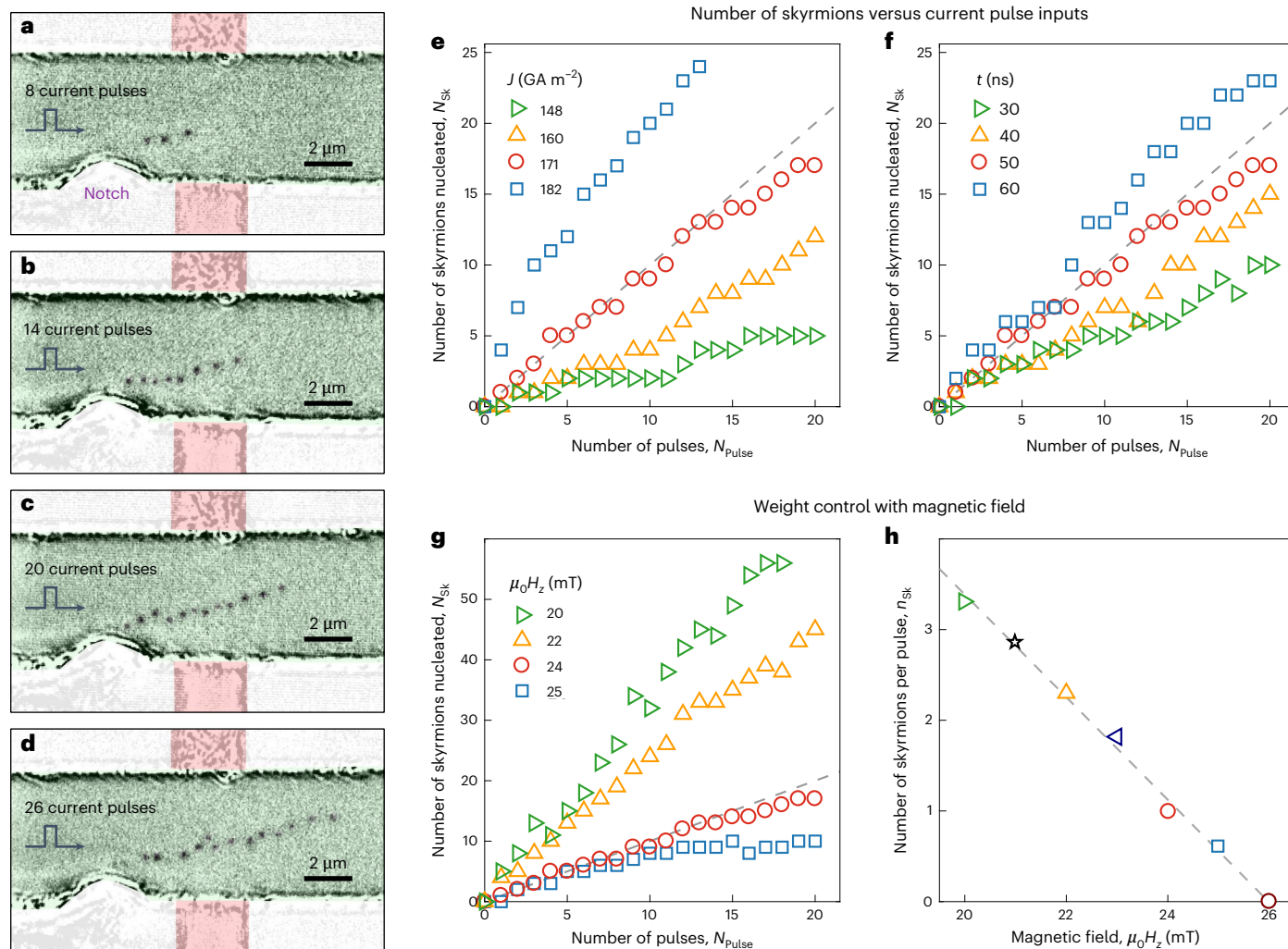
Fig. 2 | Controlled nucleation of magnetic skyrmions at a notch using current pulses as inputs and weight fine-tuning. a–d , Kerr microscopy images of the device shown in Fig. 1d, after the application of 8 ( a ), 14 ( b ), 20 ( c ) and 26 ( d ) current pulses at J = 160 GA m -2 , t = 50 ns and \mu_0H_z = 24 mT. e, f , Number of skyrmions nucleated in the track, N_{sk} , with the number of pulses applied, N_{pulse} , (fixed \mu_0H_z = 24 mT) for several current densities J with fixed t = 50 ns ( e ) and for several pulse durations t with fixed J = 171 GA m -2 ( f ). g, h , Control of weight using
