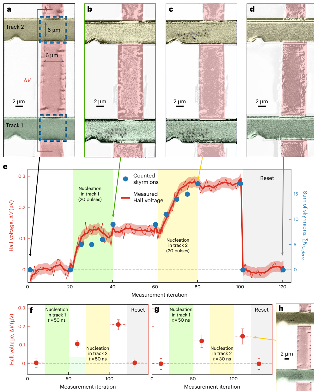
Fig. 4 | Weighted sum in a device composed of two parallel multilayer tracks. a–d , Kerr microscopy images of the device composed of two 6-μm-wide parallel magnetic multilayer tracks connected by a transverse 6-μm-wide Ta Hall electrode. After the saturation of the track using \mu_0 H_z = 200 mT ( a ), skyrmions can be selectively nucleated in track 1 ( b ) and track 2 ( c ), before being erased by another \mu_0 H_z = 200 mT ( d ). e , \Delta V (in red) and the corresponding sum of the skyrmion number detected in both tracks \sum N_{sk,detec} (in blue) for the successive injection of skyrmions in the tracks. Twenty nucleation pulses are successively applied to each track (green- and yellow-shaded areas for tracks 1 and 2, respectively) using a current pulse of about 116 \text{ GA m}^{-2} and 50 ns, at \mu_0 H_z = 20 mT.
