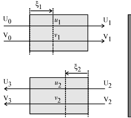
Figure XI-1: FDNLM scheme.
