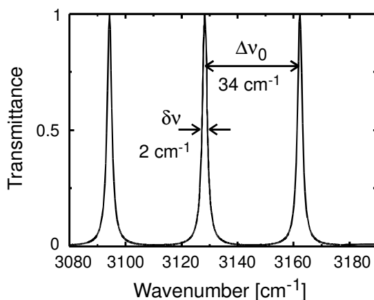
Figure IX-3: Transmission spectrum of an etalon plate of 0.1 mm thickness, the refractive index n = 1.47 and finesse of about F = 17 , in the case of normal incidence.
