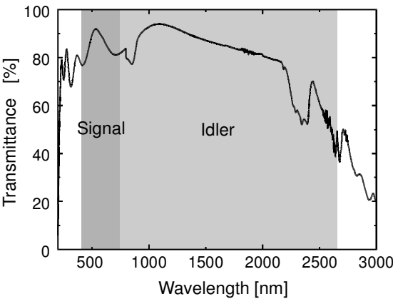
Figure VIII-2: Transmittance of 4-mm thick BBO crystal. The antireflection coatings for 532 and 1064 nm alter the transmittance in the visible spectral region.
