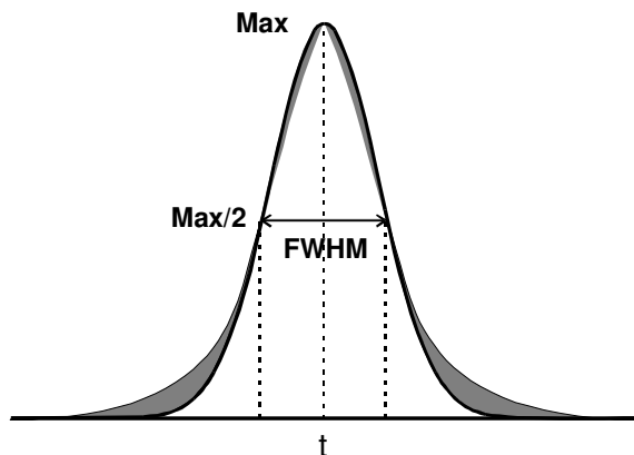
Figure V-9: The dark line is a Gaussian profile that matches the maximum and the FWHM of the deformed pulse. The gray surface area divided by the Gaussian area gives the Gaussian shape factor (GSF).
