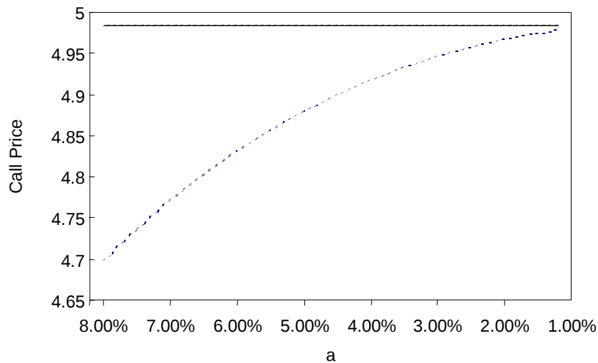
Figure 1 : Convergence of option prices : marked Poisson process
