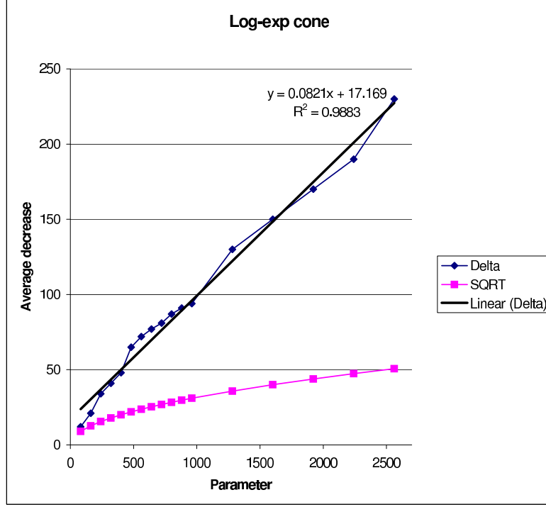
Figure 1: Average decrease of the potential for log-exp cone.
