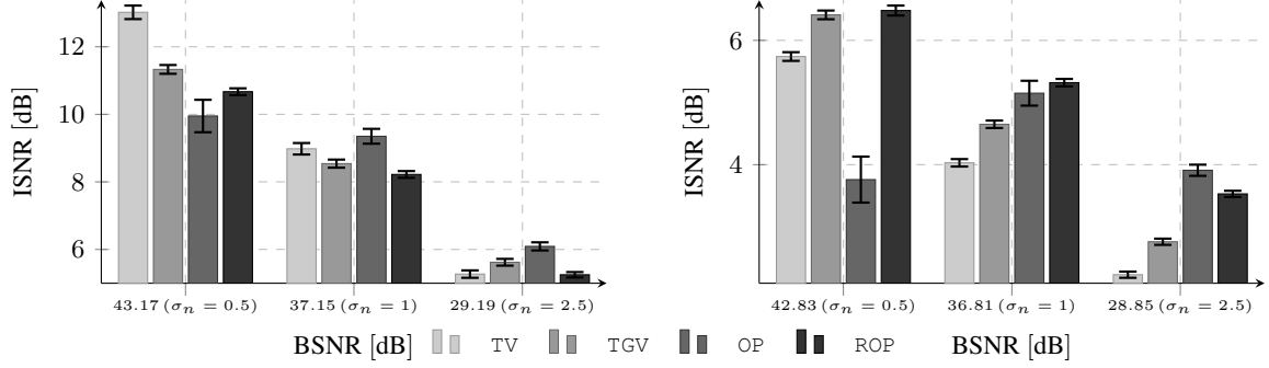
Fig. 5. Mean ISNR (100 realizations) of 2D images of size 128 \times 128 restored with different methods (TV, TGV, OP and ROP). Original images are blurred by Gaussian unimodal kernel (left: \sigma = 1.2 , right: \sigma = 2 , |\text{supp}| = 13 \times 13 ) and corrupted by additive Gaussian noise ( \sigma_n = 0.5 , \sigma_n = 1 and \sigma_n = 2.5 ). Error bars represent the standard deviation of the sample.
