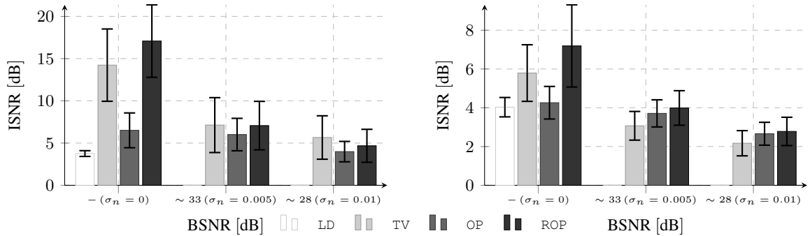
Fig. 3. Mean ISNR (100 realizations) of 1D piecewise-cubic signals of length N = 1001 in \mathcal{C}(S) (left: S = 7 , right: S = 47 ) restored with different methods (LD, TV, OP and ROP). Original signals are blurred by Gaussian unimodal kernel ( \sigma = 2 , |\text{supp}| = 13 ) and corrupted by additive Gaussian noise ( \sigma_n = 0 , \sigma_n = 0.005 and \sigma_n = 0.01 ). Error bars represent the standard deviation of the sample.
