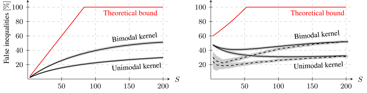
Fig. 2. Mean proportion (1000 realizations) of wrong inequalities in \mathbf{A}_H as a function of the number of sub-domains S for 1D piecewise-linear signals in \mathcal{C}(S) ( N = 1001 ) blurred by Gaussian unimodal or bimodal kernel ( \sigma = 2 , |\text{supp}| = 13 ) and (right) corrupted by Gaussian noise ( \sigma_n = 0.01 ). Solid lines: \mathbf{A}_H computed from \mathbf{z} ; dashed lines: \mathbf{A}_H computed from \hat{\mathbf{v}} . Gray areas represent the standard deviation.
