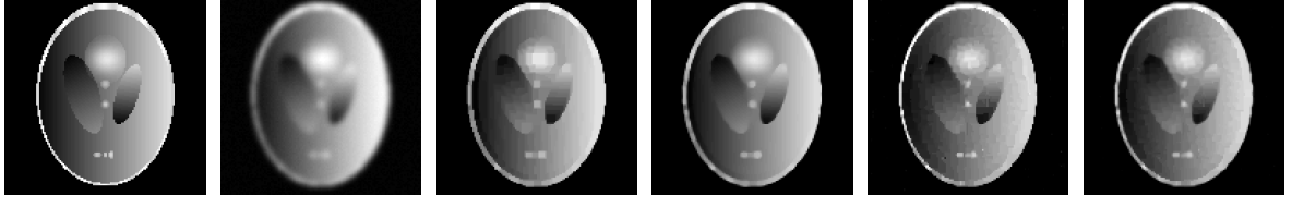
Fig. 4. Results on synthetic data. From left to right: original image, corrupted image (convolution with isotropic Gaussian kernel ( \sigma = 2 , |\text{supp}| = 13 \times 13 ) and corruption with additive Gaussian noise ( \sigma_n = 1 )), TV, TGV, OP and ROP restored images.
