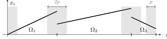
Fig. 1. Signal \mathbf{x} \in \mathcal{C}(3) on \Omega = \Omega_1 \cup \Omega_2 \cup \Omega_3 . Preservation of order relationships is uncertain for elements at the boundaries of \Omega and at the junctions between sub-domains.
