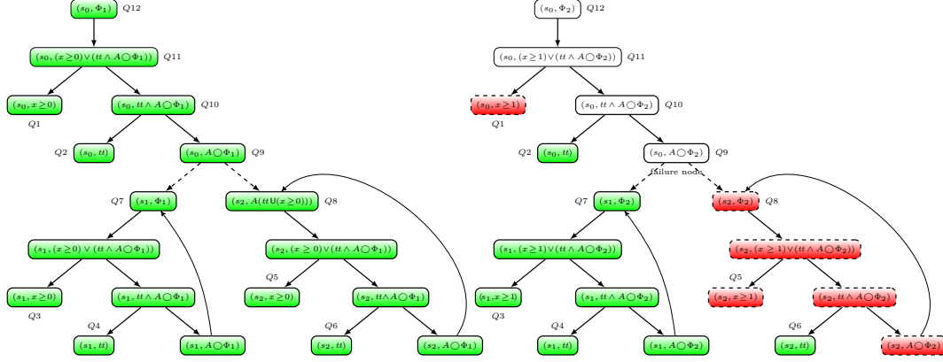
Figure 27: G_{\alpha^{\text{gen-join}}(M_1) \times \Phi_1} .
