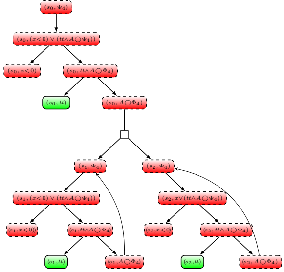
Figure 30: G_{\alpha^{\text{gen-join}}(M_1) \times \Phi_4} .
