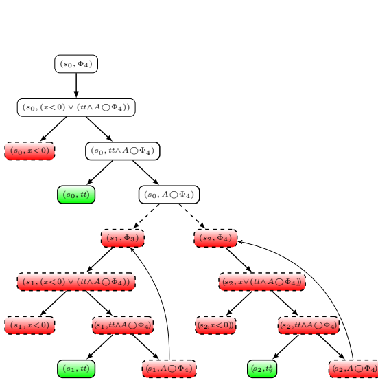
Figure 29: G_{\alpha^{\text{join}}(M_1) \times \Phi_4} .
