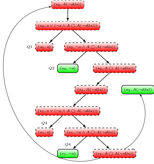
Figure 14: G_{\pi_{\llbracket c \wedge \neg f \rrbracket}(\mathcal{F}_1) \times \Phi_1}
