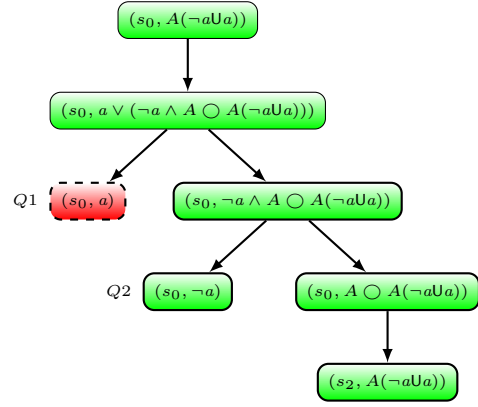
Figure 15: G_{\pi_{\llbracket c \wedge f \rrbracket}(\mathcal{F}_1) \times \Phi_1}
