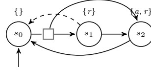
Figure 19: GMTS \alpha^{\text{gen-join}}(\mathcal{F}_1) .
