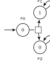
Figure 22: \alpha^{\text{gen-join}}(M_1) .
