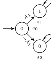
Figure 20: M_1 .
