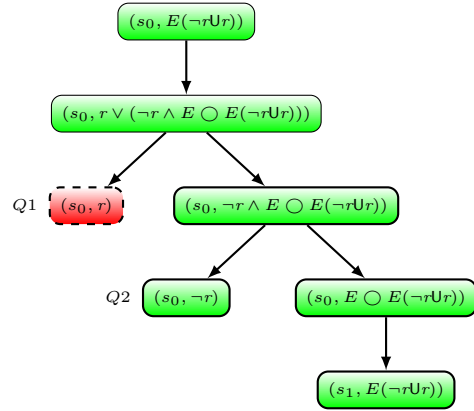
Figure 17: G_{\alpha^{\text{join}}(\pi_{\llbracket \neg f \rrbracket}(\mathcal{F}_1)) \times \Phi_2}
