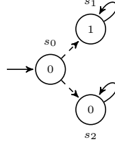
Figure 21: \alpha^{\text{join}}(M_1) .
