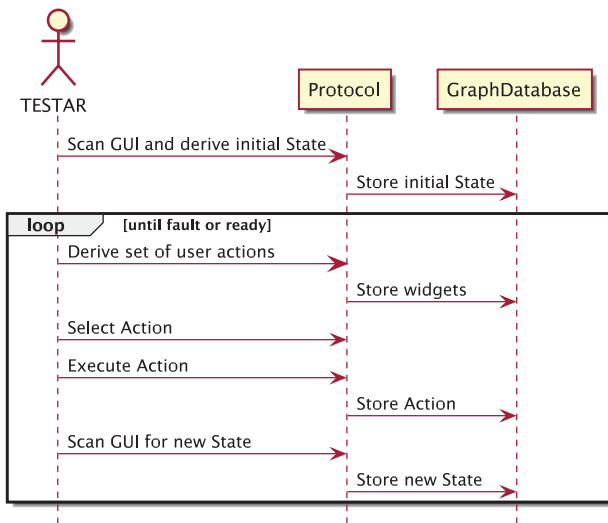
Fig. 3. Storing State, Widget and Action during the execution of an application in TESTAR
