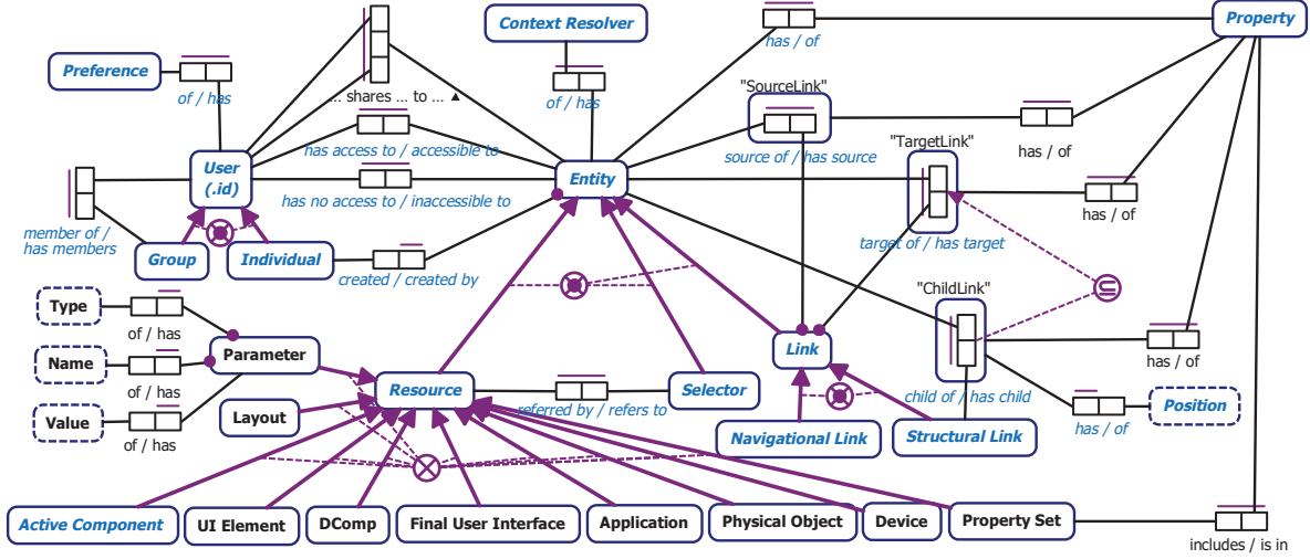
Fig. V.1: Conceptual model based on RSL
