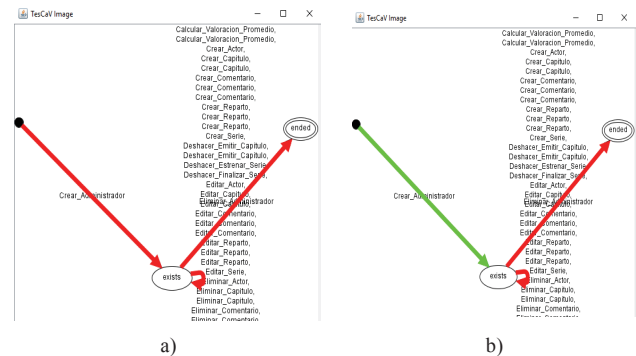
Fig. 4. Selected AT criterion: a) not covered transition, b) covered transition
