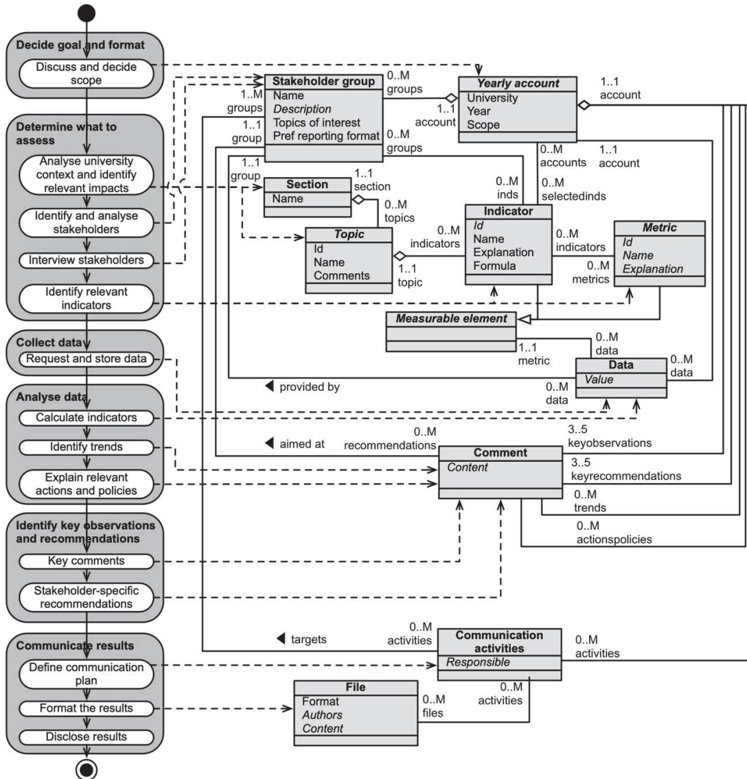
Fig. 3. PDD of the UniSAF method [10], created by analysing the method documentation and tools. Elements in italics denote that the concept was implicit an unnamed in the method documentation. For instance, the method manual does not mention Topic explicitly, but they refer to occasionally impacts and issues; the Excel tool collects the names of topics but does not label the concept itself. Similarly, Metric is not explicitly distinguished from Indicator.
