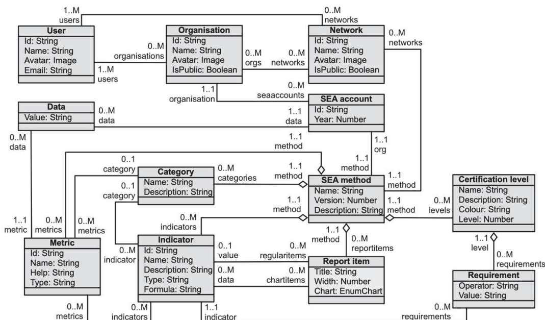
Fig. 4. openSEA DSL metamodel (i.e. underlying model of the openSEA tool). We have added some concepts and relationships that are not related to the DSL per se, but are needed to manage and use the tool (e.g. the concepts Organisation , Network , User , SEA account and Data )
