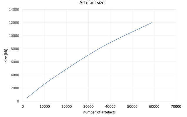
Fig. 8. Disk usage versus the number of artefacts
