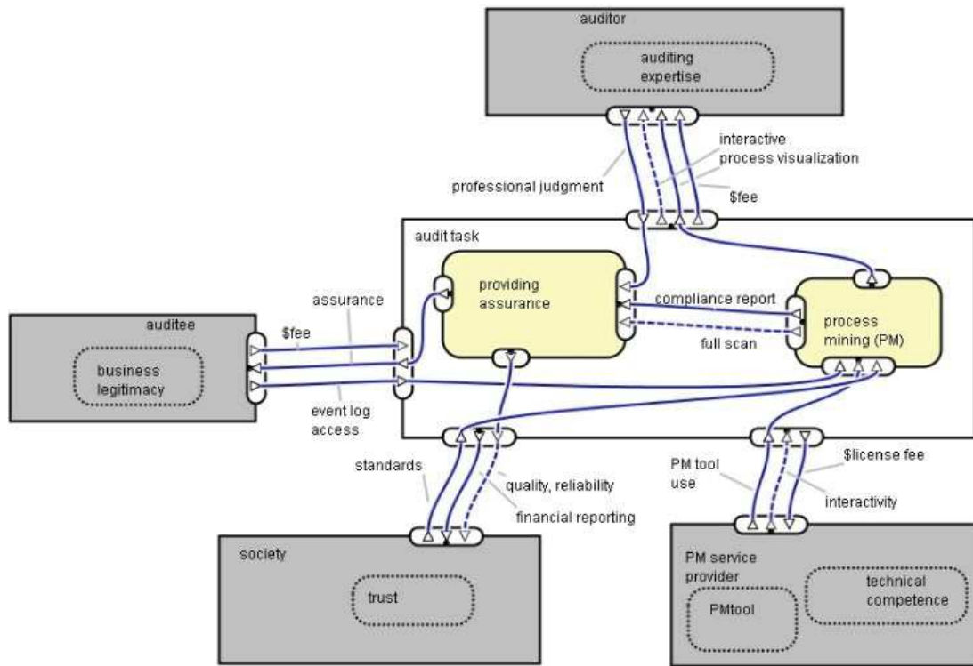
Fig. 5 Value Encounter model Process Mining application
