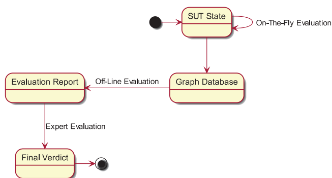
Fig. 5. Accessibility oracle types in TESTAR
