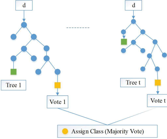
Fig. 3. Classification phase of random forest classifier
