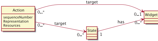
Fig. 2. Main structure of the internal model of the SUT constructed by TESTAR during test execution
