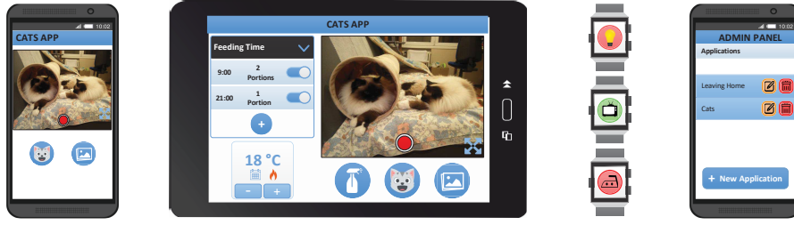
Fig. III.1: Mock-up of Lucy’s cats application (smartphone), Lucas’ version (tablet), his leaving home application (smartwatch) and the administration panel
