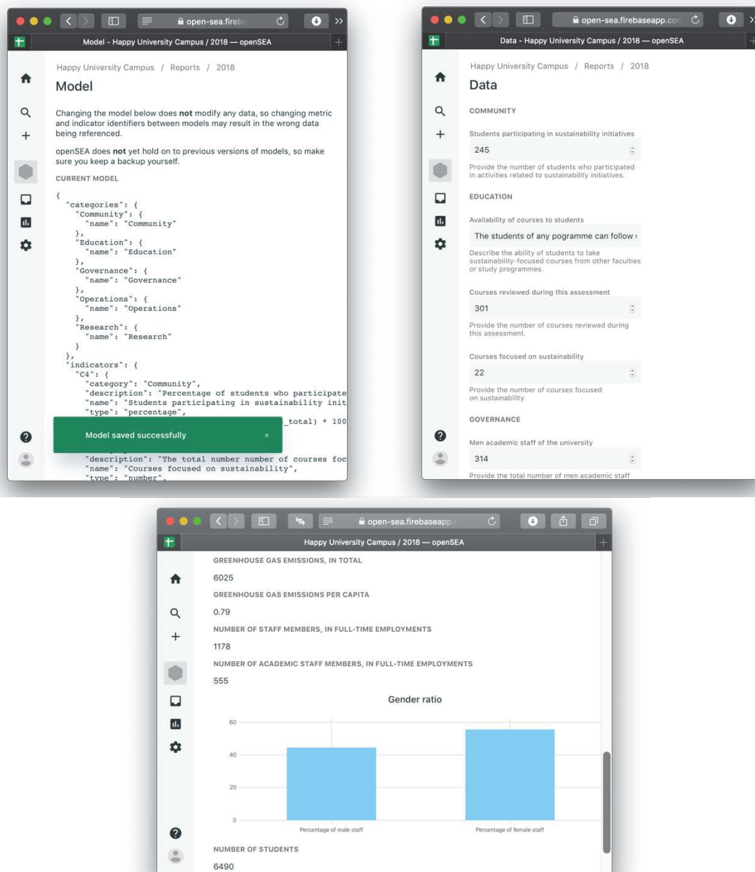
Fig. 5. Three screenshots of the openSEA tool. On the top-left, the tool informs that the model chosen for the UniSAF accounting of the (fictional) Happy University has been successfully loaded; find a fragment of this model is Appendix D. Every time a user uploads an updated version of the model (or an additional model), the tool interprets it (merging the models if required) and updates the other screens accordingly. On the top-right, the screen supporting the “Collect data” activity of UniSAF, based on the specification of metrics; see the field corresponding to the metric Men academic staff of the university , mentioned earlier. On the bottom, the screen reporting the results of the SEA account. The Gender ratio report item is displayed as a bar chart, whereas the rest are displayed as numbers, as specified in the method model.
