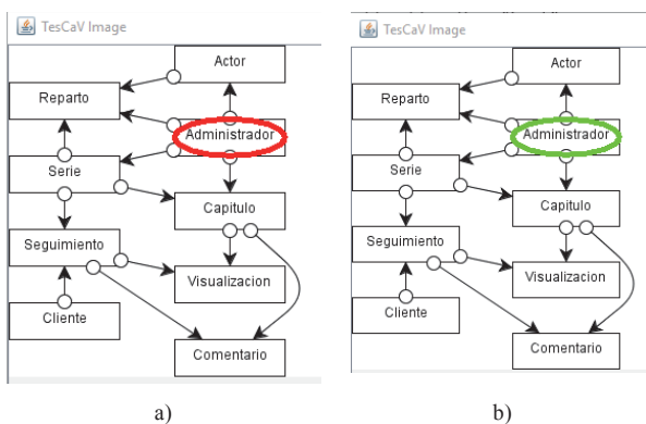
Fig. 3. Selected CA criterion: a) not covered entity, b) covered entity.
