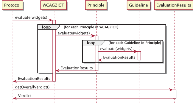
Fig. 6. Sequence diagram for accessibility evaluation with TESTAR
