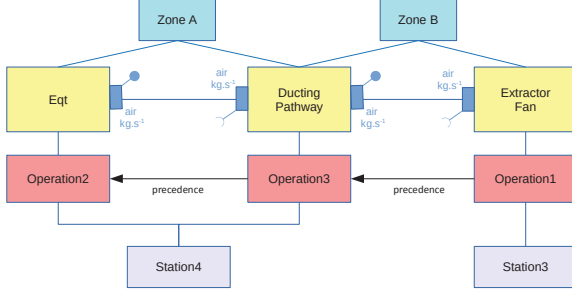
Fig. 3. Example model instantiation at level N + 1 .
