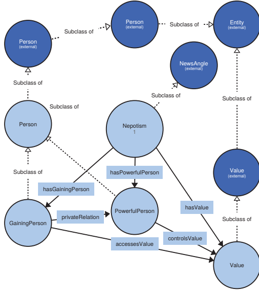
Fig. 4. An OWL representation of the nepotism angle.
