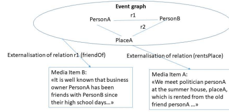
Fig. 5. Externalisation of entities and relations
