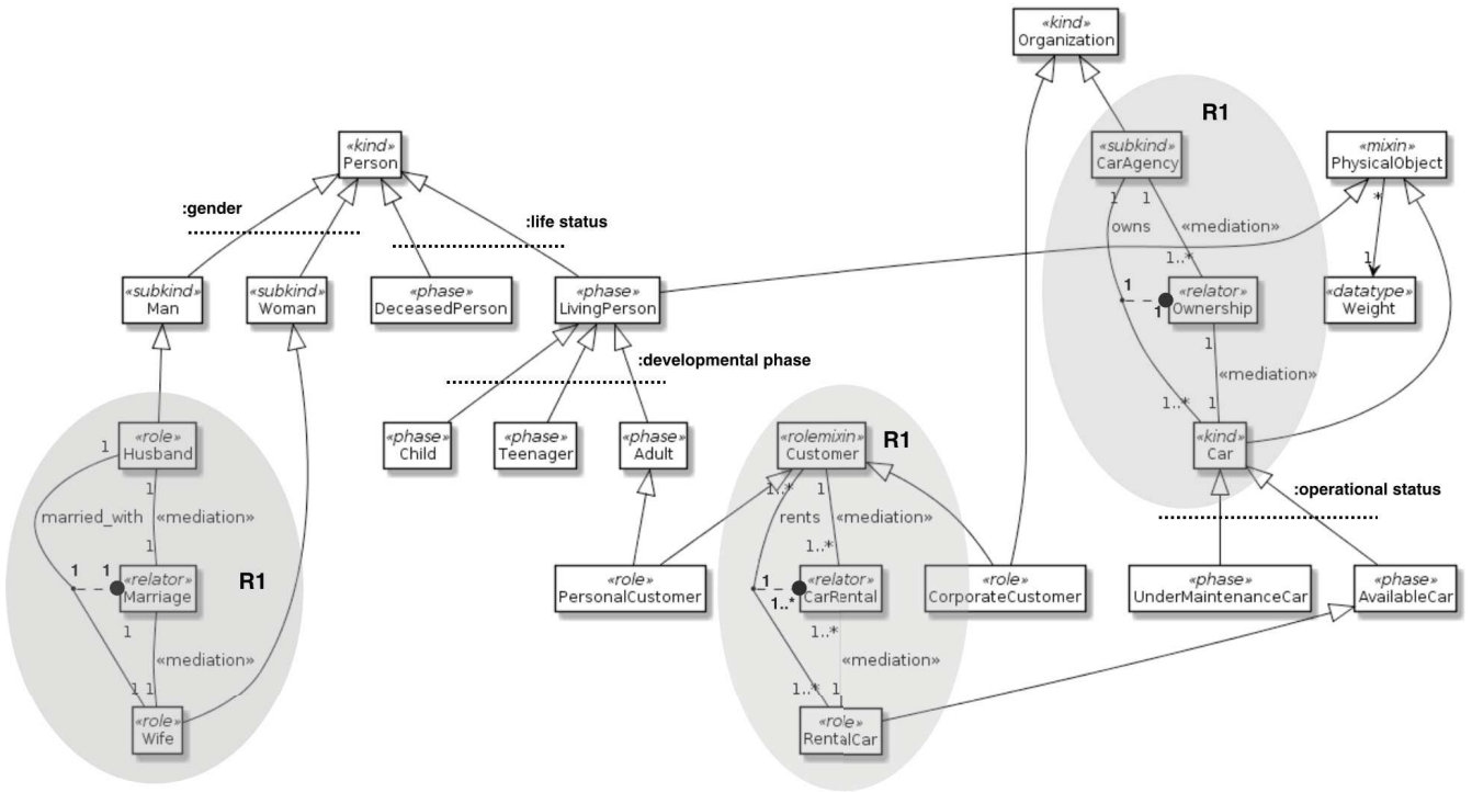
Fig. 1. An Example of an OntoUML Model.
