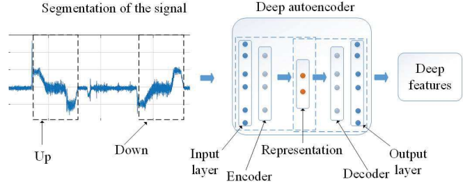
Fig. 2. Deep autoencoder feature extraction approach
