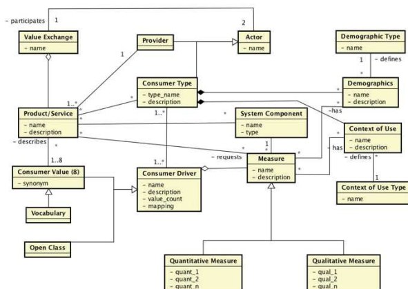
Fig. 1. Consumer Preference MetaModel
