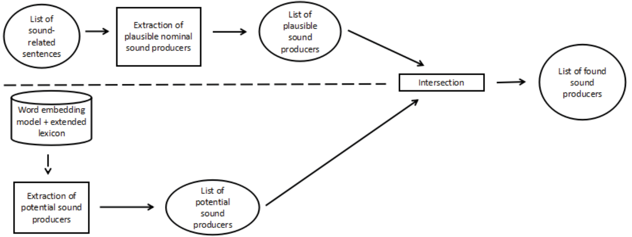
Fig. 3. Details of the method based on word embeddings
