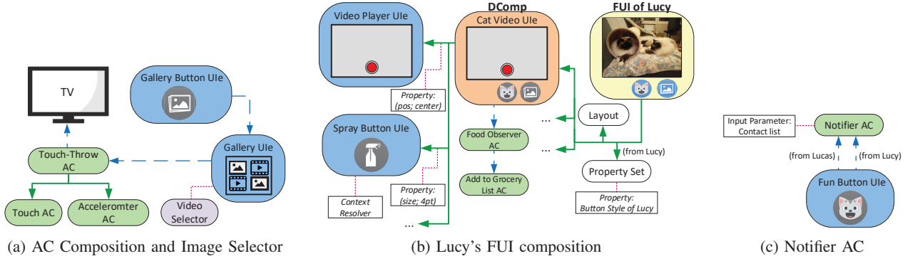
Fig. V.2: Examples of conceptual model instantiations
