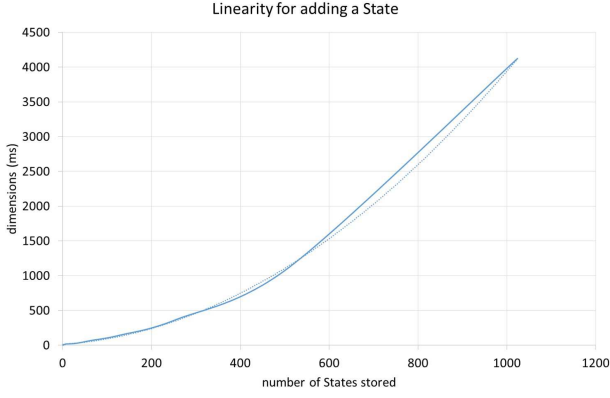
Fig. 7. Linearity for adding a state
