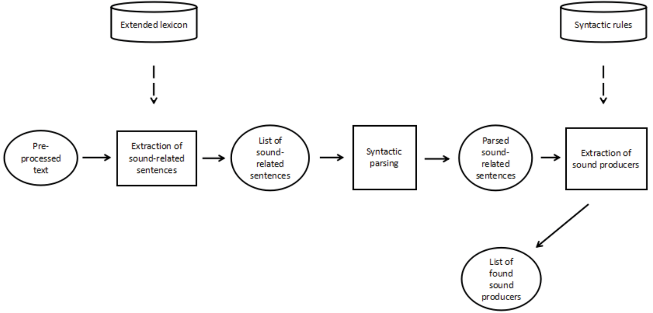
Fig. 2. Step of the method based on dependency parsing
