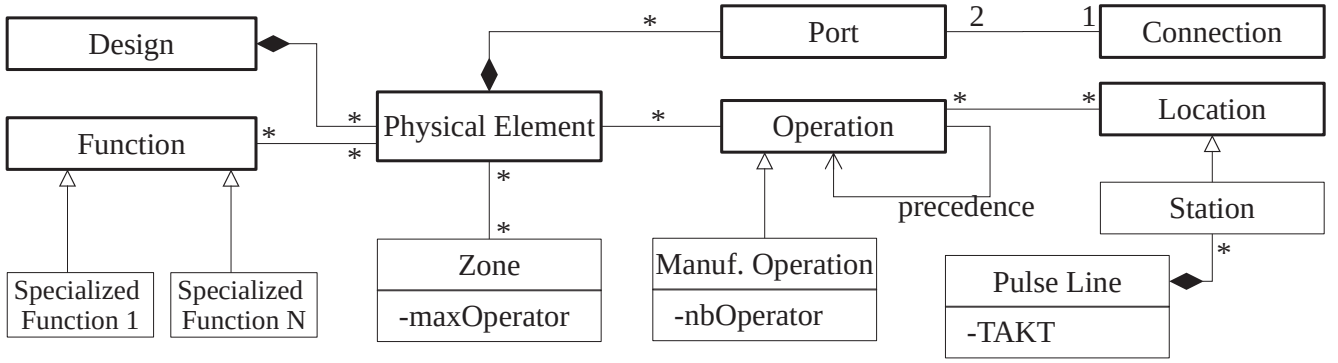
Fig. 1. Example: product and production class diagram.
