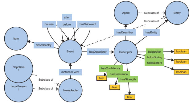
Fig. 3. Ontology for representing events, their event graphs, and their matching news angles.
