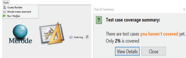
Fig. 2 Generation and Coverage of the application test cases.
