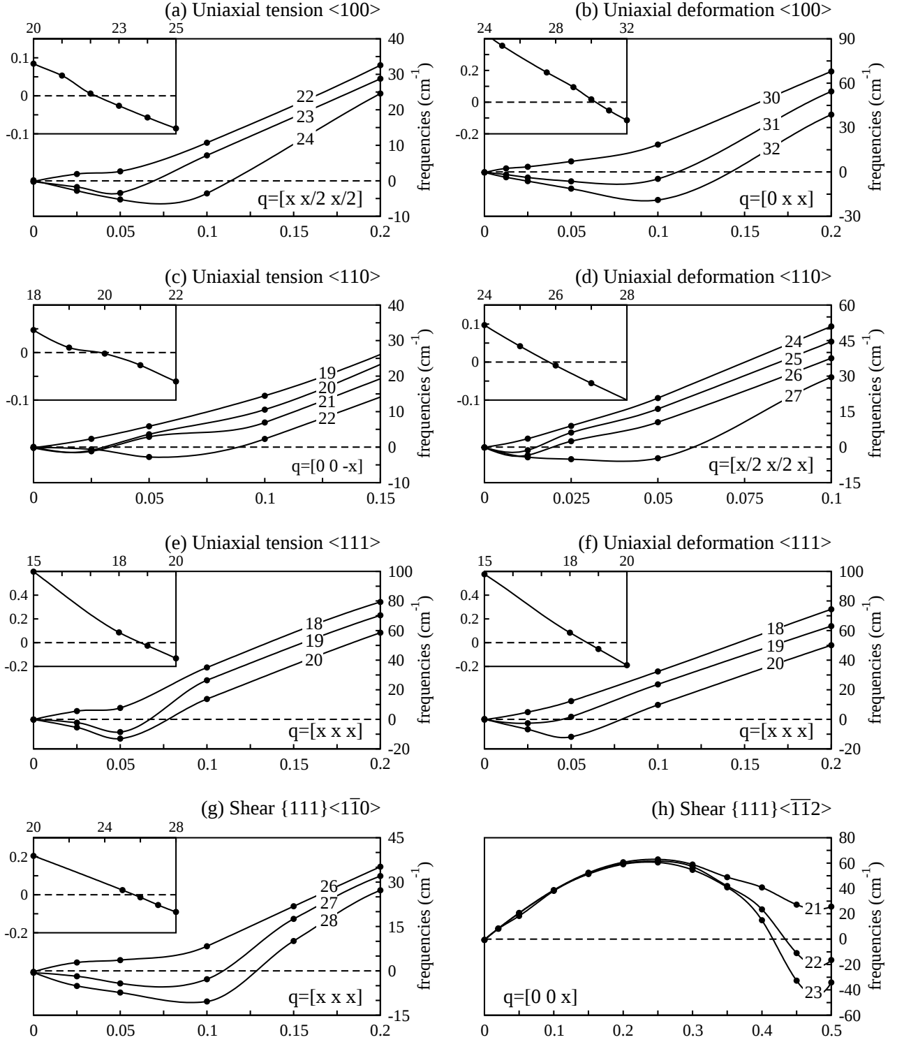
FIG. 3: Phonon energies along the direction of the first reported instability for various strains, for each of the investigated deformation conditions. The directions are indicated by their wavevector q given in reciprocal coordinates by multiples of the x -coordinate of the plot. The level of strain is indicated in % on the curve. The stiffness tensor eigenvalue (given in 100 GPa) corresponding to the phonon mode as a function of strain (in %) are reported in insets. Lines come from spline interpolation of the calculated results.
