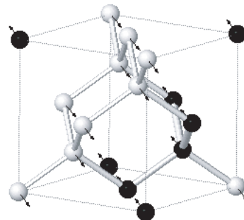
FIG. 4: Representation of the atomic displacements inducing the phase transition when a \{111\}\langle \bar{1}\bar{1}2 \rangle relaxed shear is applied to the silicon structure.
