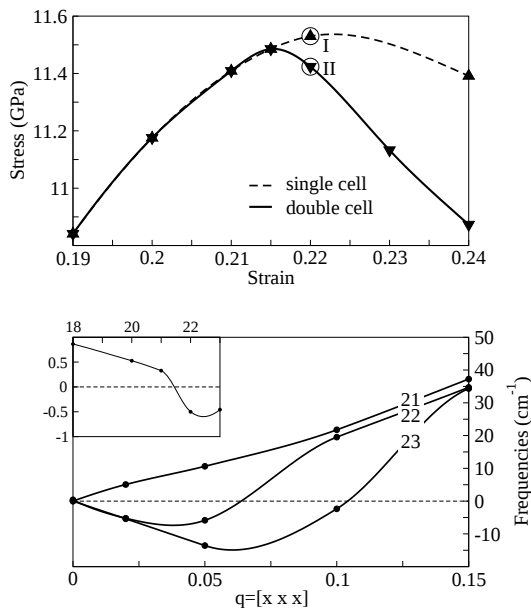
FIG. 5: (a) Comparison of the \{111\}\langle\bar{1}\bar{1}2\rangle relaxed shear loading path calculated with a single and a double unit cell. When working with the single cell (dashed curve), a phonon instability is detected (point I); while, with the double cell (solid curve), the first instability to occur (point II) is elastic. (b) Phonon energies calculated at point II along the direction of instability, as a function of strain (lines come from spline interpolation of the calculated results).
