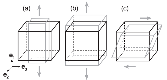
FIG. 1: Schematic representation of the loading conditions. (a) uniaxial tension [fully relaxed tension]; (b) uniaxial deformation [unrelaxed tension]; (c) relaxed shear.
