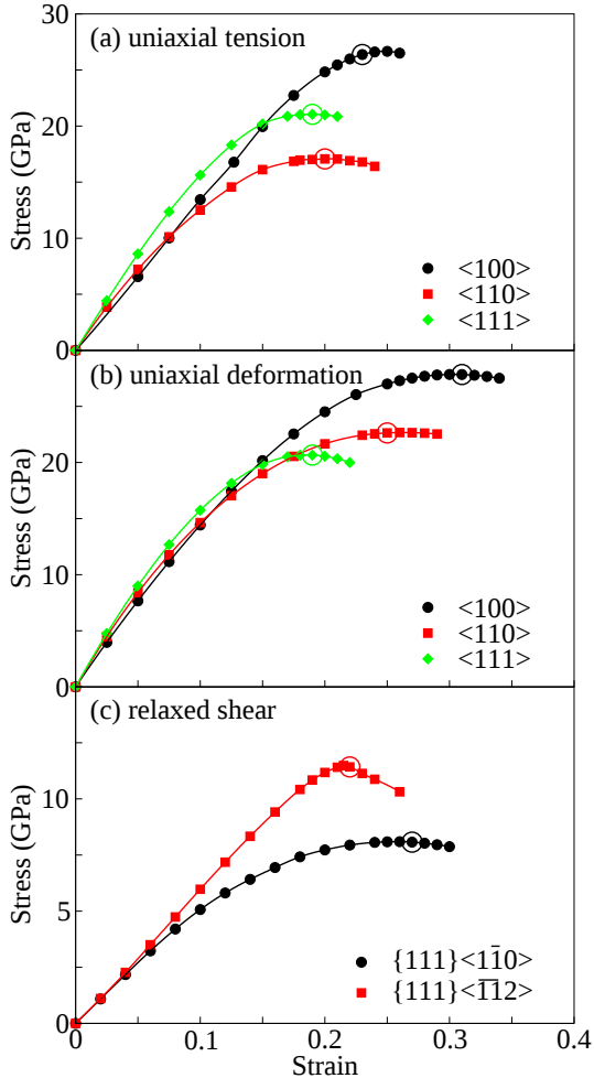
FIG. 2: (Color online) Stress strain relations for various loading paths (as indicated in insets). The open ring indicates the first appearance of an unstable phonon mode along each path.
