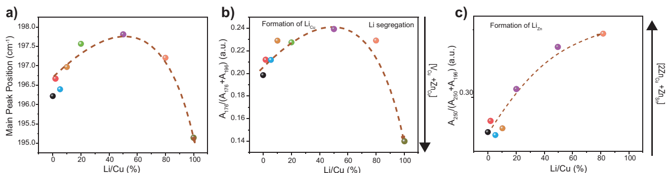
Figure 4. a) Plot of the ACZTSSe main peak position in Raman spectra as a function of Li content. b) Plot of the area ratio of the 176 cm -1 peak to the main peak. c) Plot of the area ratio of the 250 cm -1 peak to the main peak.
