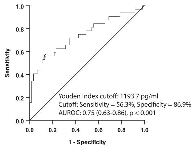
Fig. 2 Receiver-operating characteristic curve of serum GDF-15 concentrations for ≥F2 fibrosis (≥8.2 kPa as measured by VCTE). Sample size n = 93.
