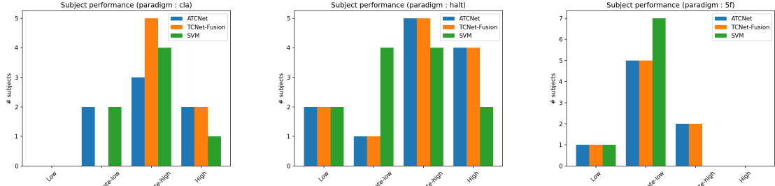
Figure 2: BCI control performance for respectively the CLA (left), HaLT (middle) and 5F (right) paradigms. BCI controls are defined as 4 equal groups ranging from chance level (defined as 1 / \text{number\_of\_labels} ) to 1, as explained in the main text.
