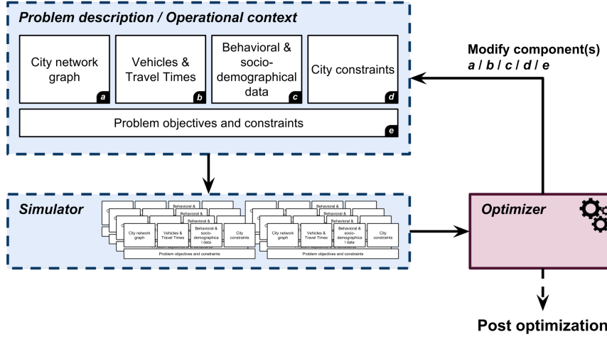
Figure B.1: The simulation-optimization framework.
