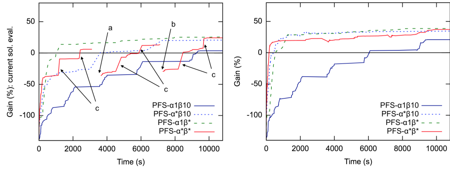
Figure 8.2: Evolution through time of the gain of the expected cost of the current solution with respect to the average cost of the w&s policy, during a single execution of four PFS instantiations for instance 50c-50w-1 (with K = 10 vehicles). Left: gain evaluated under \mathcal{R}^q at current scale \alpha . Right: gain evaluated under \mathcal{R}^{q+} at scale \alpha = 1 .
