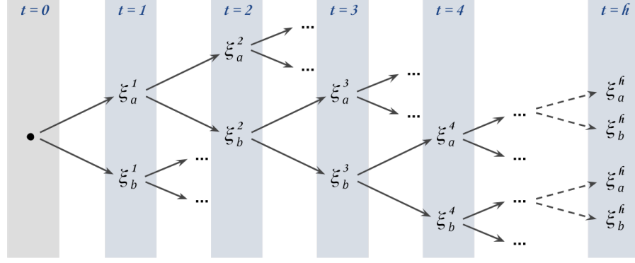
Figure 2.3: Tree structure of the problem. For simplicity, the random variable has only two possible outcomes (denoted a and b ) at each period, leading to 2^{h-t} leaf nodes. Each leaf node \zeta_i^h corresponds to a specific scenario.
