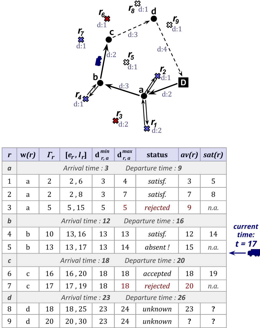
Figure 5.3: Example of second-stage solution at time t = 17 , under strategy \mathcal{R}^q . A filled cross represents a request that appeared, an empty one a request that is either still unknown (e.g., r_8 ) or revealed as being absent (i.e., did not appear, e.g., r_5 ). Here \pi_k = \langle r_a, r_1, \dots, r_9 \rangle is the sequence of requests assigned to the vehicle, according to (x, \tau) . We assume q_r = s_r = 0, \forall r \in R . sat(r) represents, for a request r , the time at which r gets satisfied. Function available(r) is here designated by av(r) for short.
