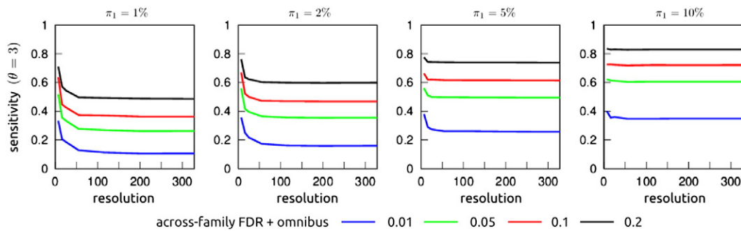
Fig. 4. Sensitivity on simulations with independent tests, K = 7 , L_k in (28,136,325,1540,6555,19900,53956), corresponding to the number of connections associated with the resolutions selected by MSTEPS on the SCHIZO dataset. The sensitivity is plotted as a function of resolutions (number of brain parcels) at four tested (within-resolution) FDR levels: 0.01, 0.05, 0.1, 0.2. For each resolution, the sensitivity was evaluated for tests at a single parcellation with the specified number of parcels. A test is only considered as significant if in addition an omnibus test against the global null hypothesis across resolutions as been rejected at p < 0.05 . Each column corresponds to a certain proportion of non-null hypothesis per resolution \pi_1 with an effect size \theta = 3 .
