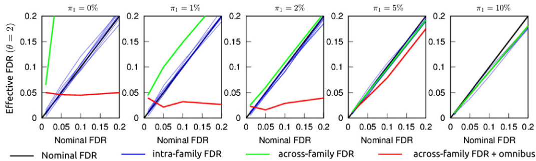
Fig. 3. Nominal vs effective FDR on simulations with independent tests ( K = 7 , L_k in {28,136,325,1540,6555,19900,53956}), corresponding to the MSTEPs resolutions in the SCHIZO dataset). The effective FDR within resolution (blue), across resolutions (green) and across resolutions with omnibus (red) is plotted against the nominal FDR (black), for four levels: 0.01, 0.05, 0.1, 0.2. Plots are presented for different proportions of non-null hypothesis per resolution \pi_1 (0 %, 1 %, 2 %, 5 %, 10 %), and an effect size \theta = 2 . For large \theta and/or \pi_1 , the omnibus test is always rejected, and the green plot matches perfectly the red plot, which becomes invisible.
