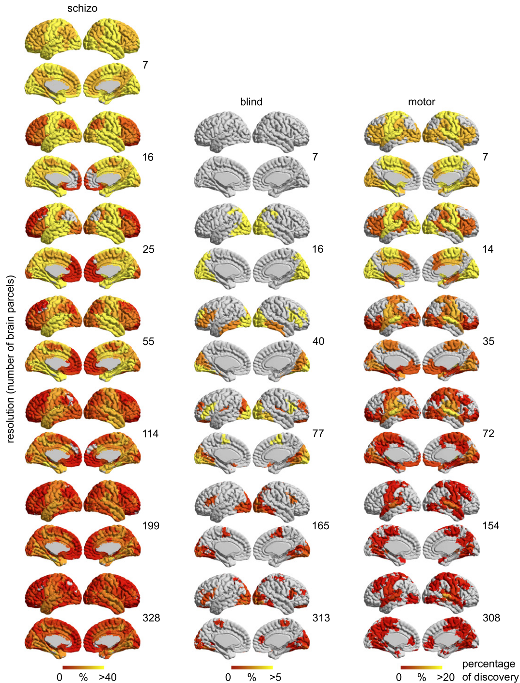
Fig. 9. Percentage of discovery maps in the three real datasets for all MSTEPs resolutions. Surface maps show the percentage of connections with a significant effect, for each brain parcel, in respectively the SCHIZO, BLIND and MOTOR contrasts. Maps are projected onto the MNI 2009 surface. See Fig. 8 for volumetric representations showing results at the subcortical level in the SCHIZO contrast.
