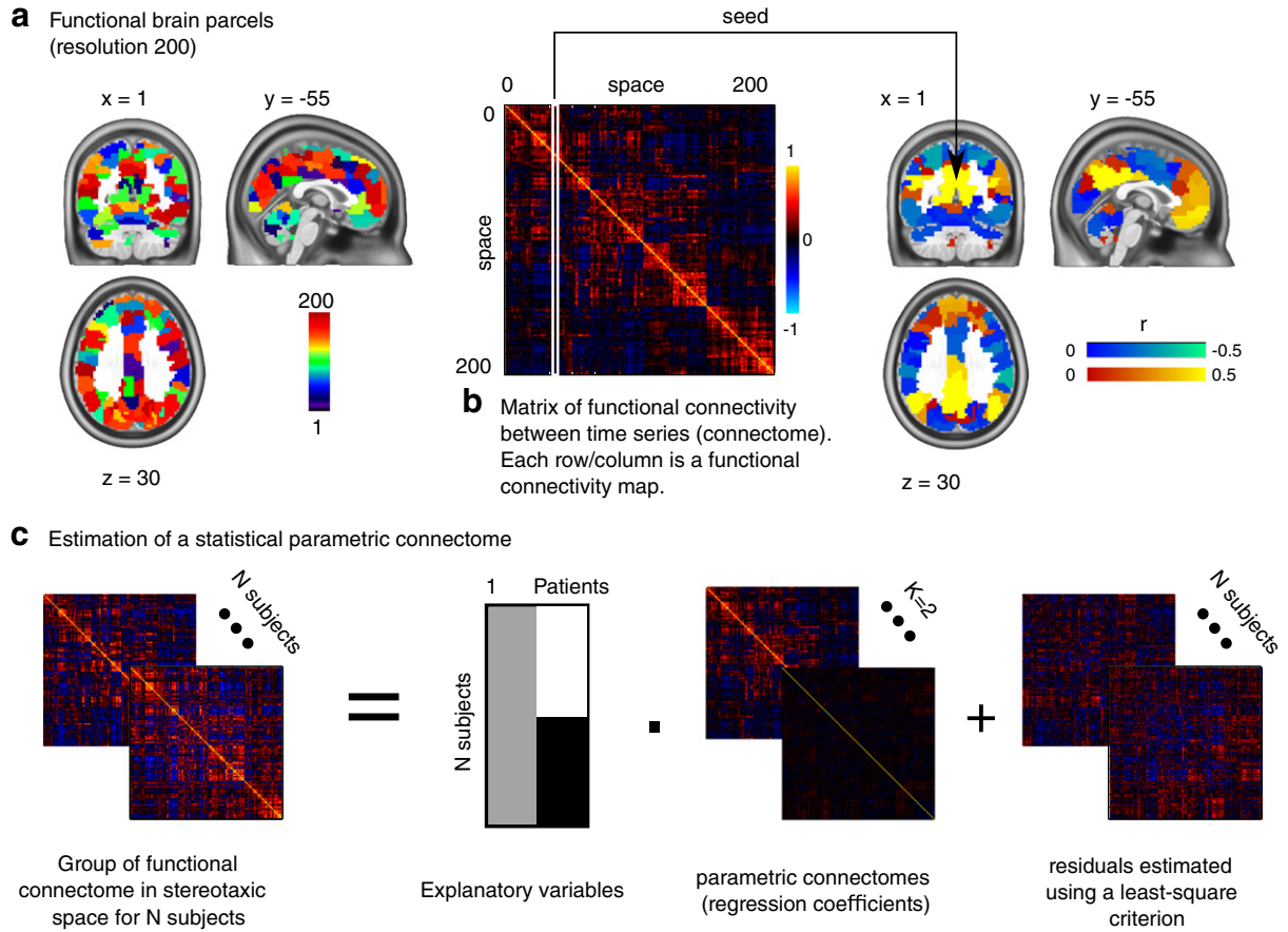
Fig. 1. General linear model applied to connectomes. The connectivity is measured between R brain parcels generated through a clustering algorithm (panel a). The connectome is a R \times R matrix measuring functional connectivity between- and within-parcels (panel b). The association between phenotypes and connectomes is tested independently at each connection using a general linear model at the group level (panel c). The results presented here are for illustration purpose only, and not related to the results presented in the application sections of the manuscript.
