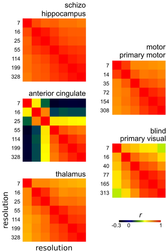
Fig. 11. Correspondence of effects maps across resolutions for the three real datasets. Correlation matrices show pairwise comparisons between 7 and 6 MSTEPs resolutions of the effects maps for three selected seeds in the SCHIZO dataset and one a priori seed in each of the BLIND and MOTOR dataset.
