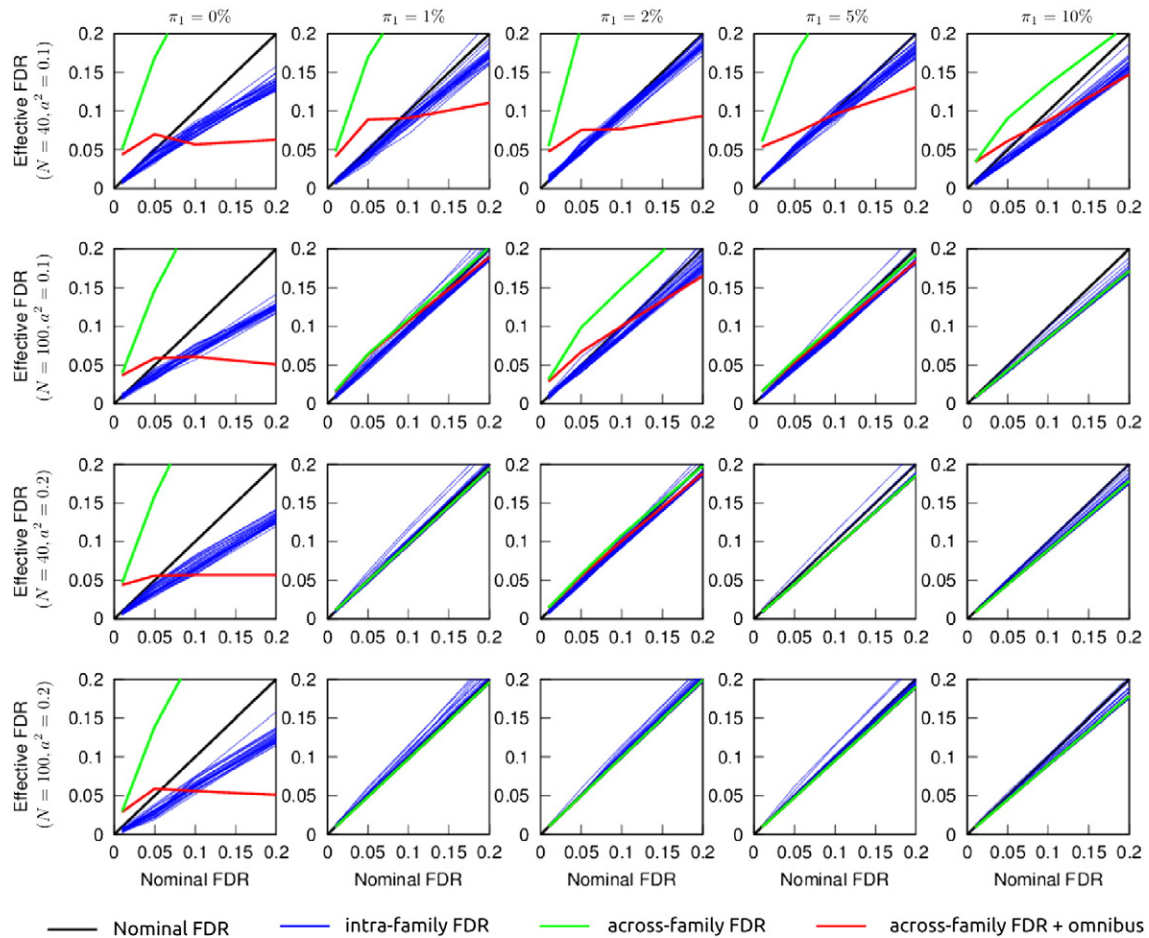
Fig. 5. Nominal vs effective FDR on simulations with dependent tests ( K = 30 , L_k ranging from 55 to 45150, corresponding to the number of connections associated with a regular grid of resolutions covering 10 to 300 with a step of 10). The effective FDR is plotted against the nominal FDR within each resolution (blue plots), across all resolutions (green plots) and across all resolutions, combined with an omnibus test for rejection of the global null hypothesis (red plot). The expected (nominal) values are represented in black plots, corresponding to the four tested FDR levels: 0.01, 0.05, 0.1, 0.2. Each column corresponds to a certain proportion of non-null hypothesis per resolution \pi_1 (0%, 1%, 2%, 5%, 10%), and each row corresponds to a different combination of effect and sample size N in {40, 100}, a^2 in {0.1, 0.2}, see text for details. Please note that in the presence of strong signal (large \theta and/or \pi_1 ), the omnibus test is always rejected, and the green plot matches perfectly the red plot, which becomes invisible.
