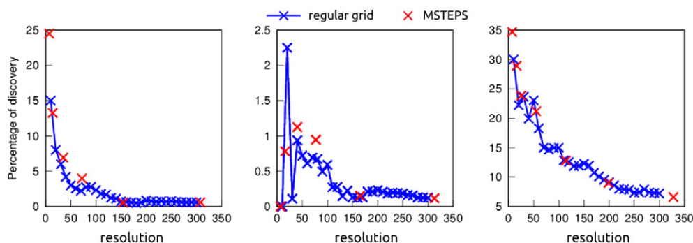
Fig. 7. Percentages of discovery as a function of resolutions (number of brain parcels). Plots show the percentage of discovery for the MOTOR, BLIND and SCHIZO contrasts. For each resolution, the percentage of discovery was evaluated for tests at a single parcellation with the specified number of parcels. The blue curve represents the resolutions selected on a regular grid, from 10 to 300 with a step of 10, and the red crosses show the resolutions selected by the MSTEPS procedure (see text for details).
