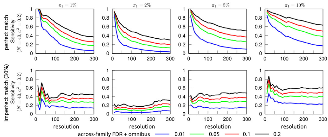
Fig. 6. Sensitivity on simulations with dependent tests ( K = 30 , L_k ranging from 55 to 45150, corresponding to the number of connections associated with a regular grid of resolutions covering 10 to 300 with a step of 10). The sensitivity is represented as a function of resolution, for four FDR levels: 0.01, 0.05, 0.1, 0.2, with either no mismatch or a 30% mismatch between the true and test clusters. For each resolution, the sensitivity was evaluated for tests at a single parcellation with the specified number of parcels. In addition to FDR control within resolution, an omnibus test at p < 0.05 was performed. Each column corresponds to a certain proportion of non-null hypothesis per resolution \pi_1 (0 %, 1 %, 2 %, 5 %, 10 %), with a sample size N = 40 and \alpha^2 = 0.2 .
