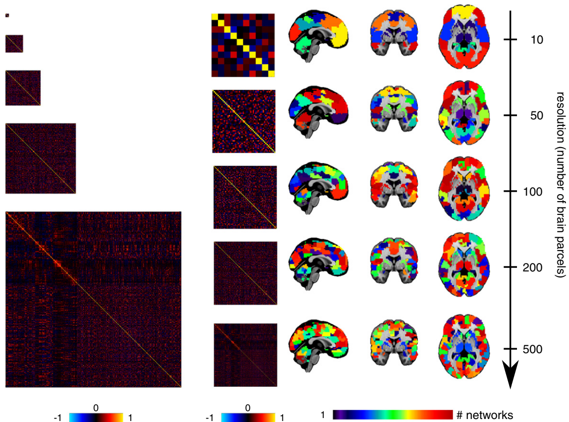
Fig. 2. General linear model applied to connectomes at multiple spatial resolutions. The generation of data-driven brain parcels is iterated at different resolutions (number of brain parcels), using the bootstrap analysis of stable clustered (BASC), with a hierarchical clustering using Ward's criterion. The statistical parametric connectomes are represented using both their real size (left column) and after rescaling to fit identical size (middle column) to illustrate the quadratic increase in the number of connections (multiple comparisons) that comes with an increase in the number of parcels. The results presented here are for illustration purpose only, and not related to the results presented in the application sections of the manuscript.
