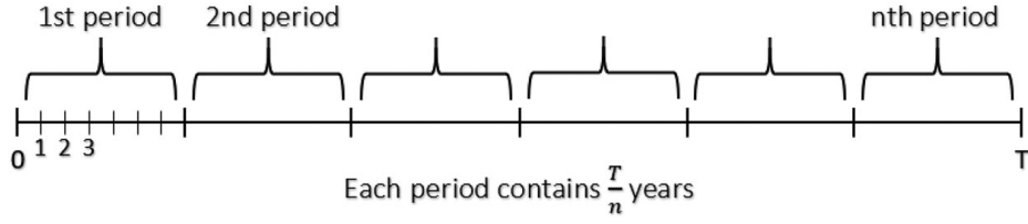
Figure 1. Representation of a \frac{T}{n} -years product.
