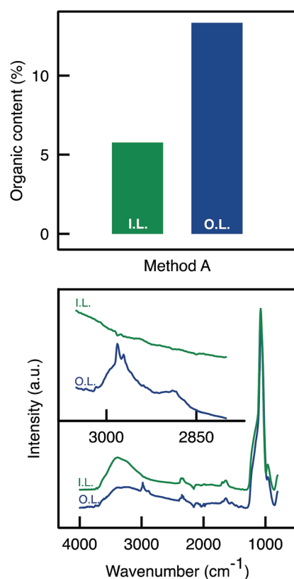
Fig. 3 (Top) Total organic content determined by TGA analyses on the outer and inner parts of the A50 A monolith. (Bottom) C–H stretching band absorbance was detected around 2900\text{ cm}^{-1} only for the outer layer of the sample A50 A .
