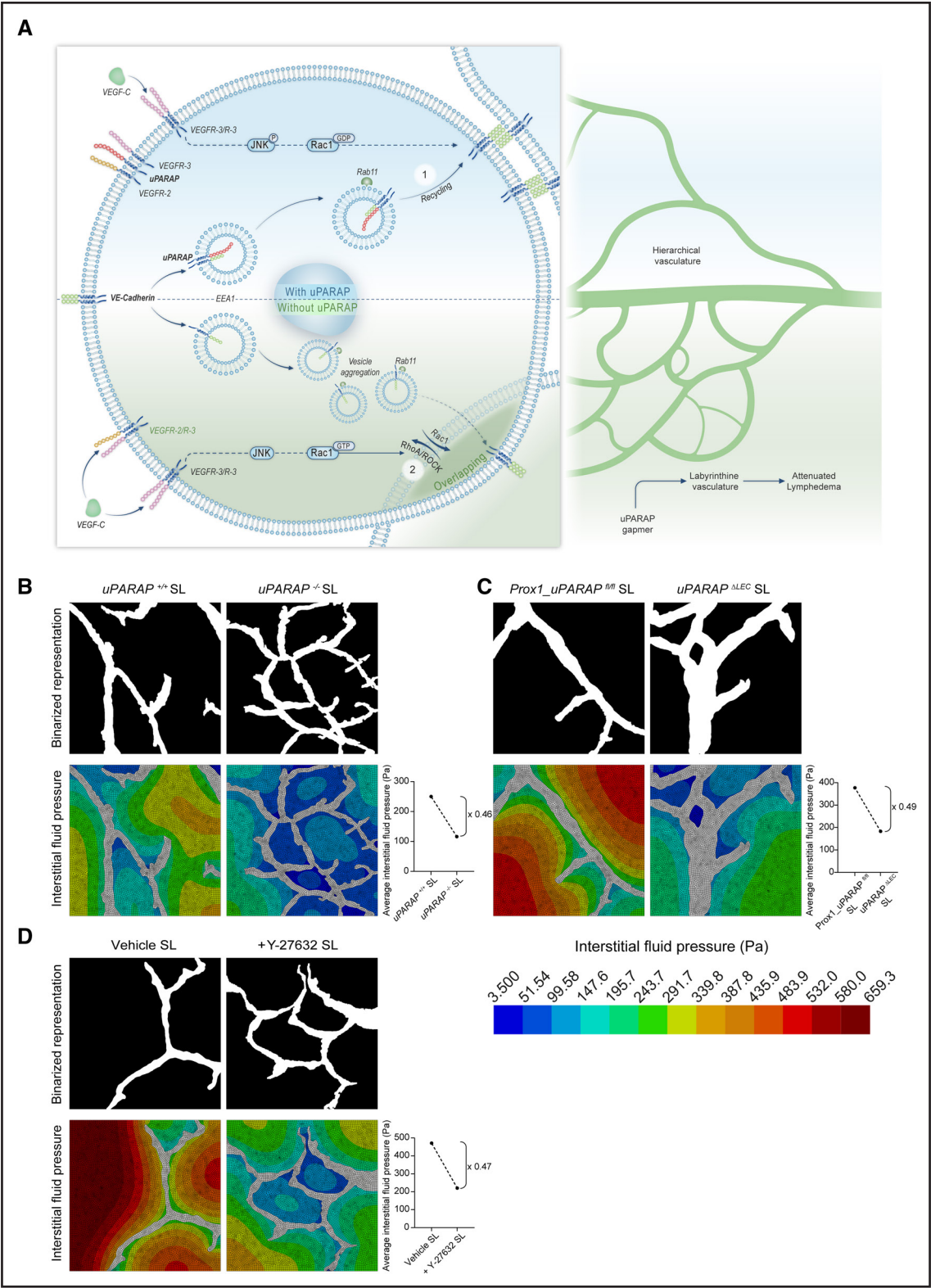
Figure 7. In silico simulation of fluid absorption in different topologies of the lymphatic vasculature. A , Schematic representation of the proposed model of labyrinthine vasculature. The reestablishment of lymphatic endothelial cell (LEC)–LEC junctions upon vascular endothelial growth factor–C (VEGF–C) stimulation relies on the correct endosomal trafficking of VE–cadherin and small GTPase activities (Rac1 [Ras–related C3–rich protein 1] for the formation of protrusions and ROCK [rho–associated coiled coil containing kinase]/RhoA (Ras homolog family member A) for their retraction). (Top) uPARAP (urokinase plasminogen activator receptor–associated protein) binds to VE–cadherin in early endosomes (EEA1) and drives it to Rab11 + recycling endosomes for its return to the cell surface. uPARAP also reduces VEGFR–2/VEGFR–3 heterodimerization, leading to increased Rac1 activity (Rac1–GTP). 16 In the presence of uPARAP, appropriate (Continued)
