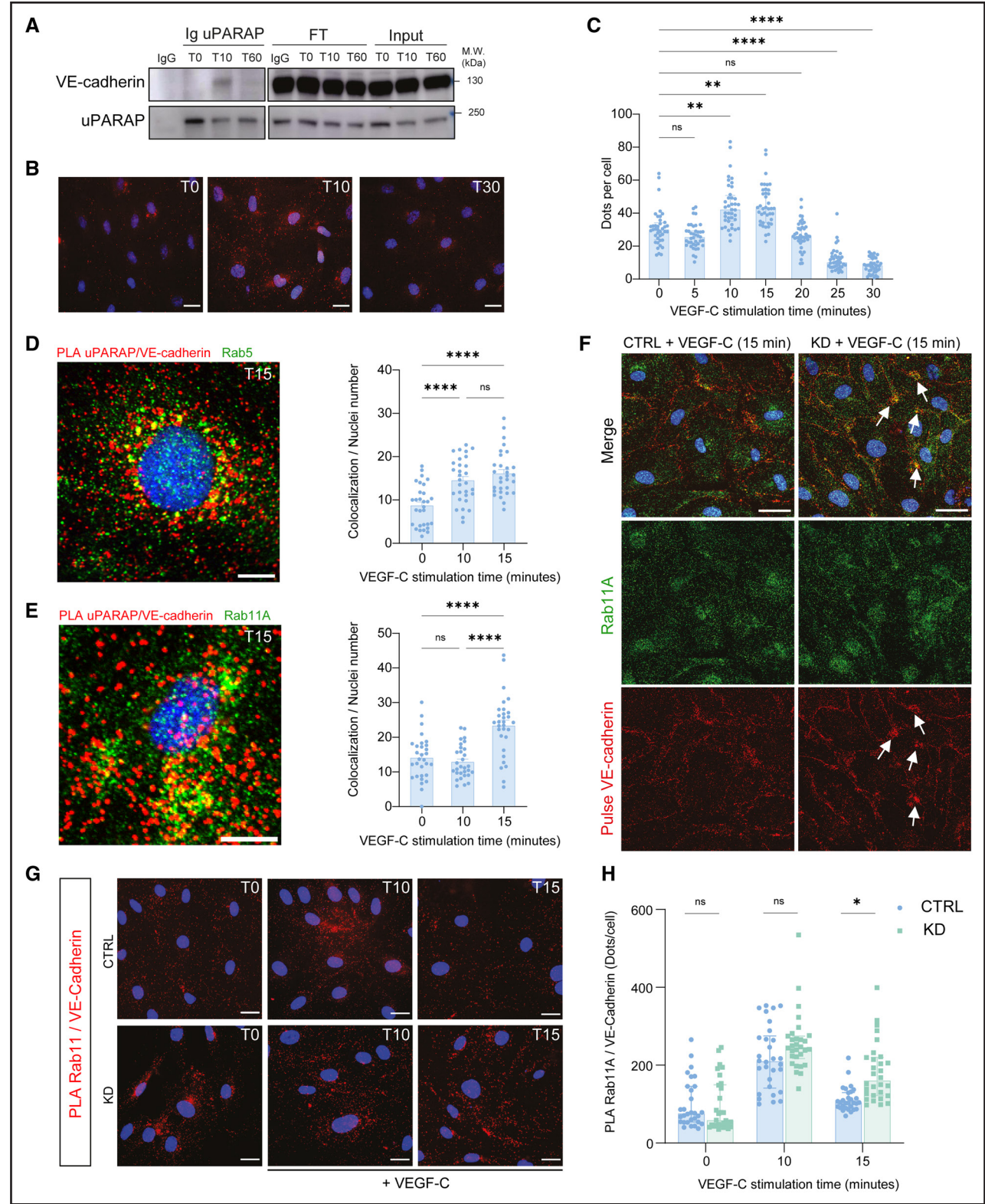
Figure 5. uPARAP interacts with vascular endothelial cadherin during its intracellular trafficking. A , Immunoprecipitation of uPARAP (urokinase plasminogen activator receptor-associated protein) from lymphatic endothelial cells (LECs) stimulated with vascular endothelial growth factor–C (VEGF–C) for 0, 10, or 60 minutes (T0 to T60). Vascular endothelial (VE) cadherin and uPARAP protein levels were revealed by Western blot in immunoprecipitates, flowthrough (FT), and input samples. Control immunoprecipitation was performed with a mouse control antibody (immunoglobulin G). B , uPARAP/VE–cadherin complex was determined by proximity ligation assay (PLA) in LECs treated with VEGF–C during the indicated time (T, in minutes). C , Positive red dots of PLA VE–cadherin/uPARAP were quantified and normalized by nuclei count. Data are medians with interquartile ranges of 40 independent microscope fields by condition from 2 independent experiments. D and E , Representative images (left, at 15 minutes of VEGF–C stimulation) of Rab5 ( D ) or (Continued)
