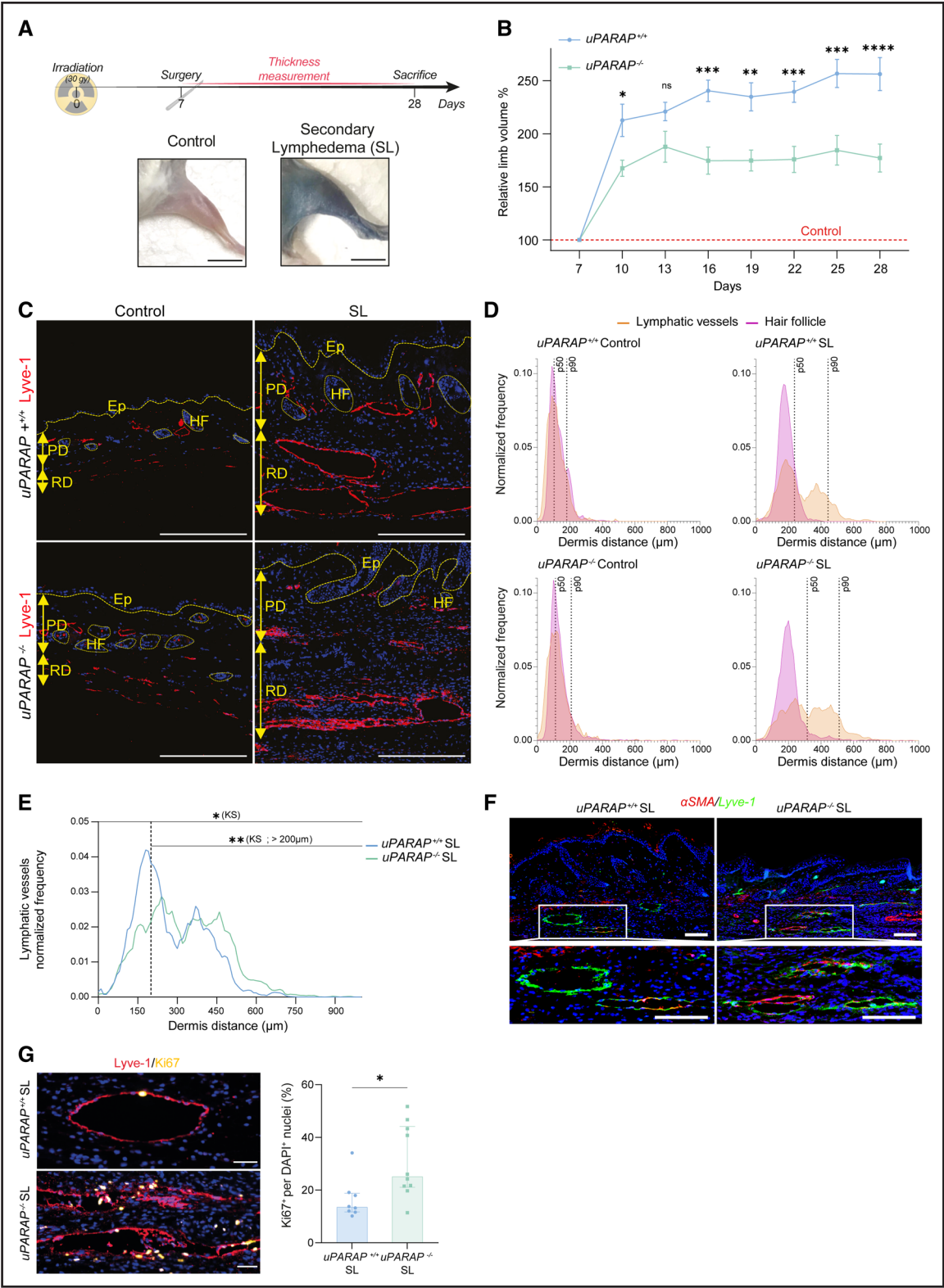
Figure 1. uparap deficiency attenuates secondary lymphedema. Secondary lymphedema (SL) was induced in WT ( uPARAP +/+ ) (n=8) and uparap -deficient ( uPARAP -/- ) (n=10) mice. A , Timeline of the experiment with representative images of control and SL limb at day 28. Scale bars=1 cm. B , Follow-up of the relative volume of hindlimb subjected to SL induction in uPARAP +/+ or uPARAP -/- mice. Results are expressed as percentage of control limb volume (100%, dotted line). Data are mean±SEM. C , Representative images of Lyve-1 + vessels (red) with nuclei (blue) in control and SL skin. Scale bars=250 μm. D , Spatial distribution of lymphatic vessels (orange) as the distance from the basal epithelial layer (distance=0 on the x axis). Hair follicle density (purple) is presented to delineate hair follicle-associated lymphatic vessels in the papillary dermis. P50 and P90 percentiles correspond to the (Continued)
