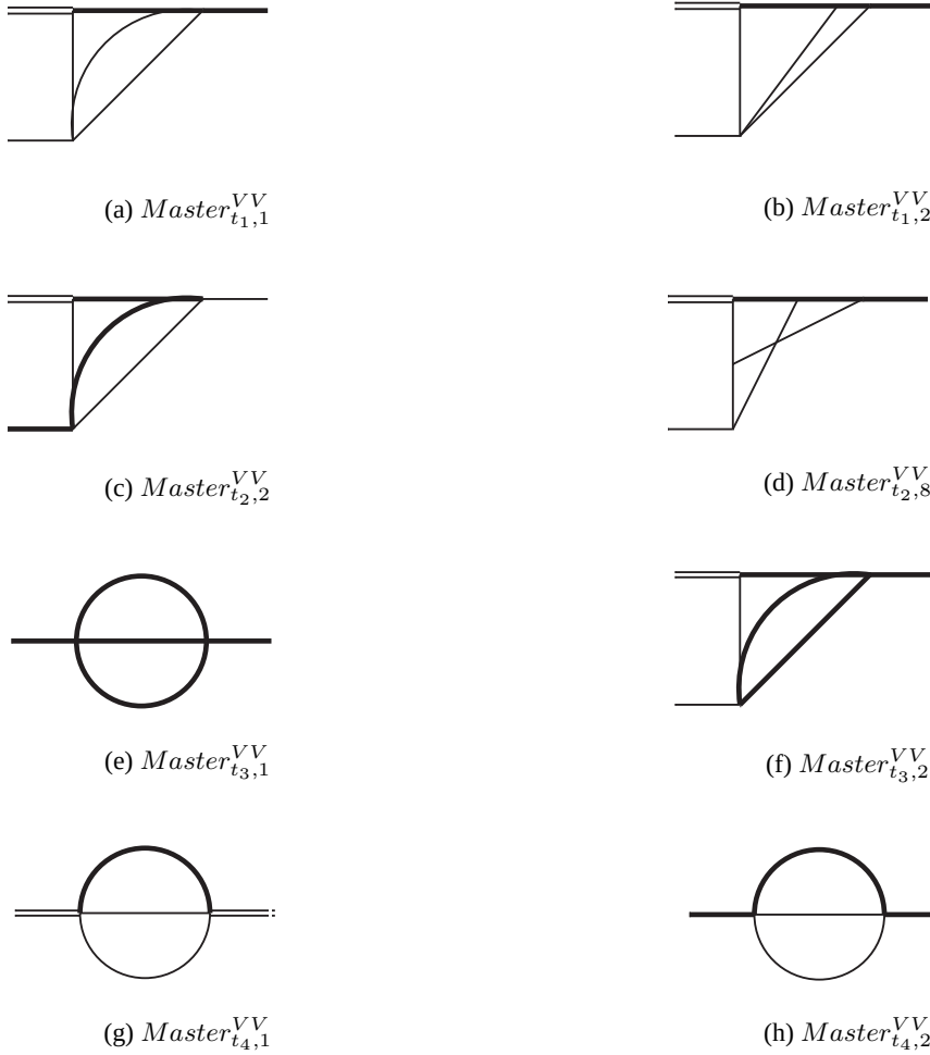
Figure 5.25: Set of independent subtopologies for b + W^* \rightarrow t at 2-loop.
