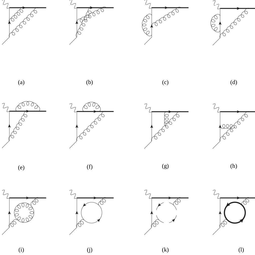
Figure 5.23: 2-loop corrections to b + W^* \rightarrow t
