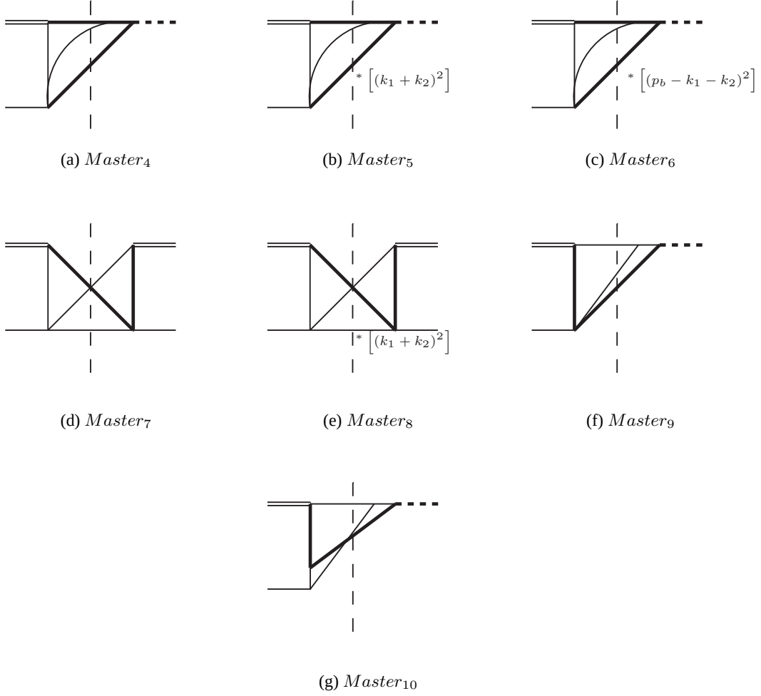
Figure 5.11: Set of independent MIs for b + W^* \rightarrow t + b + \bar{b} .
