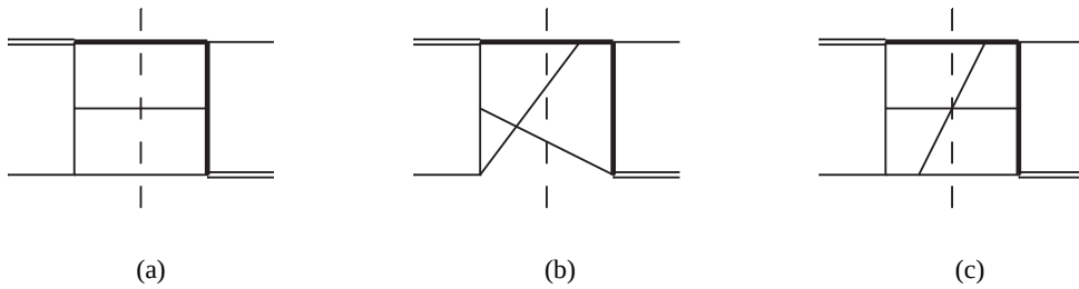
Figure 5.27: Independent topologies to g + W^* \rightarrow t + \bar{b} + g .
