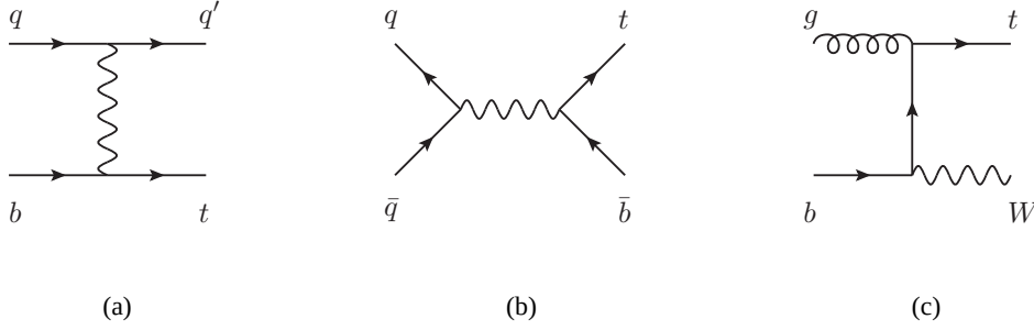
Figure 2.4: Tree-level Feynman diagrams for Single Top production.
