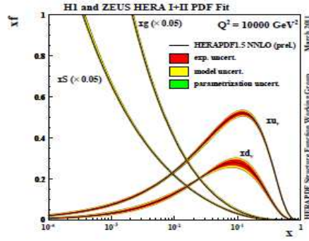
Figure 2.2: HERAPDF1.5NNLO PDF evaluated at \mu^2 = 10000 \text{ GeV} . The behaviour for \mu^2 = m_t^2 \sim 30000 \text{ GeV} is similar.
