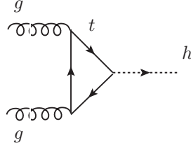
Figure 2.10: Higgs production via gluon fusion.
