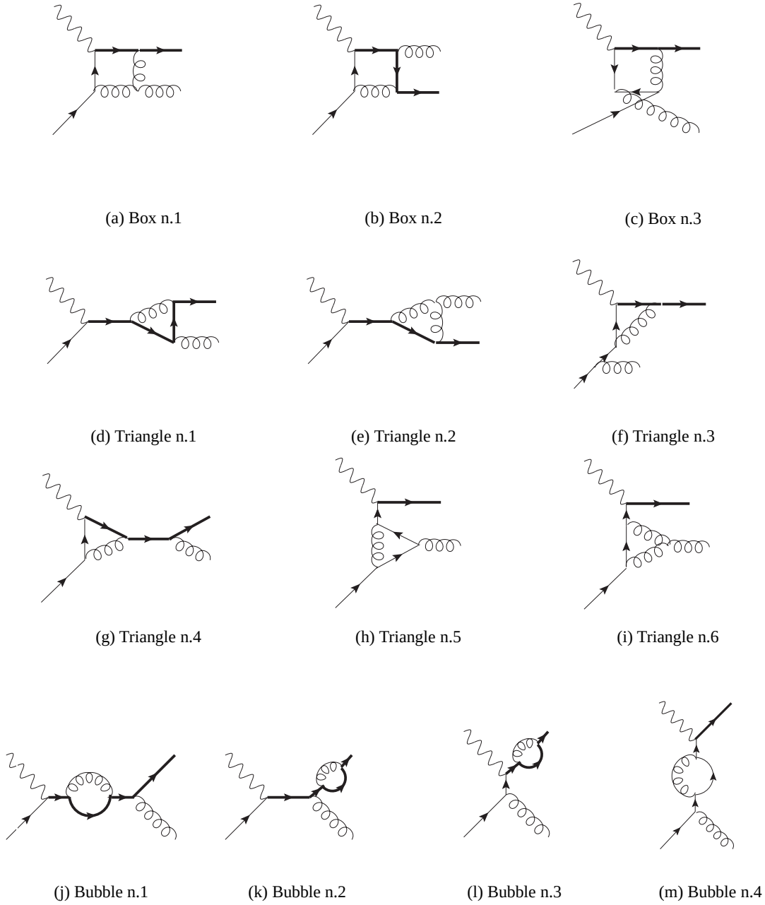
Figure 5.12: 1-loop corrections to b + W^* \rightarrow t + g
