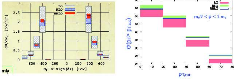
Figure 2.12: Left plot: Tevatron results for the invariant mass distribution M_{tt} for top quark pair production at NNLO accuracy. Right plot: NNLO cross-section for the production of single top quarks at the LHC 7 TeV, as a function of the cut of the p_T of the top quark.
