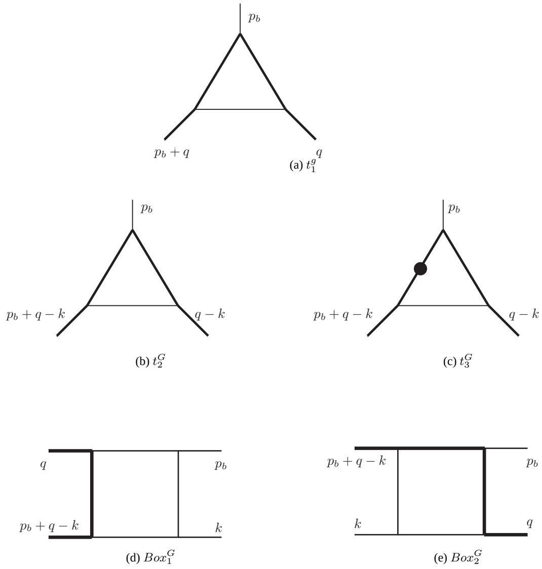
Figure 5.33: Independent 1-loop boundary conditions for the gluon RV Master Integrals (new with respect to the ones encountered in the bottom channel).
