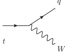
Figure 2.5: Top quark decay into quark and W boson.
