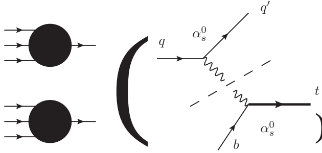
(a) Structure Functions contributions to Single top in t -channel at \mathcal{O}(\alpha_w^2) .
