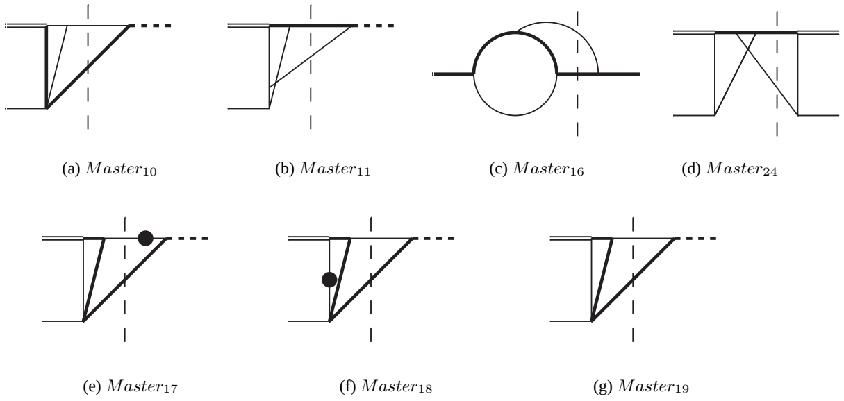
Figure 5.15: Set of independent MIs for b + W^* \rightarrow t + g at 1-loop ( Master from 10 to 24).
