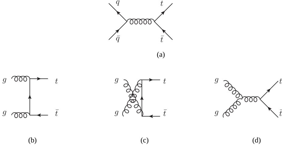
Figure 2.1: Tree-level diagrams for strong production of t\bar{t} pair.
