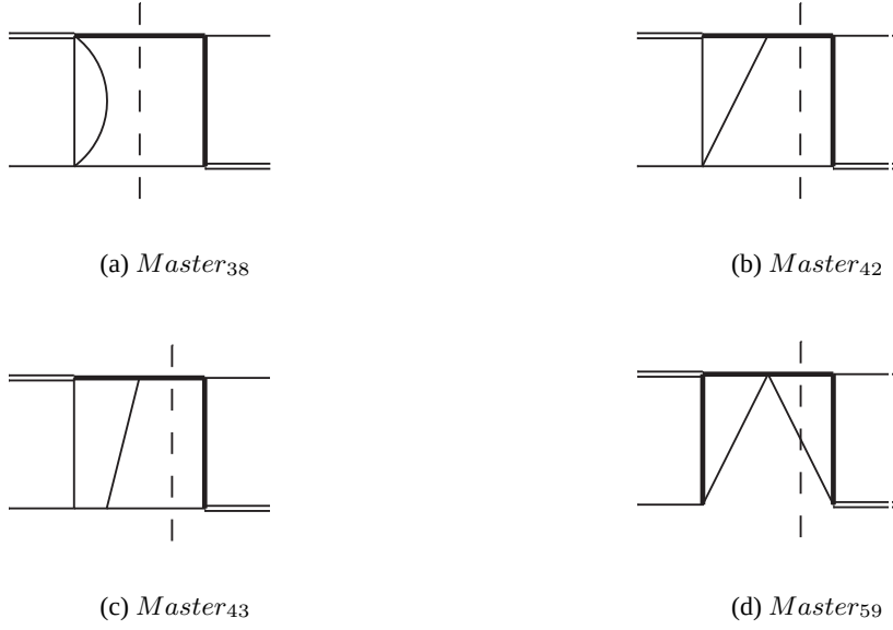
Figure 5.32: Set of new MIs appearing in g + W^* \rightarrow t + \bar{b} at 1-loop ( Master from 38 to 59). Simple thin lines are massless, simple thick lines, double lines and thick dashed lines are massive and correspond respectively to m_t^2 (either internal or external), Q^2 and s (only external).
