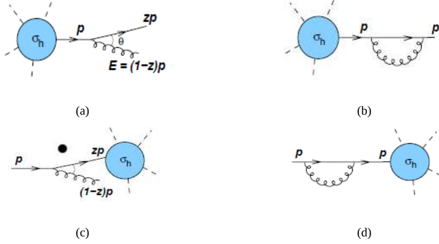
Figure 3.2: Single real and virtual QCD radiation from the initial and final state of a generic process h .
