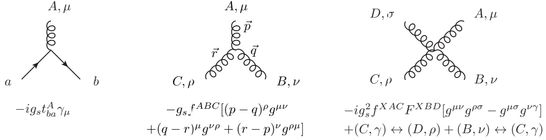
Figure 3.1: Feynman rules of QCD.
