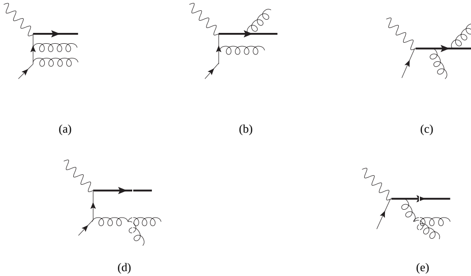
Figure 5.5: Tree-level diagrams for b + W^* \rightarrow t + g + g
