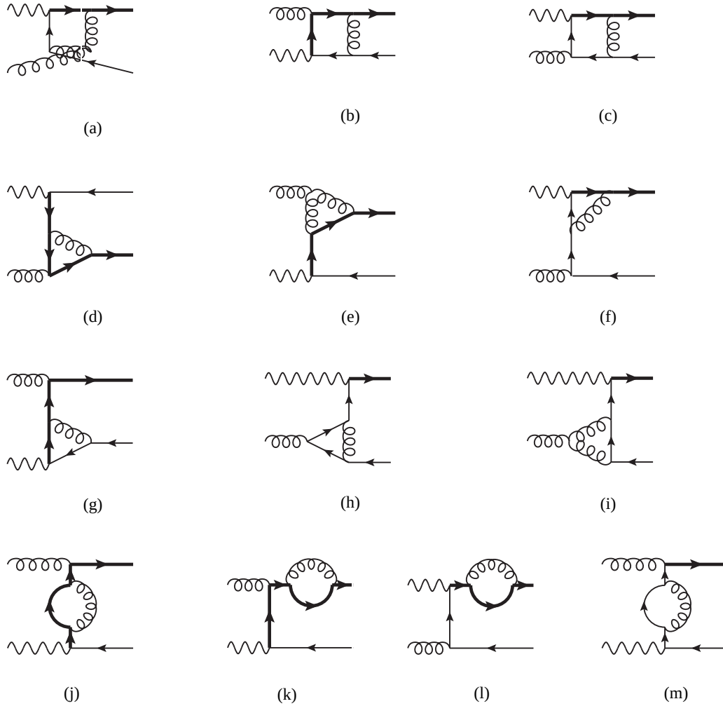
Figure 5.29: 1-loop corrections to g + W^* \rightarrow t + \bar{b}
