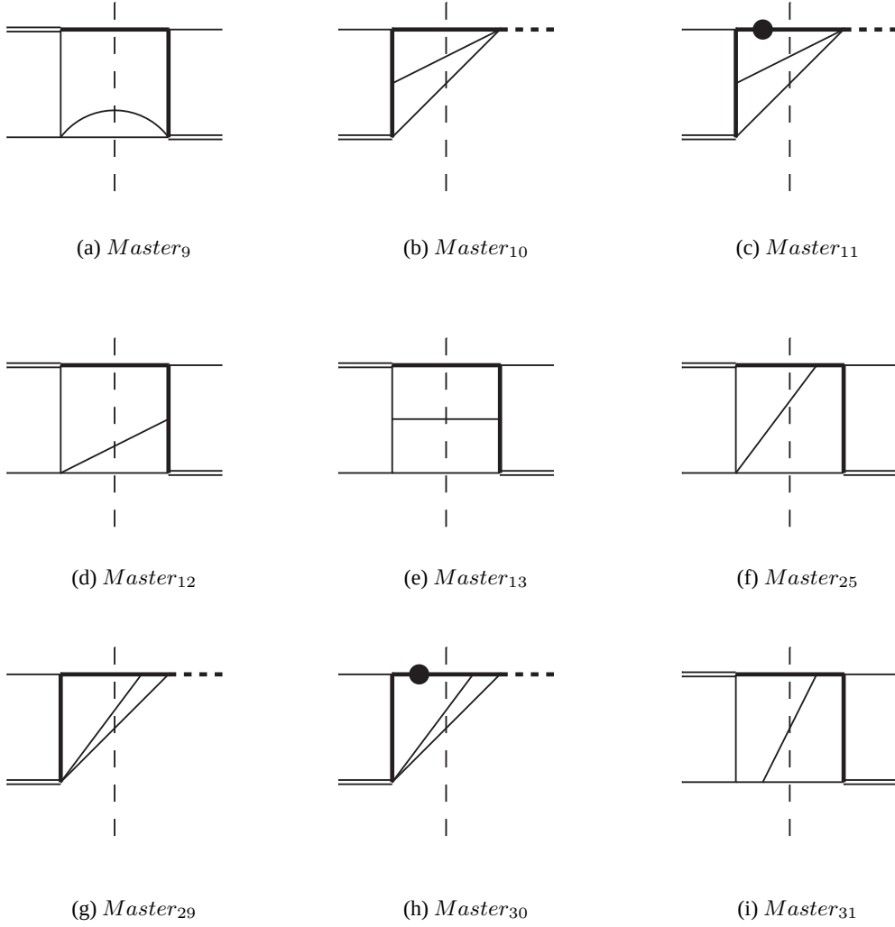
Figure 5.28: Set of new MIs appearing in g + W^* \rightarrow t + \bar{b} + g .
