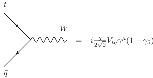
Figure 2.3: Top weak current.
