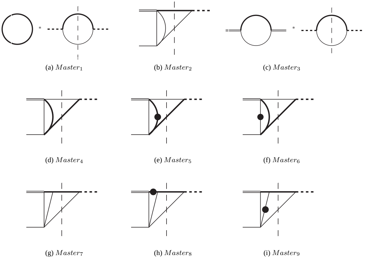
Figure 5.14: Set of independent MIs for b + W^* \rightarrow t + g at 1-loop ( Master from 1 to 9).
