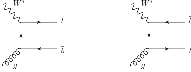
Figure 3.9: Leading-Order diagrams for Single Top production in t -channel in 4F-scheme.
