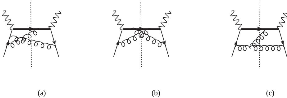
Figure 5.6: Phase-space diagrams for b + W^* \rightarrow t + g + g corresponding respectively to the independent topologies t_1, t_2, t_3 .
