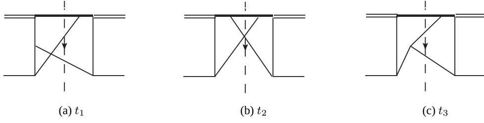
Figure 5.7: Independent topologies to b + W^* \rightarrow t + g + g .
