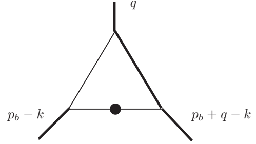
(b) Triangle n.3: t_3
