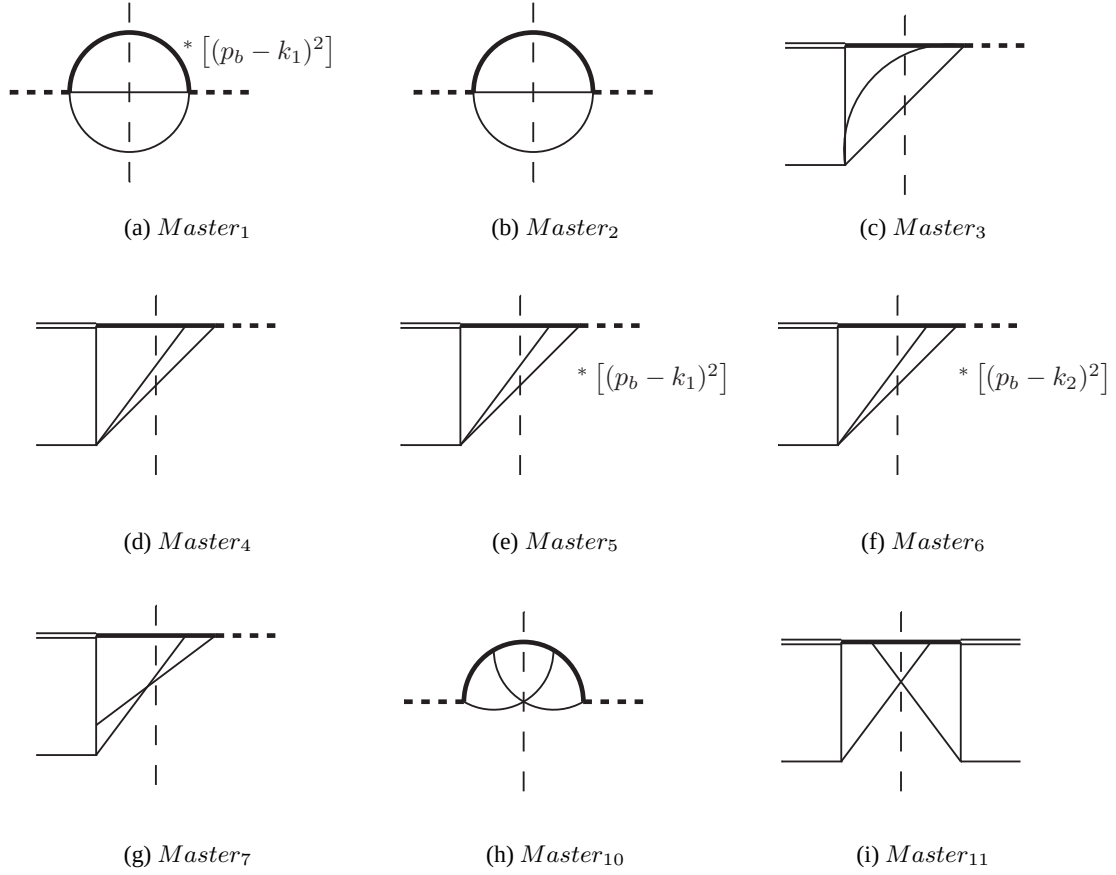
Figure 5.8: Set of independent MIs for b + W^* \rightarrow t + g + g .
