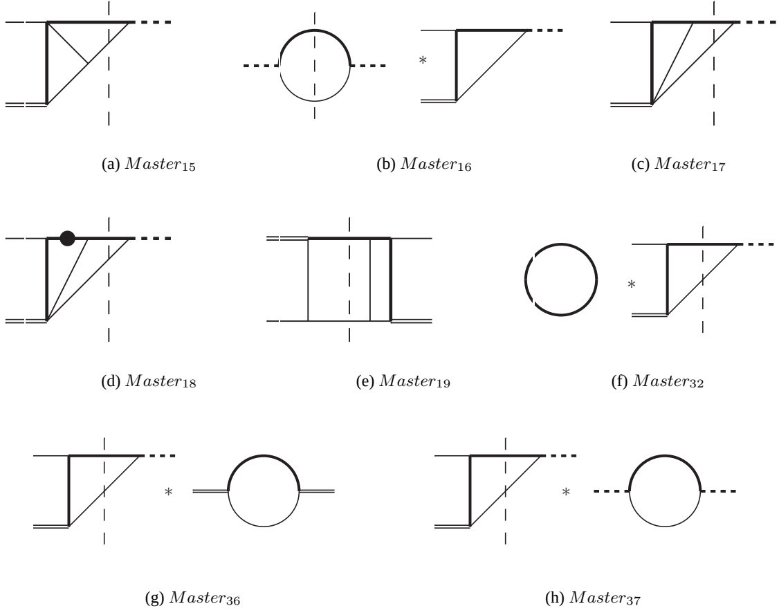
Figure 5.31: Set of new MIs appearing in g + W^* \rightarrow t + \bar{b} at 1-loop ( Master from 15 to 37).
