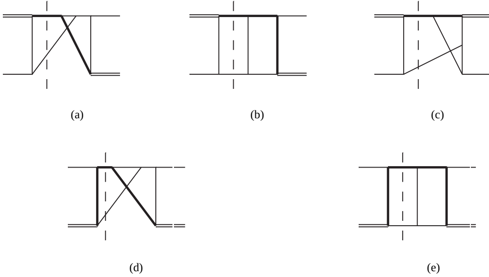
Figure 5.30: Independent topologies to [g + W^* \rightarrow t + \bar{b}]_{1-loop} .
