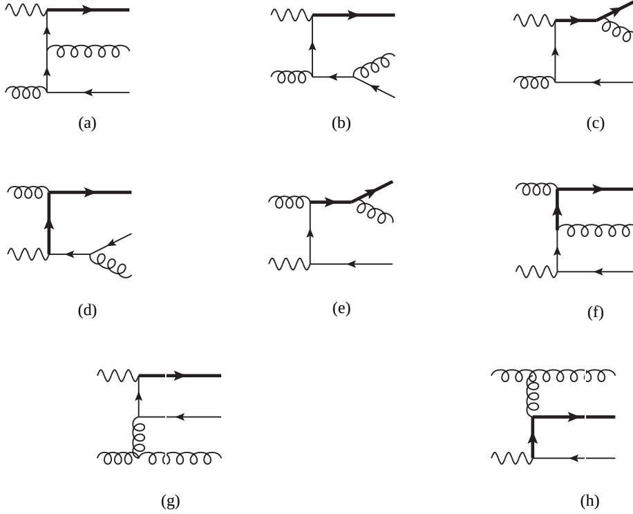
Figure 5.26: Tree-level diagrams for g + W^* \rightarrow t + \bar{b} + g
