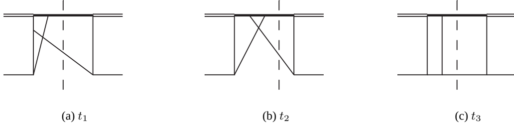
Figure 5.13: Independent topologies to [b + W^* \rightarrow t + g]_{1-loop} .
