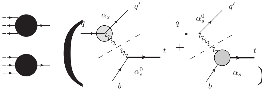
(b) Structure Functions contributions to Single top in t -channel at \mathcal{O}(\alpha_w^2 \alpha_s) .
