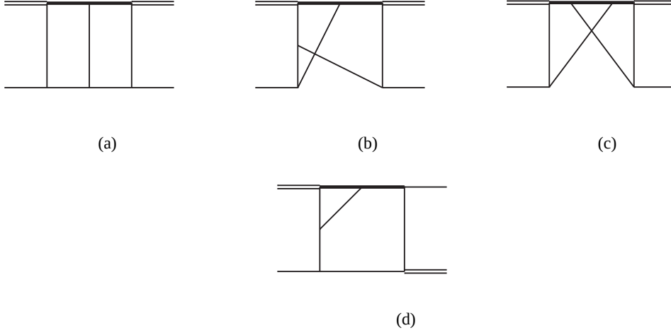
Figure 5.24: Independent topologies for [b + W^* \rightarrow t]_{2l} .
