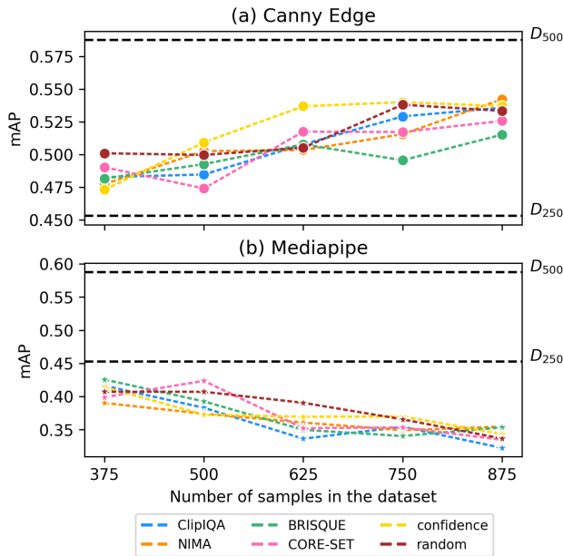
Fig. 5. Performance Evaluation of the trained YOLOv8 models on test set. Influence of sampling methods (ClipIQ, NIMA, BRISQUE, CORE-SET, confidence) on COCO dataset for ControlNet (a) Canny Edge (b) Mediapipe . "random" sampling refers to plots (a) and (b) of Fig.4 for which the synthetic images are selected randomly.
