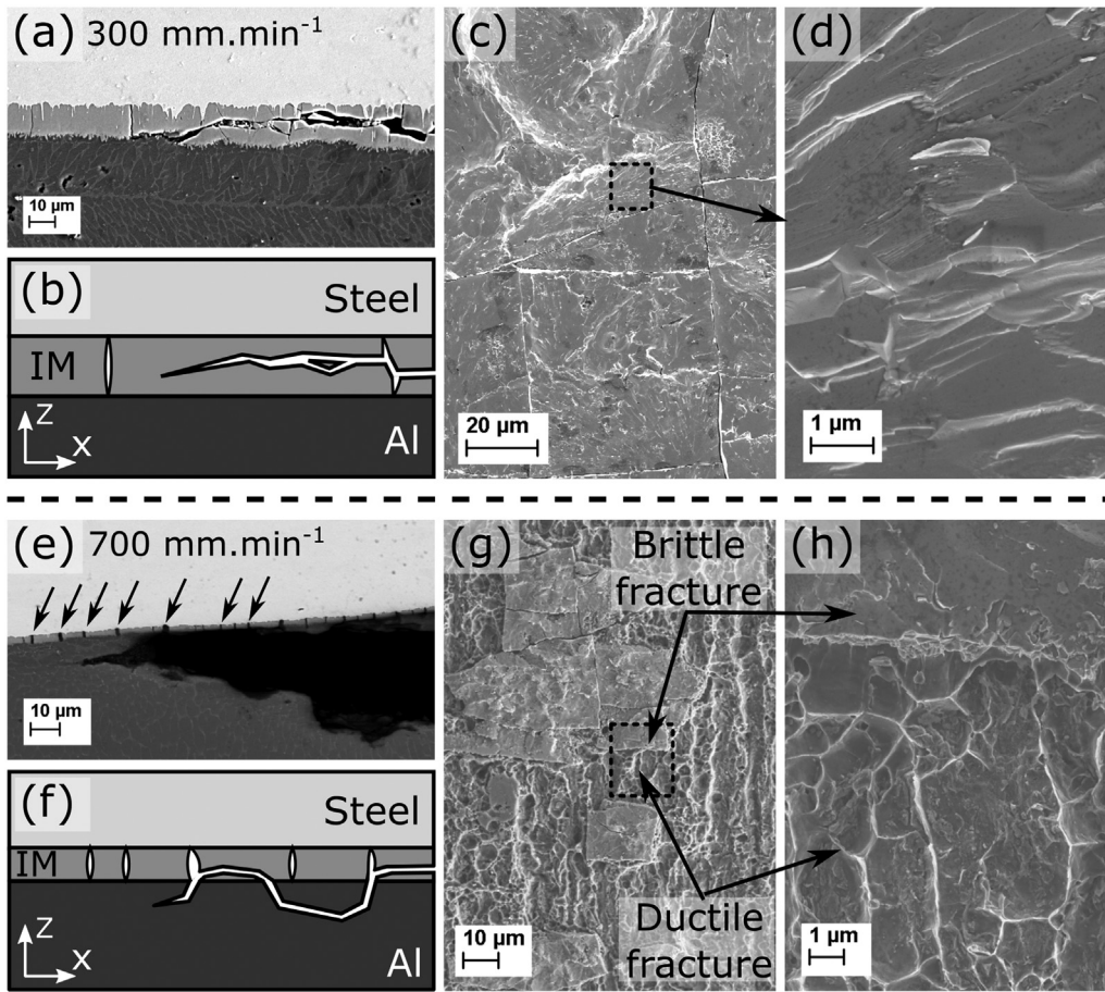
Fig. 10. Crack and surface observations for the Fe-Al system corresponding to a weld performed at (a, b, c and d) 300 mm min -1 and (e, f, g and h) 700 mm min -1 . (a and b) Longitudinal cross section and schematic representation of the crack propagation through the IM layer, respectively. (c and d) Surface observations of the fracture revealing a brittle fracture at low and high magnification respectively. (e and f) Longitudinal cross section and schematic representation of the alternating crack propagation through the Al plate and the IM layer, respectively. (g and h) Surface observations of the fracture surface revealing a ductile fracture at low and high magnification respectively.
