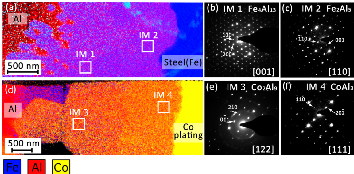
Fig. 4. (a and d) EDX elemental maps acquired on FIB samples of the Fe-Al and Co-Al systems, respectively. (b, c, e and f) are SAED patterns obtained on IM1, IM2, IM3 and IM4, respectively, with indicated zone axis corresponding to the identified phase.
