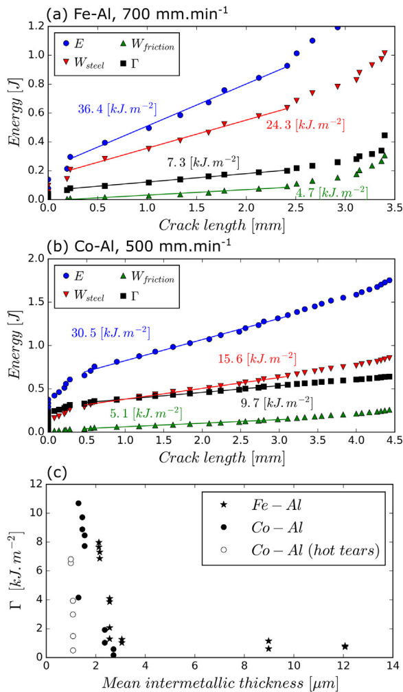
Fig. 9. Calculation of the critical energy release rate, \Gamma , on (a) a Fe-Al specimen welded at 700 mm min -1 and (b) a Co-Al specimen welded at 500 mm min -1 . Each point of the curve corresponds to a frame of the video recording. The continuous lines correspond to the linear fit. (c) Calculated critical energy release rates, \Gamma , for the Fe-Al and the Co-Al systems as a function of the mean IM layer thickness. The empty marks denote the presence of hot tears in the specimen.
