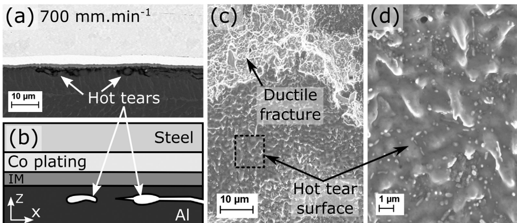
Fig. 12. Crack and surface observations for a weld with a Co interlayer at 700 mm min -1 . (a and b) Longitudinal cross section and schematic representation, respectively, of the crack propagation through the Al and the hot tear defects. (c) Surface observation of the fracture surface revealing a combination of hot tears and ductile fracture surfaces. (d) Observation at high magnification of the surface of a hot tear showing a solidification structure.
