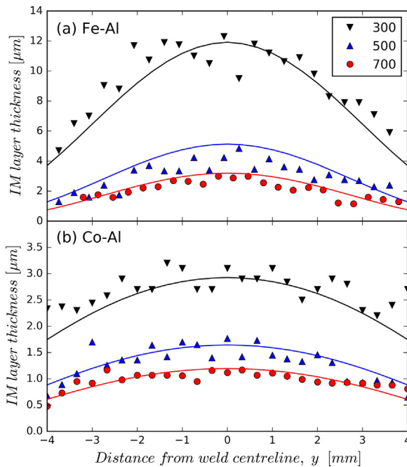
Fig. 5. Thickness of the IM layer in the (Y, Z) plane (defined in Fig. 1). The points represent the measured thickness from the SEM images. The continuous lines are drawn using Eqs. 2 and 3 with the fitted parameters given in Table 7 and the temperature field from the FE simulations. Results are provided for the welding systems, (a) Fe-Al, and (b) Co-Al, at three welding speeds (300, 500 and 700 mm min -1 ).
