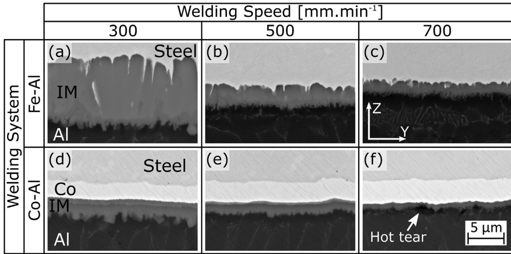
Fig. 3. Backscatter SEM micrographs of the intermetallic phases formed at the interface for the Fe-Al and Co-Al welding systems with welding speeds of 300, 500 and 700 mm min -1 , respectively.
