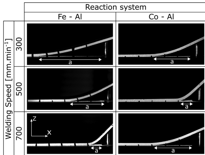
Fig. 6. Frames from the video recording of the crack propagation test at a constant rod displacement of 3 mm for the Fe-Al and Co-Al systems at three different welding speeds (300, 500 and 700 mm min -1 ). The horizontal black marks on the specimens are spaced of 5 mm starting from the tip of the notch.
