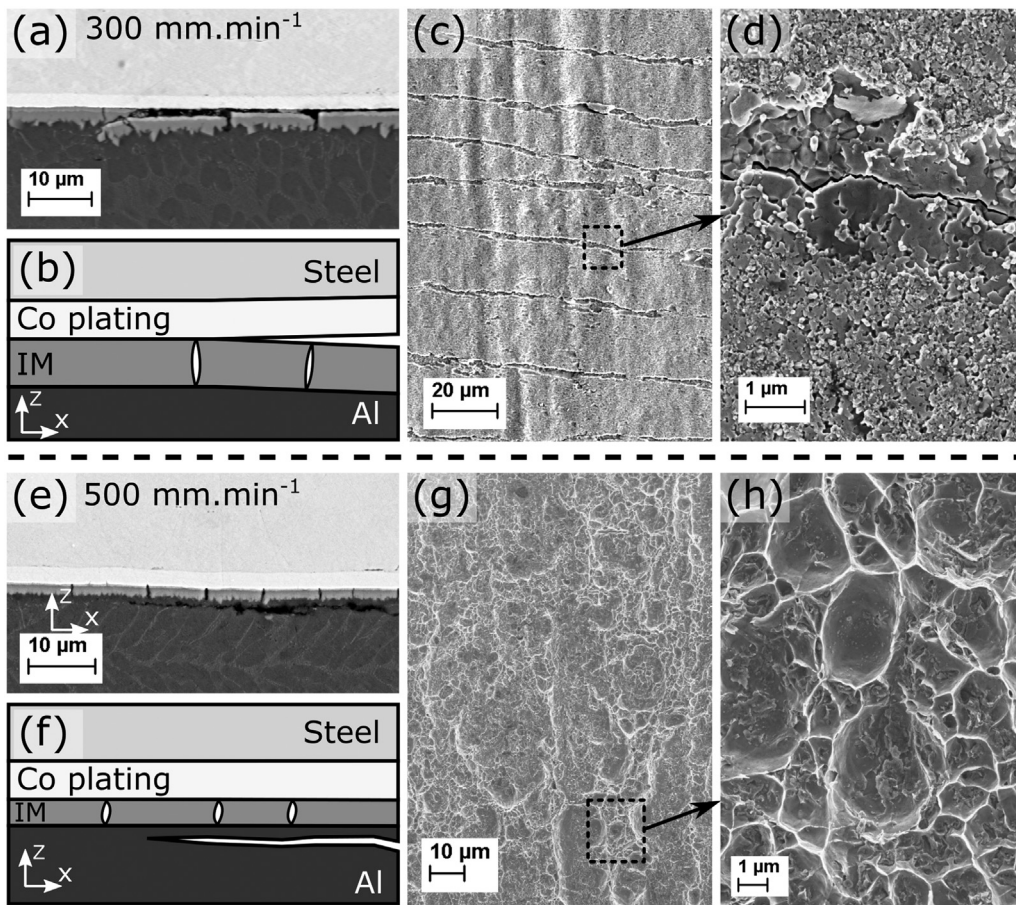
Fig. 11. Crack and surface observations for the Co-Al system corresponding to a weld performed at (a, b, c and d) 300 mm min -1 and (e, f, g and h) 500 mm min -1 . (a and b) Longitudinal cross section and schematic representation of the crack propagation through the IM-plating, respectively. (c and d) Surface observations of the fracture revealing the faceted Al 13 Co 4 grains on the Al side of the fracture. (e and f) Longitudinal cross section and schematic representation of the crack propagation through the Al, respectively. (g and h) Surface observations of the fracture surface revealing a ductile fracture characterised by dimples at low and high magnification respectively.
