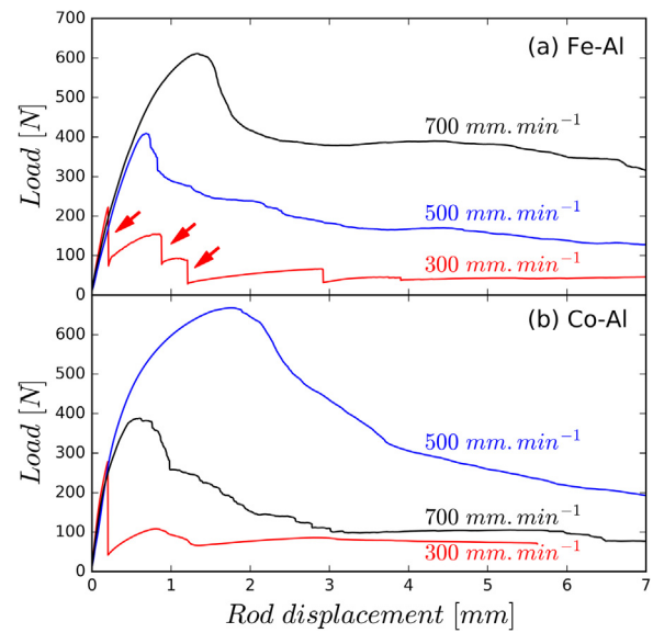
Fig. 7. Load-displacement curves of the pushing rod measured during the crack propagation tests for the (a) Fe-Al and (b) Co-Al systems. The red arrows denote a sudden brittle propagation of the crack at 300 mm min -1 in the Fe-Al system.
