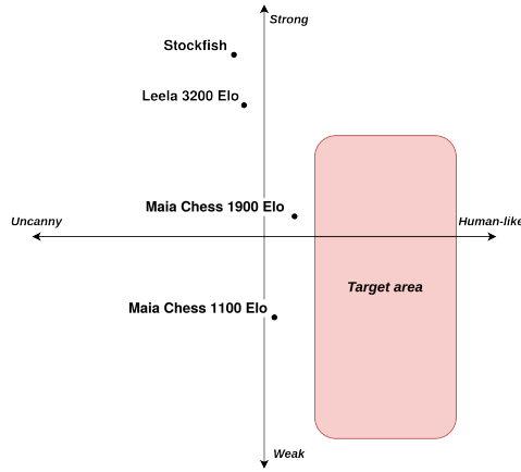
Figure 1.1: Some artificial agents for chess are plotted on this graph based on their performance in the move matching task [4]. The x-axis goes from 0% of human moves predicted (uncanny) to 100% (human player). The y-axis measures playing strength against the current top engine, Stockfish ( https://stockfishchess.org/ ), with a measured Elo of 3641 on the CCRL scale at the time of writing. Current approaches tend to predict human moves with around 50% chance, and the playing strength of an agent does not correlate to it being more or less human. Our aim is to target the red area , focusing on human-likeness rather than playing strength.
