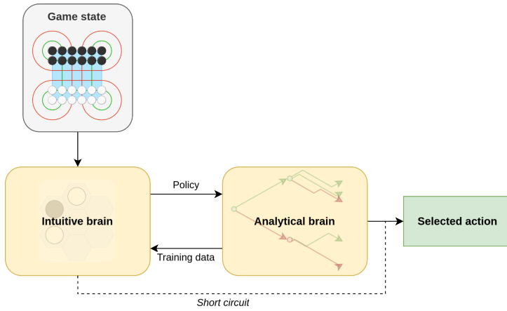
Figure 4.2: Co-dependency between the two systems of DPTC is illustrated as a back-and-forth, the intuitive brain guiding the analytical MCTS algorithm during its iterations by reducing the search space drastically, while the results of this deeper analysis are learnt from to sharpen the intuition of the model.
