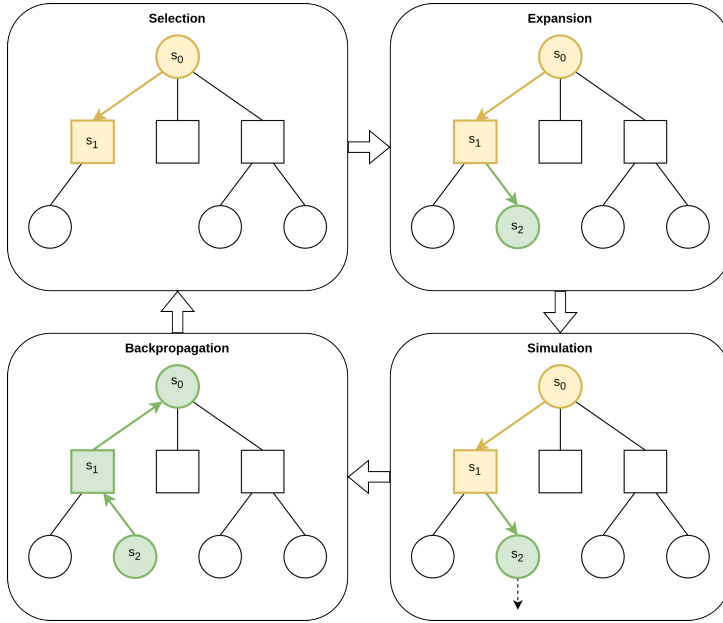
Figure 2.2: Graphical representation of one iteration of the MCTS algorithm. We first select a non-expanded node by going down the tree while balancing exploration and exploitation. The selected node is then expanded , leading to a sampling of possible results using playouts . The sampled result is then backpropagated to further direct future iterations of the algorithm.
