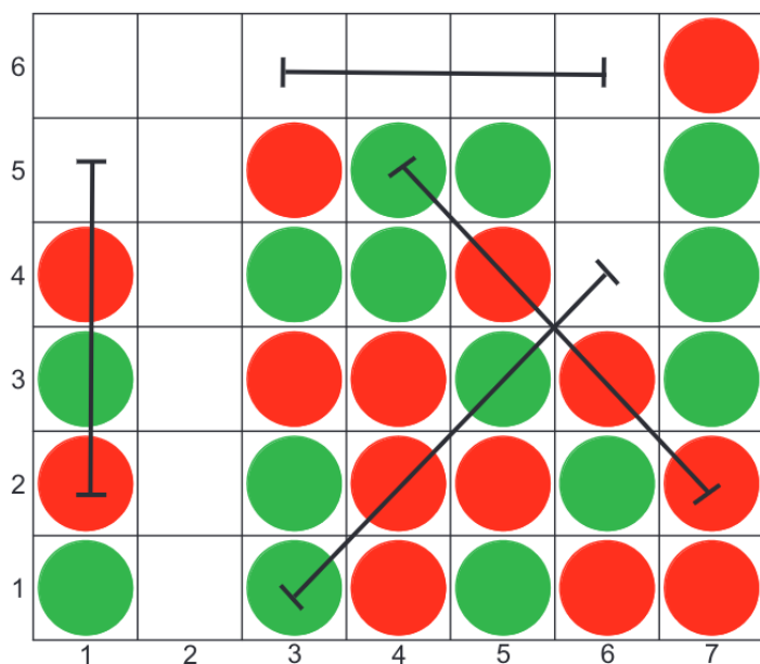
Figure 3.4: An example of the four possible contexts described by Mandziuk in his paper [23]. It matches lines of 4 pieces, in any direction, and for all cells.
