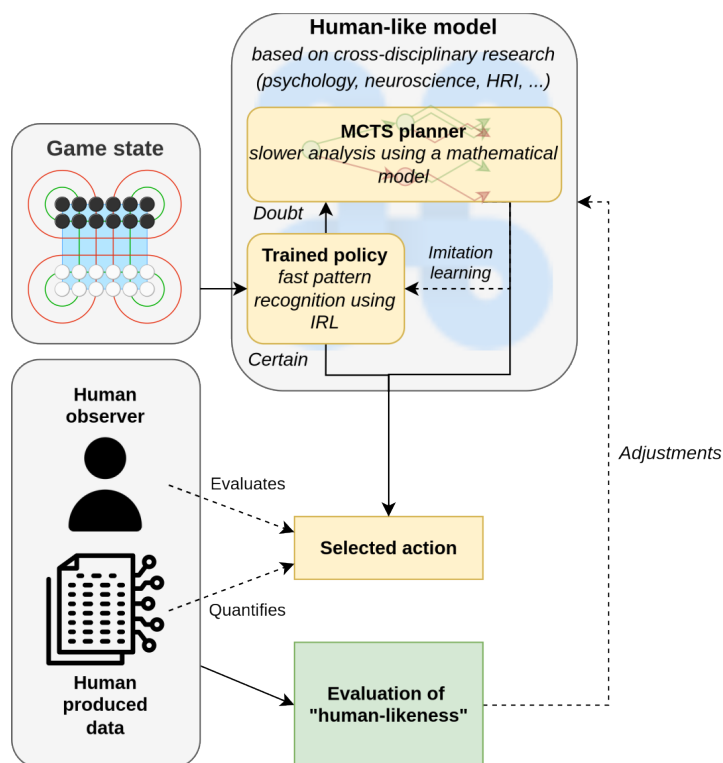
Figure 4.1: A preliminary experimental setup involving an AI model inspired by the dual-process theory of cognition [75]. This model integrates a rapid pattern recognition system developed through Inverse Reinforcement Learning (IRL) and based on state-action features (System 1) that defaults to a Monte Carlo Tree Search model (System 2) when it encounters states of uncertainty regarding the optimal action. The outputs of this model are assessed both qualitatively by humans through a Turing test and quantitatively by comparing them against statistical player profiles. This two-pronged evaluation method aims to gauge the model's "human-likeness" effectively, ensuring a robust measure of its performance in scenarios mimicking human decision-making.
