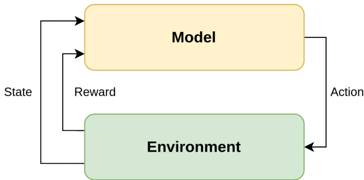
Figure 2.3: Visualization of the reinforcement learning framework. The agent and environment form a feedback loop where the agent modifies the environment through its actions, receiving a reward and updated observation (state) in exchange. The observed reward and state can then be used to train the agent so it maximizes the received reward in future interactions.
