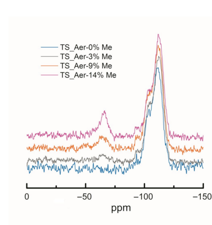
Figure 1. Solid-state 29 Si direct excitation MAS-NMR spectra of calcined TS_Aer-x%Me. Spectra are normalized to the Q 4 contribution and are vertically offset for clarity.
