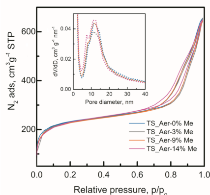
Figure 4. N 2 physisorption isotherms of TS-Aer x%Me catalysts. Pore size distributions (PSDs) based on the desorption branch of the isotherms are shown in inset.
