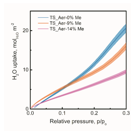
Figure 5. Vapor water adsorption isotherms normalized by the specific surface area ( SSA_{corrected} ) at low relative pressures. The normalized water uptake values are depicted on the curve and the shaded regions denote the estimated uncertainty of 5% due to the N_2 physisorption measurement of SSA_{corrected} .
