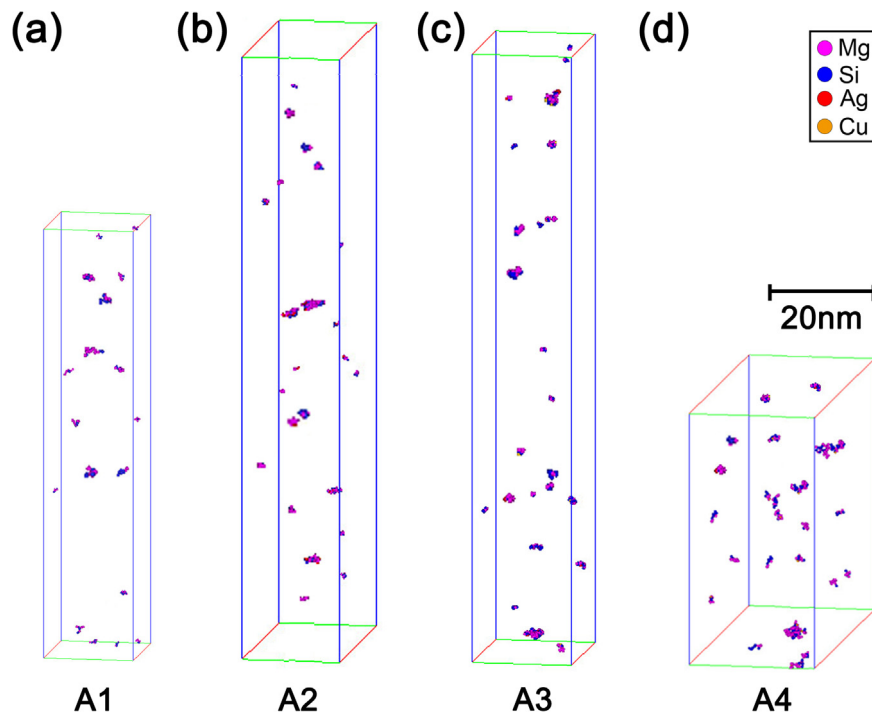
Fig. 2. Atoms maps for the four alloys after 2 weeks NA, (a) the A1 base alloy; (b) the Ag-added A2 alloy; (c) the Ag-Cu-added A3 alloy; (d) the Cu-added A4 alloy.
