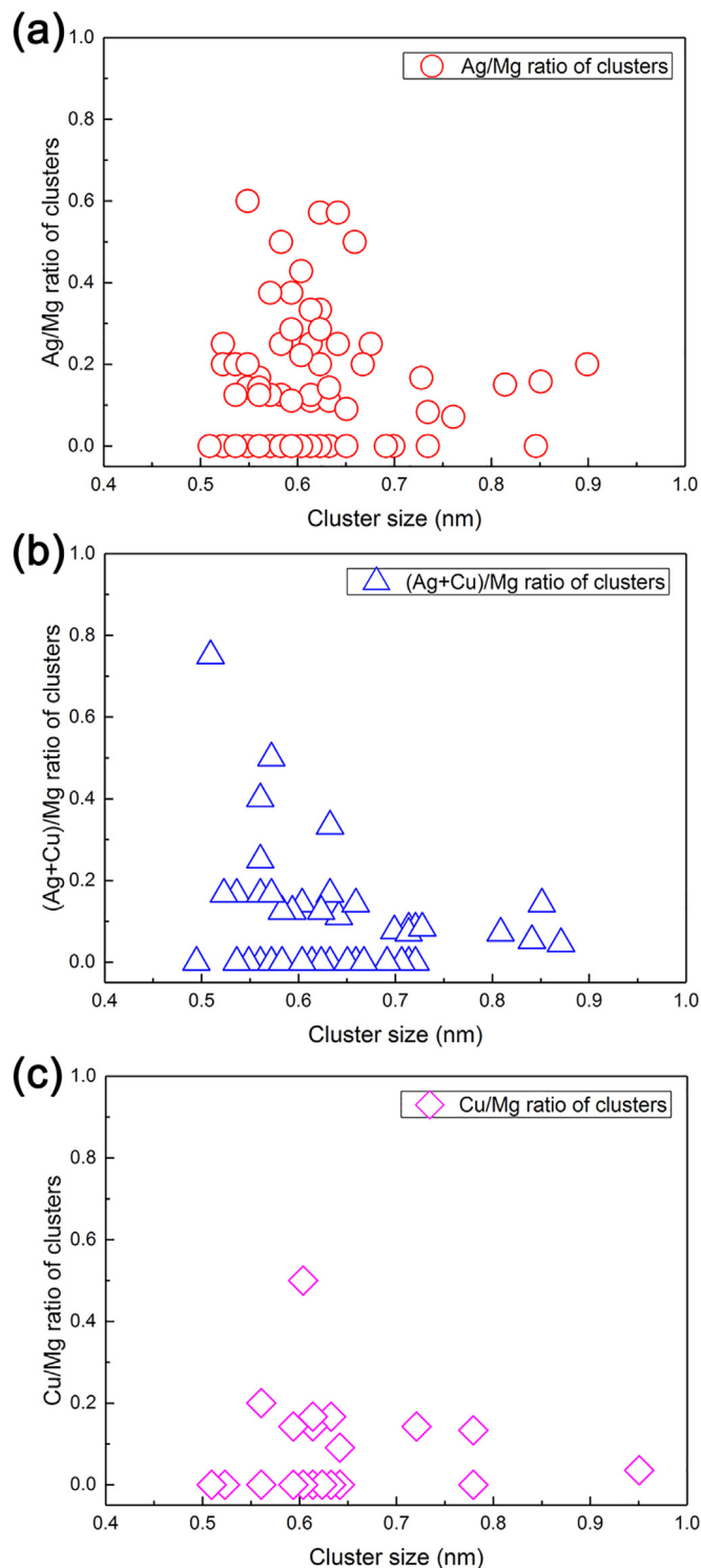
Fig. 5. Plots of the measured X/Mg ratio against cluster size after 2 weeks NA treatment for the three Ag/Cu-added alloys, (a) the Ag-added A2 alloy; (b) the Ag-Cu-added A3 alloy; (c) the Cu-added A4 alloy.
