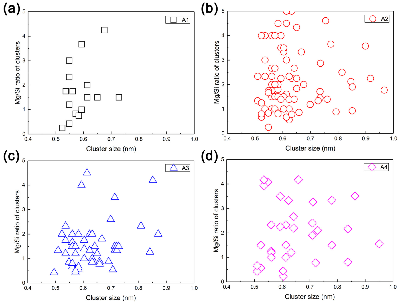
Fig. 4. Plots of the measured Mg/Si ratio of cluster against cluster size after 2 weeks NA for the four alloys, (a) the A1 base alloy; (b) the Ag-added A2 alloy; (c) the Ag-Cu-added A3 alloy; (d) the Cu-added A4 alloy.
