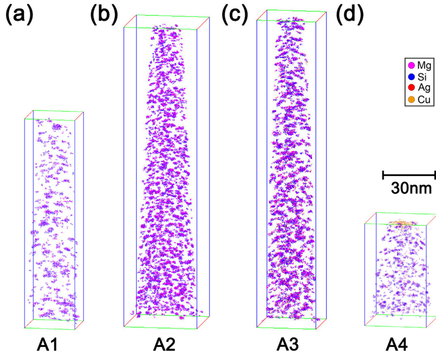
Fig. 6. (a) Atoms maps for the four alloys after AA at 443 K for 5 min, (a) the A1 base alloy; (b) the Ag-added A2 alloy; (c) the Ag-Cu-added A3 alloy; (d) the Cu-added A4 alloy.
