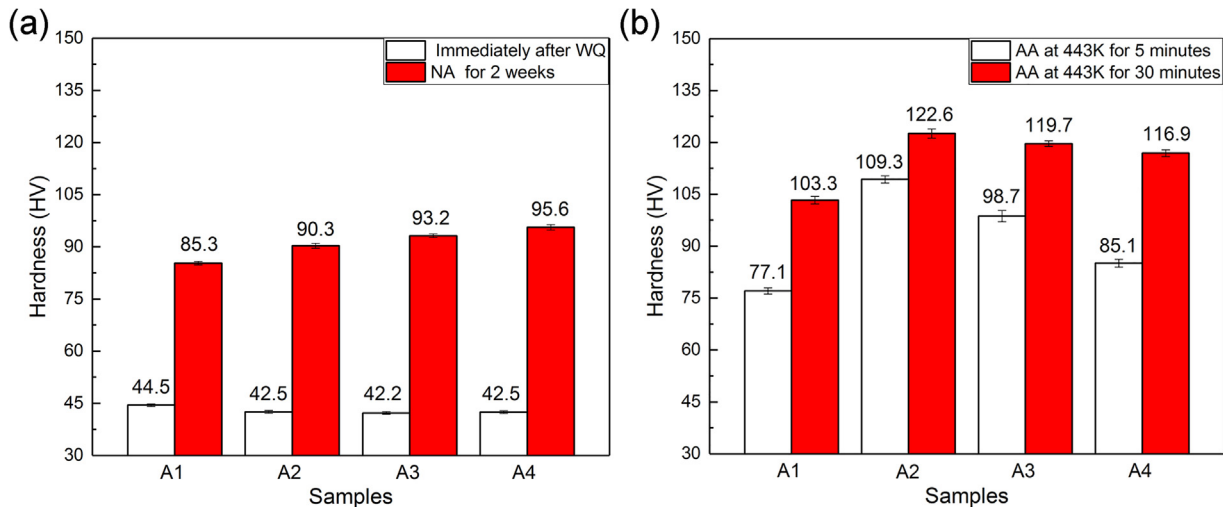
Fig. 1. Vickers hardness for the four alloys (a) immediately after WQ and 2 weeks NA, (b) AA at 443 K for 5 min and 30 min immediately after WQ.
