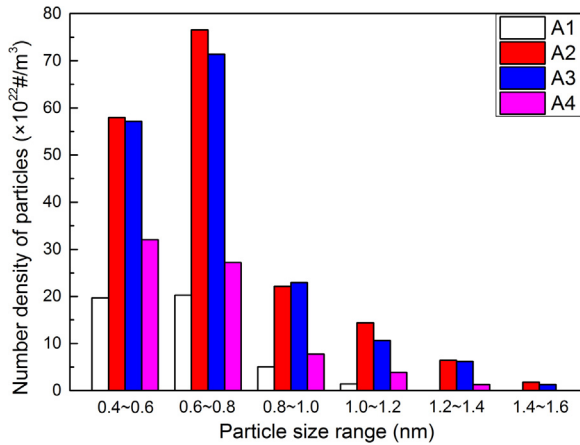
Fig. 7. Number density of particles as a function of the particle size for the four alloys after AA at 443 K for 5 min.
