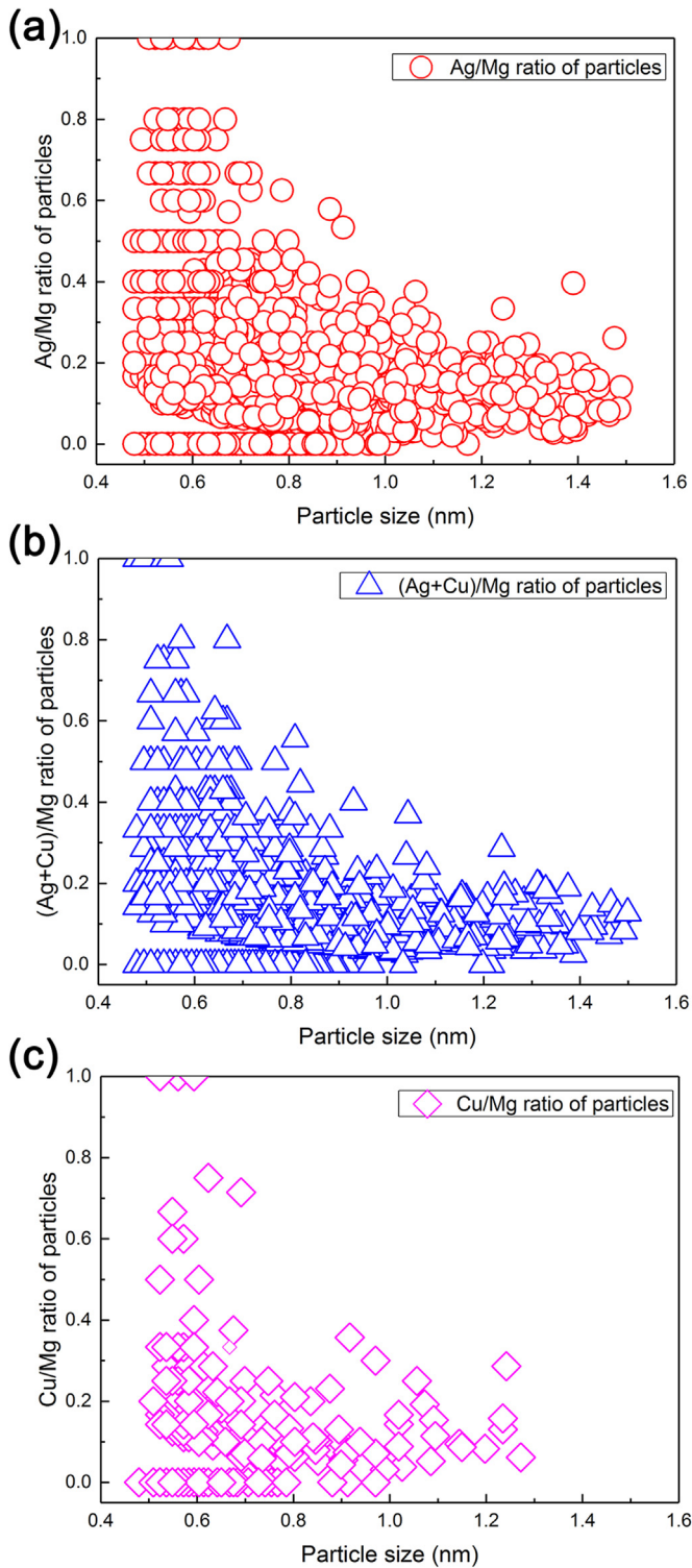
Fig. 9. Plots of the measured particle X/Mg ratio against particle size after 5 min AA treatment for the three Ag/Cu-added alloys, (a) the Ag-added A2 alloy; (b) the Ag-Cu-added A3 alloy; (c) the Cu-added A4 alloy.
