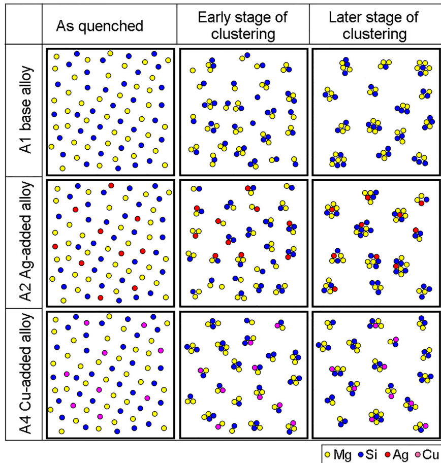
Fig. 10. The schematic illustrations of cluster evolution in the A1 base alloy, the Ag-added A2 alloy and the Cu-added A4 alloy during NA treatment.
