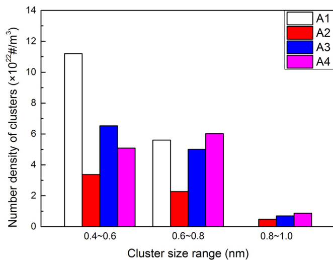
Fig. 3. Number density of clusters as a function of the cluster size for the four alloys after 2 weeks NA.
