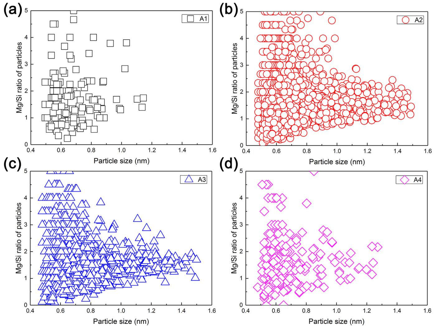
Fig. 8. Plots of the measured particle Mg/Si ratio against particle size after 5 min AA for the four alloys, (a) the A1 base alloy; (b) the Ag-added A2 alloy; (c) the Ag-Cu-added A3 alloy; (d) the Cu-added A4 alloy.
