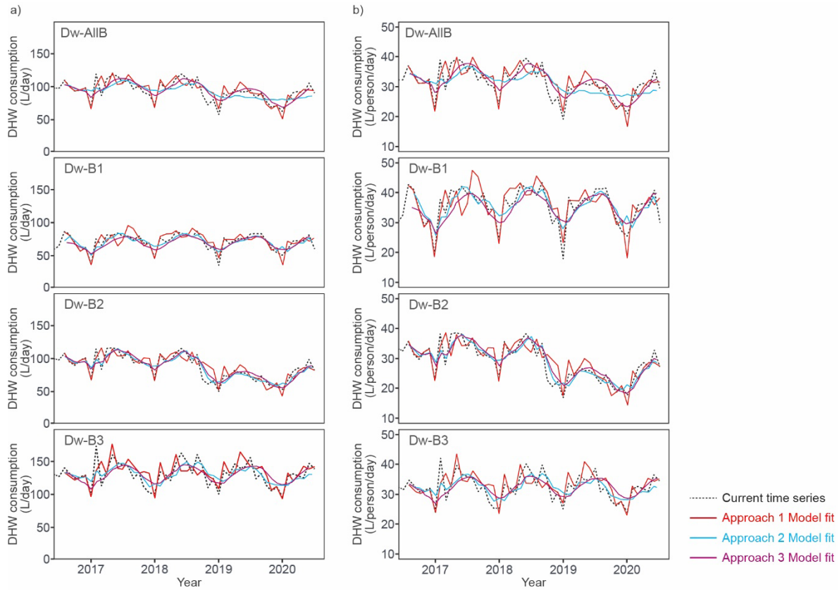
Figure 3. DHW estimation level in a) L/day and b) L/person/day, with the 3 approaches and different dwelling typologies
