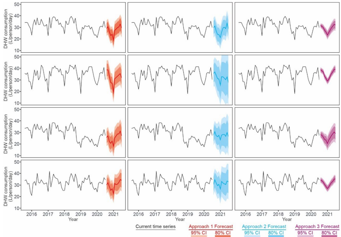
Figure 5. DHW prediction in L/person/day with the 3 approaches and different housing layouts.
