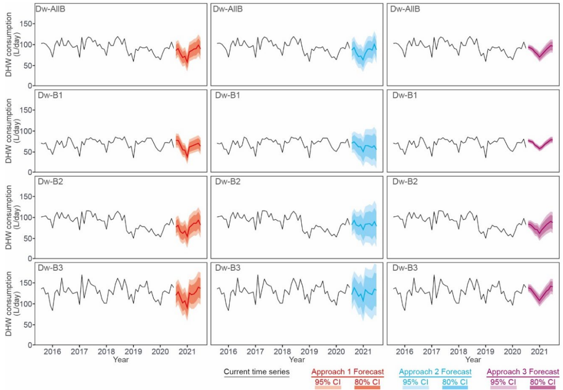
Figure 4. DHW prediction in L/day with the 3 approaches and different housing layouts.
