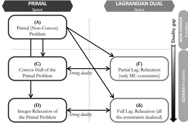
Fig. 1. Landscape of problems for computing / estimating convex hull prices.
