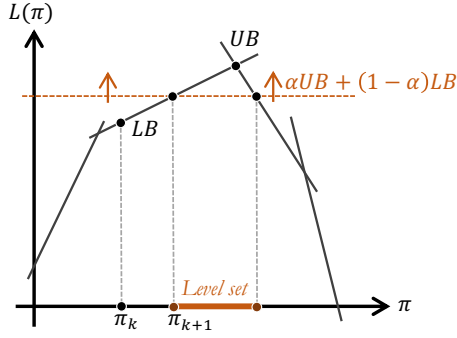
Fig. 2. Illustration of projection on the level set.
