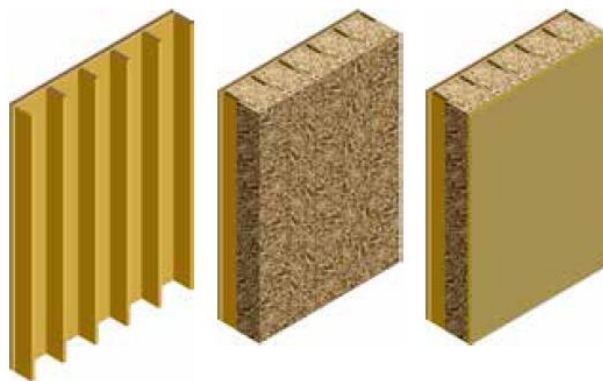
Fig 1: Straw-bale wall studied, prefabricated in Wallonia
