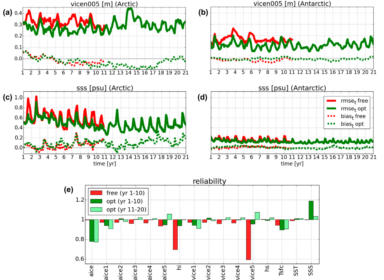
Fig. 12. Panels (a,b) and (c,d): \text{rmse}_t (bold lines) and \text{bias}_t (dotted lines) of vices and SSS for FREE (red, only first 10 years) and for the optimal setting (green, 20 years) in the Arctic and in the Antarctic, respectively. Panel (e) shows the summary of the global time and space averaged reliabilities of all considered variables for FREE (red), and the optimal setting (green), where the evaluation is splitted into decades.
