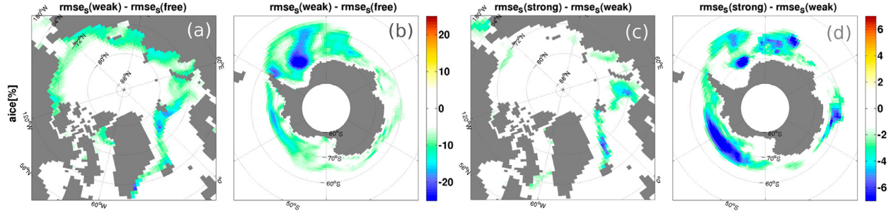
Fig. 5. Differences in rmse_s of aice between WEAK and FREE in the Arctic (a) and in the Antarctic (b) with maximum rmse_s of 35%, and between STRONG and WEAK in the Arctic (c) and in the Antarctic (d) with maximum rmse_s of 14%.
