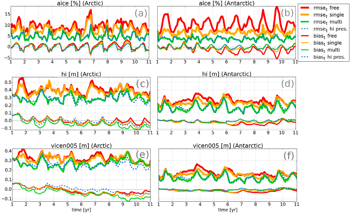
Fig. 2. \text{rmse}_t (bold lines) and \text{bias}_t (thin lines) of aice (a,b), hi (c,d) and \text{vices}_5 (e,f) in the Arctic (left column) and in the Antarctic (right column) for FREE (red), SINGLE (orange), MULTI (green) and HI_PRESERVE (blue).
