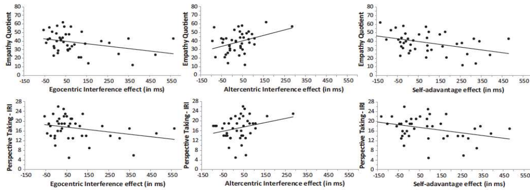
Fig. 3. Correlations between the self-reported measures of empathy and the individual scores in the belief task.
