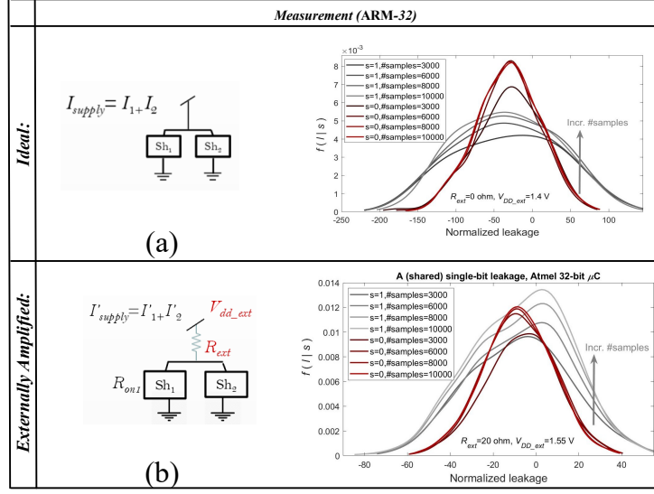
Figure 8: f(l|s) , 1 \cdot 10^6 traces: (a) R_{ext}=0\Omega (b) R_{ext}=20\Omega .
