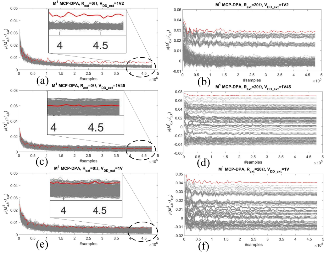
Figure 7: AES DoM Order 2. 1 st -order MCP-DPA correlation vs. the number of traces: V_{DD\_ext} = 1.2V (nominal): (a) R_{ext} = 0\Omega (b) R_{ext} = 20\Omega . V_{DD\_ext} = 1.45V : (c) R_{ext} = 0\Omega , (d) R_{ext} = 20\Omega . V_{DD\_ext} = 1V : (e) R_{ext} = 0\Omega , (f) R_{ext} = 20\Omega .
