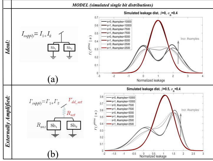
Figure 2: f(l^{simu.} | s) : (a) \beta=0 (b) \beta=0.5 .
