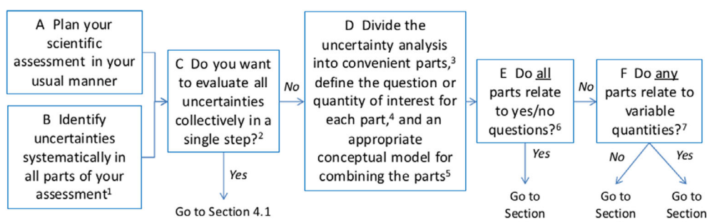
Figure 4: Deciding how to handle uncertainty in a case-specific assessment. Numbered superscripts refer to text notes following the figure in the original document (Guidance on Uncertainty Analysis in Scientific Assessments, EFSA Scientific Committee, 2018b). Letters (A,B, C, etc.) are to facilitate reference to specific steps in the figure. See original document for additional details
