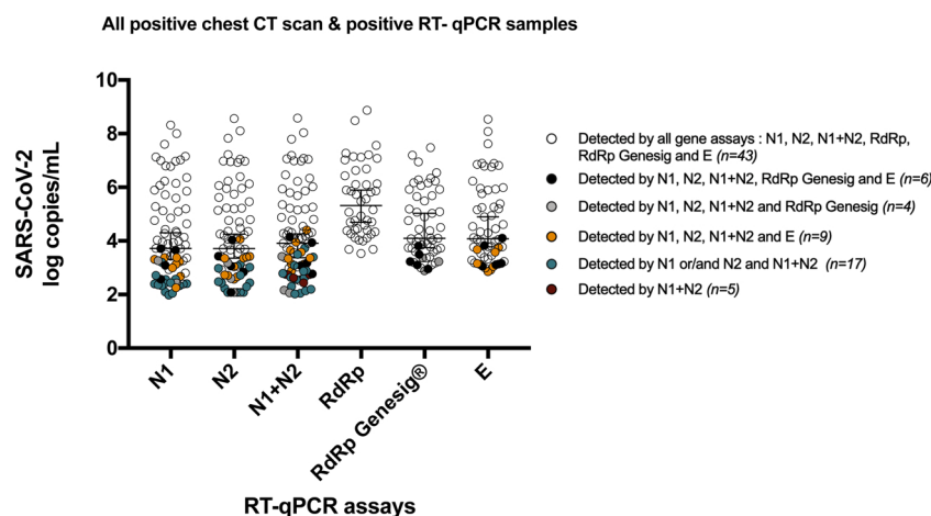
Fig. 2. Comparison of the viral load detected by the six RT-qPCR assays among the positive nasopharyngeal swabs (n = 84).
