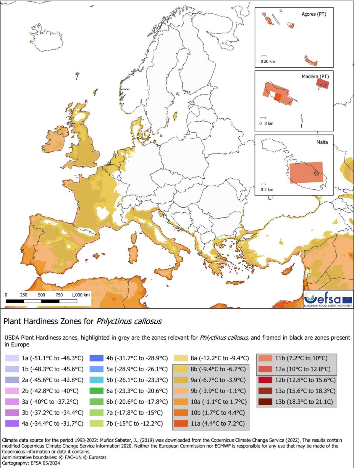
FIGURE D.3 Hardiness zone map based on the average annual minimum temperature for the period 1993–2022. The map highlights the hardiness zones (highlighted in grey in the legend) in the EU where the average minimum temperature is higher or equal to the minimum value sampled using Phlyctinus callosus occurrences. The Hardiness zone map is based on the recent implementation of the USDA Plant Hardiness Zones (2023).
