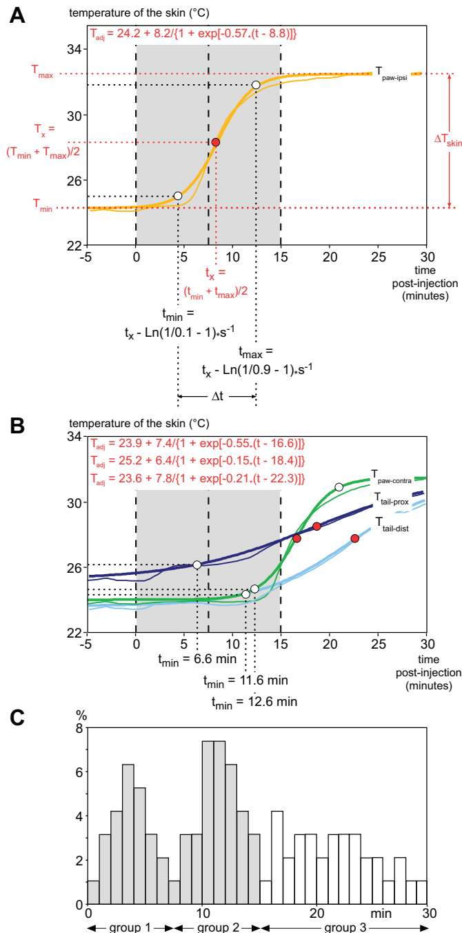
Fig. 1. Procedure to analyze the muscimol-induced variations of skin temperature. A and B , abscissa: time in minutes with reference to the end of the microinjection. Ordinate: temperature in ^\circ\text{C} . The grey area corresponds to the time intervals <7.5 and 7.5 – 15 min postinjection, delimited by vertical dotted lines. A : analysis of temperature variations observed from an ipsilateral hind paw ( T_{\text{paw-ipsi}} ). The thin yellow line is the temporal evolution of the temperature recorded during the 5-min control period and the following 30 min postinjection. The thick yellow line is the corresponding adjusted sigmoid Boltzmann curve T_{\text{adj}} = T_{\text{min}} + \Delta T_{\text{skin}} / \{1 + \exp[-(t - t_x)/s]\} , with R^2 = 0.99 (equation at top left). The adjusted parameters of the function are shown in red, namely the adjusted skin temperature during the control period ( T_{\text{min}} = 24.2^\circ\text{C} ), the adjusted maximal skin temperature at the end of the process ( T_{\text{max}} = 32.4^\circ\text{C} ), the amplitude of skin temperature variation ( \Delta T_{\text{skin}} = T_{\text{max}} - T_{\text{min}} = 8.2^\circ\text{C} ), and the inflection point ( t_x, T_x = T_{\text{min}} + \Delta T_{\text{skin}}/2 ) [(8.8 min, 28.3^\circ\text{C} )] of the sigmoid represented by a red point. The beginning ( t_{\text{min}} ) and end ( t_{\text{max}} ) of the ascending phase of vasodilatation were then calculated by considering the 10 and 90% percentiles of \Delta T_{\text{skin}} : t_{\text{min}} = t_x - \text{Ln}(1/0.1 - 1) \times s^{-1} = 4.9 \text{ min} and t_{\text{max}} = t_x - \text{Ln}(1/0.9 - 1) \times s^{-1} = 13.9 \text{ min} , represented by white points. B : calculation of the beginning of the ascending phase of vasodilatation observed from the corresponding three other recorded zones ( T_{\text{paw-contra}} , T_{\text{tail-prox}} , and T_{\text{tail-dist}} ). The thin and thick curves represent the genuine and adjusted curves, respectively. The green, dark blue, and light blue curves correspond to the contralateral hind paw, proximal and distal parts of the tail, respectively (corresponding equations provided at top left). Calculations of t_{\text{min}} were made as in A , except for the proximal part of the tail for which a 15% percentile was used in place of the 10% (see text). C : histogram showing the distribution of the beginning time of vasodilatation ( t_{\text{min}} ) for the ipsilateral hind paws, allowing the categorization into 3 groups: group 1 : t_{\text{min}} < 7.5 \text{ min} ; group 2 : 7.5 < t_{\text{min}} < 15 \text{ min} ; group 3 : t_{\text{min}} > 15 \text{ min} .
