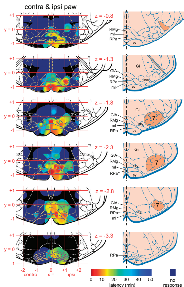
Fig. 5. Three-dimensional mapping of the hind paw response latencies t_{\text{min}} as a function of injection sites. The responses obtained from the left and right paw were merged by expressing the location of the injection site as ipsilateral (positive x -axis) vs. contralateral (negative x -axis) relative to the paw. Left : interpolated response latencies are indicated by the false colors (scale shown at bottom right). They are adjusted on frontal sections of the brain from interaural z = -0.8 (top) to z = -3.3 mm (bottom) with y being the ventrodorsal coordinate, again with reference to the interaural line. Right : drawings are based on the stereotaxic atlas by Paxinos and Watson (1986).
