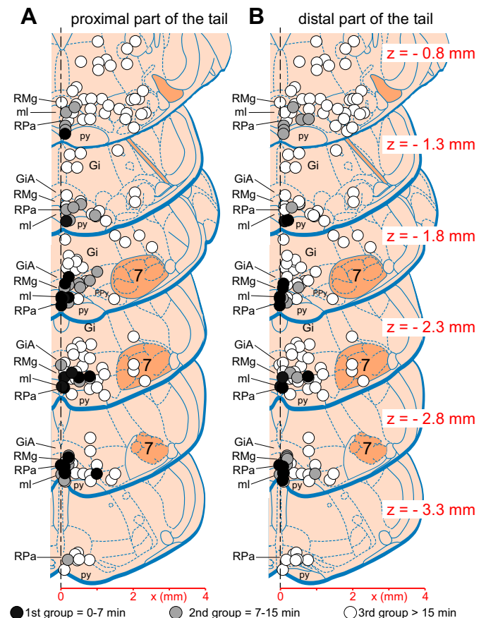
Fig. 7. Overall effects elicited by muscimol microinjection on the skin temperature recorded from the tail. A: proximal part of the tail. B: distal part of the tail. Symbols and abbreviations as in Fig. 4.
