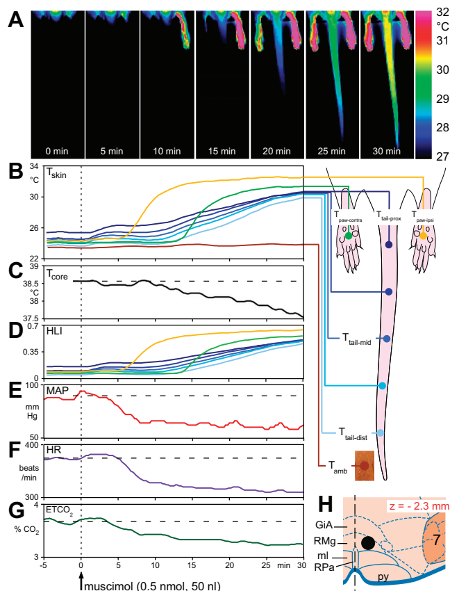
Fig. 2. Example of effects elicited by muscimol microinjection in the rostral ventromedial medulla (RVM). A : example of pictures taken at 0, 5, 10, 15, 20, 25, and 30 min postinjection of a thermographic movie recorded with a 320 \times 240 pixel resolution (see the corresponding Supplemental Video S1). The false color scale of temperature is shown at right . B : temporal evolution of the temperatures recorded during the 5-min control and 30 min postinjection periods. Abscissa: time in minutes. Ordinate: temperature in ^{\circ}\text{C} . The 8 analyzed zones (10 pixels each) are indicated on the drawing at right . T_{\text{paw-ipsi}} (yellow) and T_{\text{paw-contra}} (green) corresponds to the skin temperature of the ipsi- and contralateral hind paw, respectively. T_{\text{tail-prox}} (dark blue) and T_{\text{tail-dist}} (light blue) corresponds to the skin temperatures of the proximal and distal part of the tail, respectively; there are 3 additional intermediate blue sites between these 2 sites. T_{\text{amb}} (brown) corresponds to the ambient temperature measured from a small piece of wood. Note the stability of the control period in vasoconstriction with skin temperatures near T_{\text{amb}} . Following the microinjection, the ipsilateral hind paw skin temperature raised first, followed by the proximal and distal parts of the tail and at last the contralateral hind paw. C : temporal evolution of core temperature ( T_{\text{core}} ). Abscissa: time in minutes. Ordinate: temperature in ^{\circ}\text{C} . Note the decrease in T_{\text{core}} , starting shortly after the rise of T_{\text{paw-ipsi}} . D : corresponding heat loss index [ \text{HLI} = (T_{\text{skin}} - T_{\text{amb}})/(T_{\text{core}} - T_{\text{amb}}) ] (Romanovsky et al. 2002)] for the 7 skin areas considered. E : temporal evolution of mean arterial pressure (MAP). Abscissa: time in minutes. Ordinate: MAP in mmHg. Note the slight transitory increase in MAP shortly after the microinjection, followed by a sustained drop and then a progressive stabilization after 8 min postinjection. F : temporal evolution of heart rate (HR). Abscissa: time in minutes. Ordinate: HR in beat per minute (bpm). Note the slight transitory increase in HR shortly after the microinjection, followed by a sustained drop and then a progressive stabilization after 9 min postinjection. G : temporal evolution of \text{ETCO}_2 . Abscissa: time in minutes. Ordinate: end tidal \text{CO}_2 ( \text{ETCO}_2 ) in %. Note the parallel changes in E , F , and G . H : localization of the site of injection drawn on a frontal section of the brain in plane -2.3 mm caudal to the interaural line. The center of the injection site is located 0.3 mm lateral to the midline and 0.4 mm below the interaural line. 7, Facial nucleus; GiA, gigantocellular reticular nucleus pars alpha; ml, medial lemniscus; PPy, parapyramidal nucleus; py, pyramidal tract; RMg, raphe magnus nucleus; RPa, raphe pallidus nucleus.
