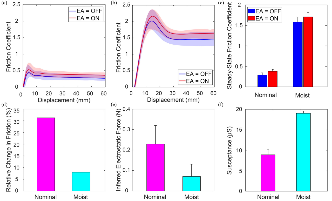
Fig. 3. Coefficient of friction (CoF) as a function of displacement with and without EA for (a) nominal and (b) moist finger conditions. The solid curves show the mean values and the shaded regions around them are the standard deviations for all trials. (c) Mean values of steady-state CoF under nominal and moist finger conditions with and without EA. (d) Relative difference in CoF between EA = ON and EA = OFF for the nominal and moist finger conditions. (e) Electrostatic forces inferred from the friction measurements for the nominal and moist finger conditions. (f) Mean values of the susceptance, an indicator of skin moisture, measured under the nominal and moist conditions.
