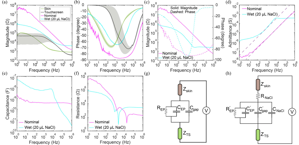
Fig. 4. The change in average electrical impedance (a) magnitude and (b) phase as a function of frequency for finger skin (green), the touchscreen itself (black), sliding finger on the touchscreen under the nominal (magenta) and wet (cyan) conditions. (c) The magnitude (solid curves) and phase (dashed curves) of the remaining impedance as a function of frequency for the sliding finger under the nominal (magenta) and wet (cyan) conditions as a function of frequency. (d) The change in the remaining admittance as a function of frequency for the sliding finger under the nominal (magenta) and wet (cyan) conditions. The dashed purple-colored lines are the one-decade-per-decade lines fitted to the admittance curves. The change in the (e) capacitance and (f) resistance at the interface between the finger skin and touchscreen under the nominal and wet conditions as a function of frequency. Our proposed circuit model for the finger in contact with a voltage-induced touchscreen under the (g) nominal and (h) wet conditions.
