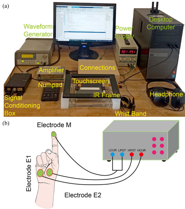
Fig. 1. (a) The setup used in our tactile perception experiments. (b) Schematic representation of skin moisture level assessment.
