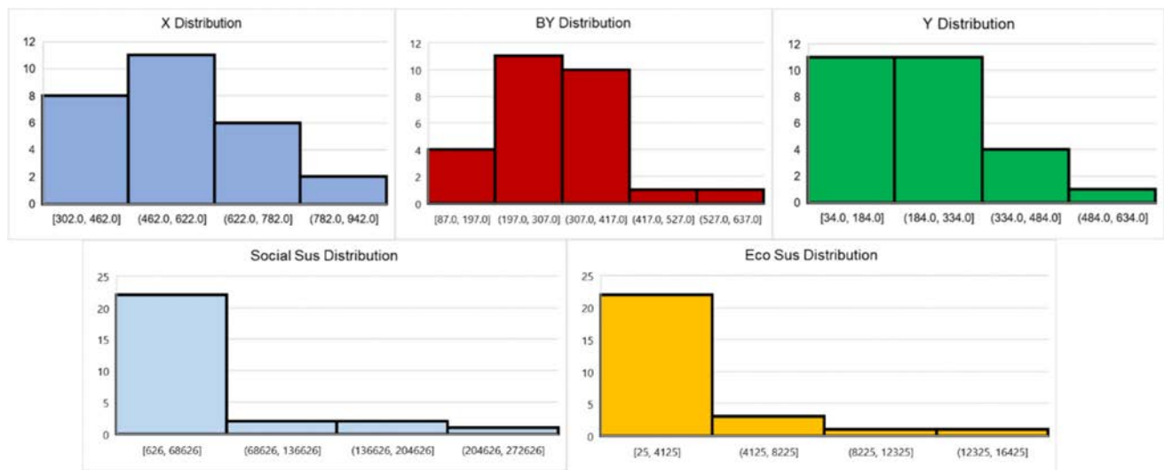
Fig. 1 Distributions of inputs, outputs and sustainability indicators. From top left: distribution of waste generated ( X ), distribution of waste sent to landfill and incinerated ( BY ), distribution of waste to be
