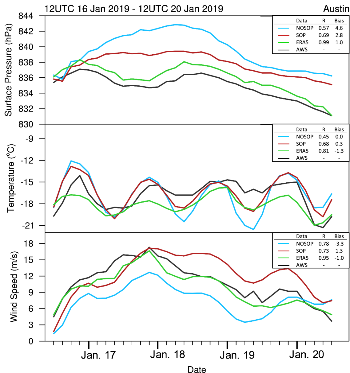
Figure 10. Time series of surface pressure (hPa, top panel), 2-m temperature ( ^{\circ}\text{C} , middle panel), and 10-m wind speed ( \text{ms}^{-1} , bottom panel) for the Austin AWS site in West Antarctica from no-SOP run (blue), SOP run (red), ERA5 global reanalysis (green), and AWS observations (black). Location of Austin marked in Figure 8. Period shown is 12 UTC 16–20 January 2019, with model values taken from forecasts initialized at 00 UTC 16 January. Panel insets show correlation coefficients and average bias error ( ^{\circ}\text{C} ) for the period for each data source.
