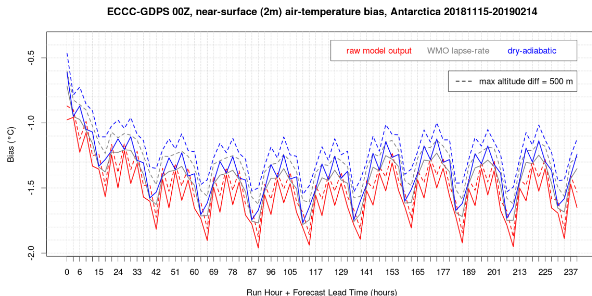
Figure 6. The Canadian Global Model (ECCC-GDPS) surface air temperature bias evaluated for the raw model output (red lines), and for the model output adjusted to the station elevation by applying the standard-atmosphere WMO-recommended lapse rate (0.0065 K/m, gray lines), and the dry adiabatic lapse rate (0.0098K/m, blue lines). The dashed lines show the bias calculated excluding stations which differ in elevation more than 500m from the model-tile altitude.
