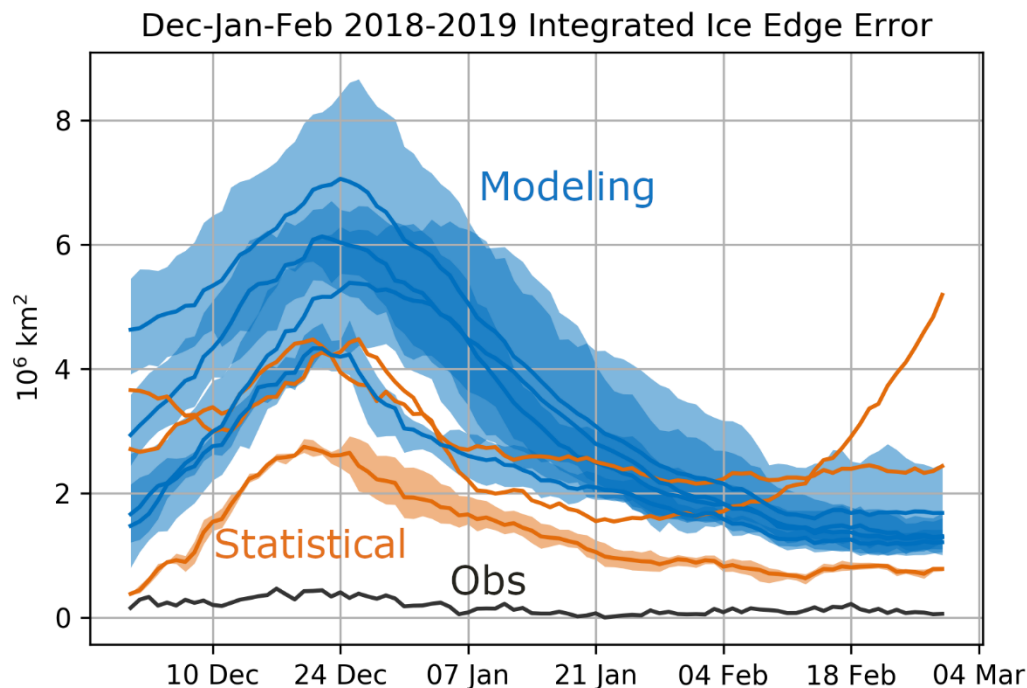
Figure 12. Integrated Ice Edge Error (IEEE; Goessling et al., 2016), a measure of spatial agreement of forecasted and observed sea-ice concentration, for dynamical model (blue) and statistical (orange) contributions participating in the austral summer 2018-2019 SIPN South coordinated forecast. The common reference verification product is NSIDC-0081 ( https://nsidc.org/data/nsidc-0081 ). Low values indicate high skill, the shadings (when available) indicate the ensemble range for a given forecasting system. The black line is the IEEE for an alternative observation product and is meant to represent uncertainty in the verification product itself.
