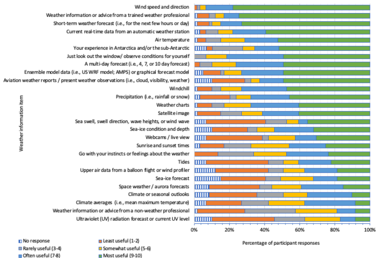
948 Figure 14. Usefulness of weather information items during deployment to the Antarctic and/or 949 sub-Antarctic. Percent of participant responses to the question: “On a scale from 1 (not at all 950 useful) to 10 (most useful), please assess how useful you find each of the following items when 951 you are in the Antarctic and/or sub-Antarctic.”
