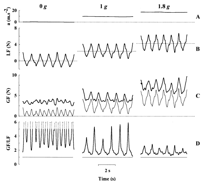
Fig. 2A–D Records of six contiguous cycles obtained during the stable period in each gravitational phase of the last trial of a non-experienced subject (NES). A The gravity level, B the load force (LF), C the grip force (GF, thick line ) and the slip force ( thin line ), and D the GF/LF ratio ( thick line ) and the slip ratio ( thin line ). The difference between the GF/LF ratio and the slip ratio reflects the safety margin. The friction coefficient was 0.5
