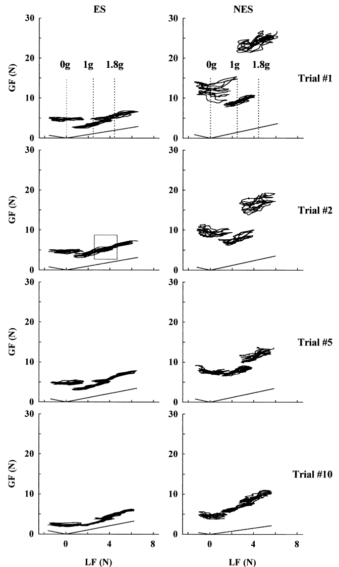
Fig. 3 The grip force (GF)–load force (LF) relationship measured during six arm cycles under three gravity levels during the first, second, fifth and tenth trials in an experienced subject (ES, left column ) and a non-experienced subject (NES, right column ). The dotted lines in the upper panels represent the object weight in each gravitational level. The slip force is presented by a straight line according to the friction coefficient of each trace. The inset in the left column shows the overlap between the load force ranges observed at 1 g and at 1.8 g. Trial 1 of the NES and the ES corresponded to the first and the fifteenth parabolic maneuvers of the aircraft, respectively
