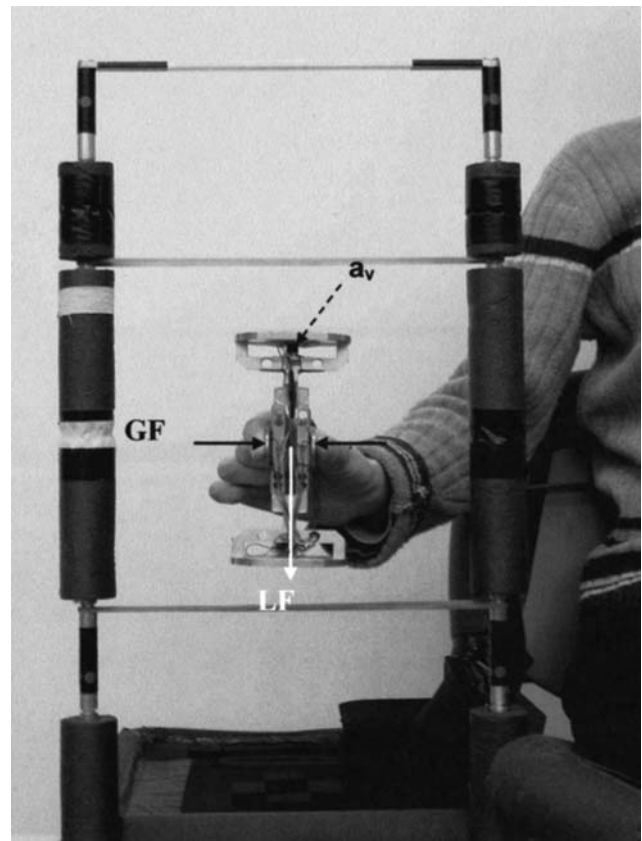
Fig. 1 Frontal view of the experimental setup. The subject moved the manipulandum up and down between the two elastic bands 20 cm apart. The grip force (GF, black arrows ) was measured by strain gauges, the load force (LF, white arrow ) was calculated from the vertical object acceleration measured by an accelerometer ( a_v , dashed arrow )
