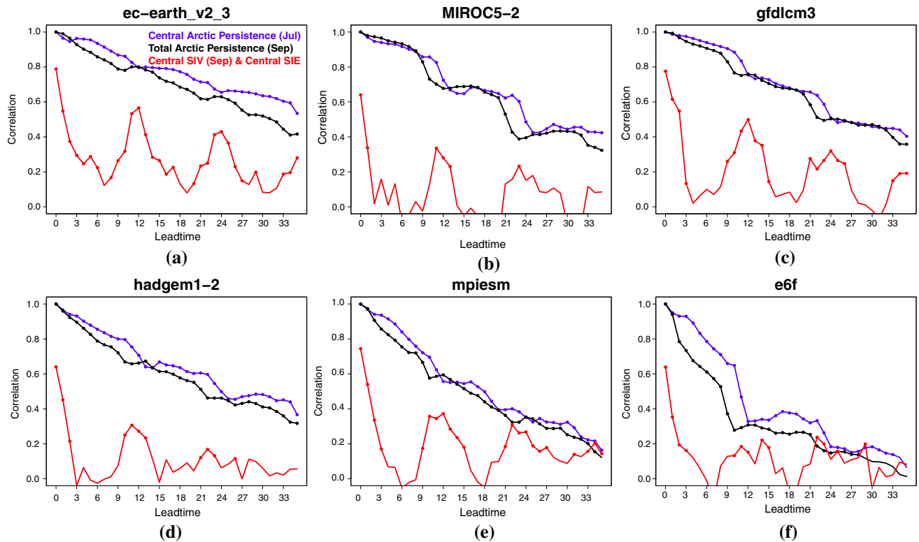
Fig. 3 In blue, the July central Arctic SIV autocorrelation. In black, the September ControlRun lagged autocorrelation for the pan-Arctic SIV. In red, the lagged correlation between the September central
