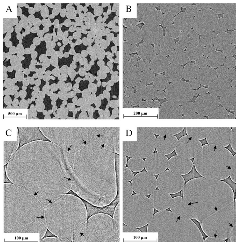
Figure 1. A to D, Tomographic images of the cortex of apple (A and C) and pear (B and D). Shown are slices ( 512 \times 512 pixels) obtained by absorption tomography (A and B), at 5- and 1.4- \mu\text{m} pixel resolution for apple and pear, respectively, and phase contrast tomography (C and D) at 700-nm pixel size. Dark regions are gas-filled intercellular spaces; light regions are cells. Cell walls (indicated by arrows) between adjacent cells can be distinguished in the phase contrast images and are specifically clear in apple cortex.
