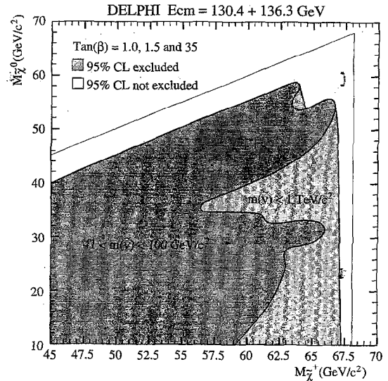
Fig. 5. Regions excluded at the 95% C.L. in the (m_{\tilde{\chi}_1^\pm}, m_{\tilde{\chi}_1^0}) plane. Three different values of \tan \beta have been used: 1, 1.5 and 35. The regions excluded when the sneutrino is light ( 41 \text{ GeV}/c^2 < m_{\tilde{\nu}} < 100 \text{ GeV}/c^2 ) are shown in dark grey; the additional regions excluded when the sneutrino is very heavy ( m_{\tilde{\nu}} = 1 \text{ TeV}/c^2 ) are shown in light grey. The outermost line corresponds to the kinematic limit.
