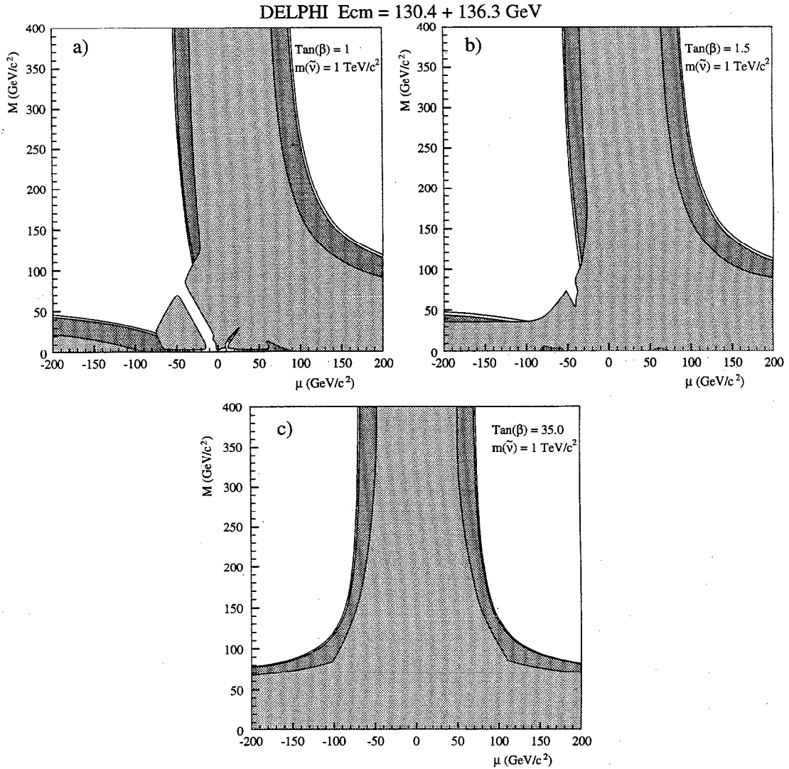
Fig. 6. Regions excluded at the 95% C.L. in the (M, \mu) plane are shown in dark grey for a) \tan \beta = 1.0 , b) \tan \beta = 1.5 and c) \tan \beta = 35 . The regions in light grey inside the curve had already been excluded at LEP1 by chargino or by neutralino searches [14]. The outermost line corresponds to the kinematic limit.
