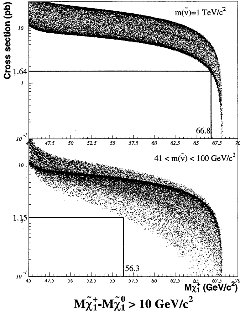
Fig. 3. Scatter plot of the expected cross-section at 136.3 GeV versus the chargino mass in the non-degenerate scenario ( \Delta M > 10 \text{ GeV}/c^2 ). The MSSM parameters M and \mu have been varied in the ranges 0 < M < 800 \text{ GeV}/c^2 and -400 \text{ GeV}/c^2 < \mu < 400 \text{ GeV}/c^2 for three different values of \tan \beta : 1, 1.5 and 35. A very heavy sneutrino ( m_{\tilde{\nu}} = 1 \text{ TeV}/c^2 ) has been assumed in the upper part and a light sneutrino ( 41 \text{ GeV}/c^2 < m_{\tilde{\nu}} < 100 \text{ GeV}/c^2 ) in the lower one.
