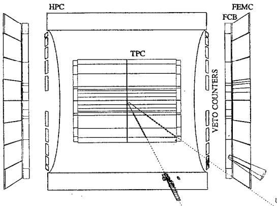
Fig. 2. Representation of the event remaining in the data after cuts. The TPC, the two crowns of the 40^\circ taggers, the FCB chambers and the FEMC calorimeter are shown. The high energy deposit of the 11.7 GeV/c particle in the barrel electromagnetic calorimeter, together with the signal of the 7.7 GeV/c particle in the 40^\circ taggers, its small energy deposit in the hadronic calorimeter and its effect in the FCB are visible.
