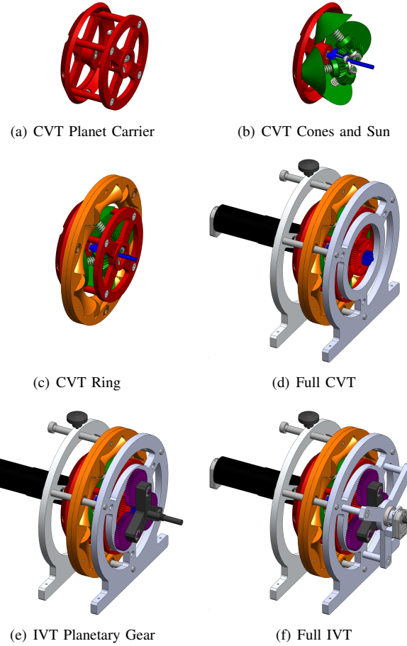
Fig. 8. Sequential assembly of the IVT CAD, highlighting the different components.
