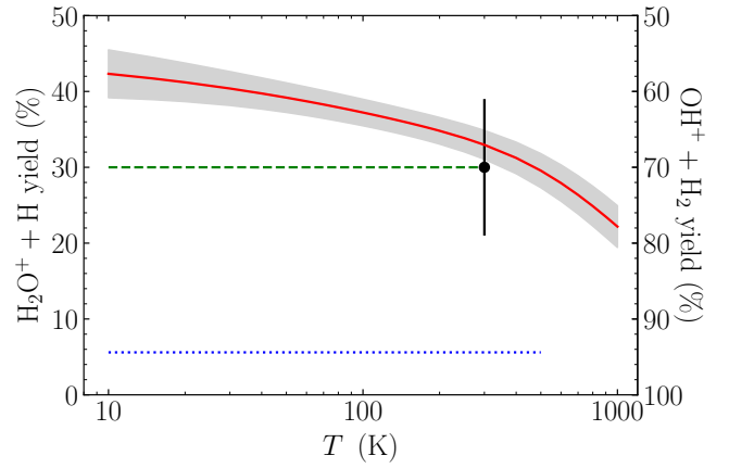
Figure 2. Branching ratio expressed as relative yield for the two product channels. Shown are: our results by the red solid line, with the gray area indicating the total experimental uncertainty at one standard deviation; the results of Milligan & McEwan (2000) by the circular data point; the results of Bettens et al. (1999) by the blue dotted line; and the ratio implemented in the astrochemical models listed in Sec. 3.2 by the green dashed line.
