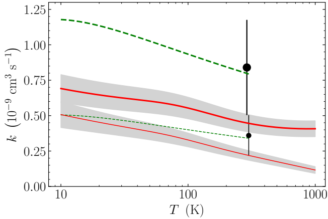
Figure 1. Thermal rate coefficient for the \text{OH}^+ + \text{H}_2 channel (upper bold data) and the \text{H}_2\text{O}^+ + \text{H} channel (lower fine data). Shown are: our results by the red solid lines, with the gray area indicating the total experimental uncertainty at one standard deviation; the results of Milligan & McEwan (2000) by the circular data points (shifted slightly in temperature for clarity); and the data implemented in the astrochemical models listed in Sec. 3.2 by the green dashed lines.
